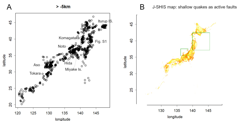
Figure 6. A. Epicentres shallower than 5 km (data from October 2025 to January 2026). Shallow events are concentrated where volcanic activity has been reported; the offshore clusters shown in Figure S1 are also visible because they occurred during the same interval. A shallow band immediately south of these features follows the Pacific coastline and corresponds to the shallow seismicity highlighted in Figure S1. The line extending from the Noto Peninsula to Sado Island lies on the Eurasian Plate and is subject to compressive loading; under the present filtering this segment appears unusually dominated by very shallow earthquakes. B. J-SIS Japan Seismic Hazard Information: shallow earthquakes and active faults [19], shown at the same scale as panel A. Inset (green outlines). Left outline: area shown in Figure 3; right outline: approximate extent of Figure S1.
