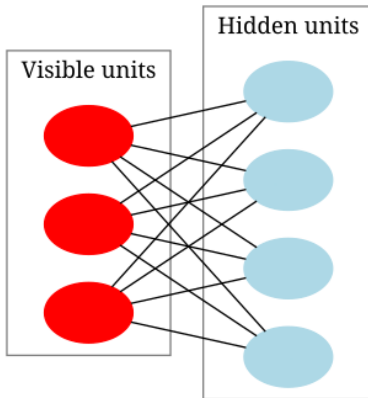
Figure 16.1. Diagram of a restricted Boltzmann machine
