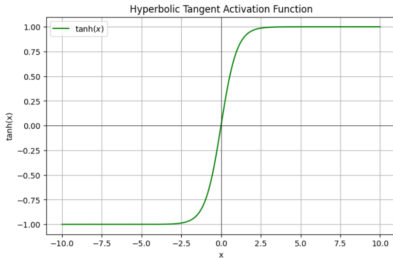
Figure 2.2. Hyperbolic Tangent Activation Function: \sigma(x) = \frac{e^x - e^{-x}}{e^x + e^{-x}}
