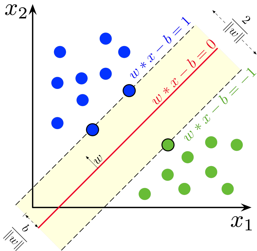
Figure 16.6. Illustration of the Support Vector Machine
