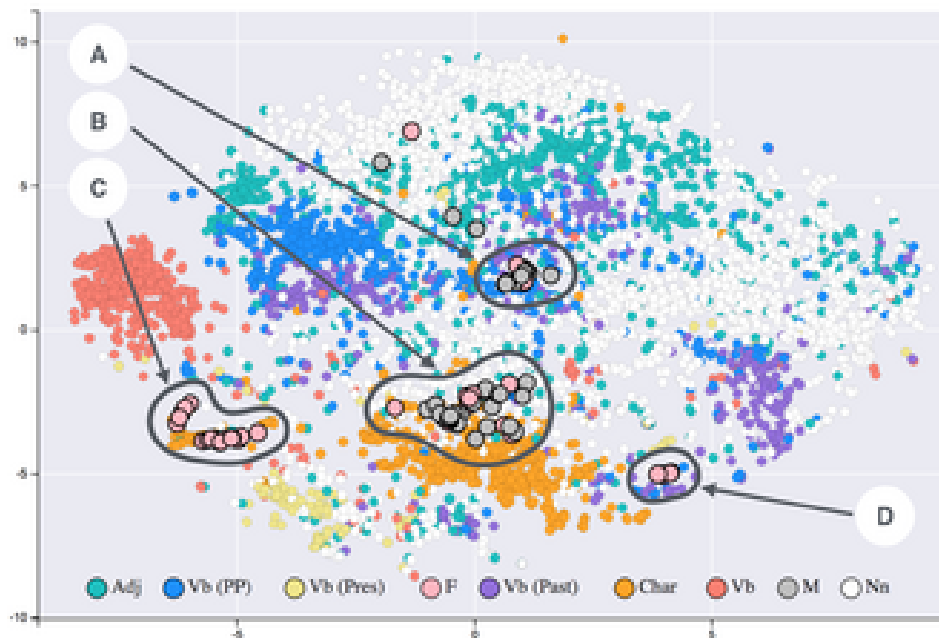
Figure 16.3. T-SNE representation of word embeddings derived from 19th-century literary texts
