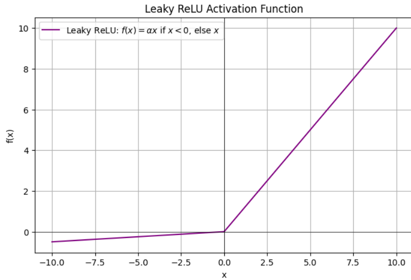
Figure 2.4. Leaky ReLU Activation Function
