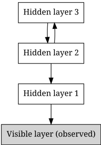
Figure 16.2. Diagram of a Deep belief network
