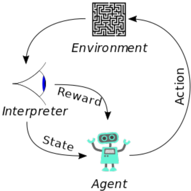
Figure 16.18. Framework of the Reinforcement Learning
