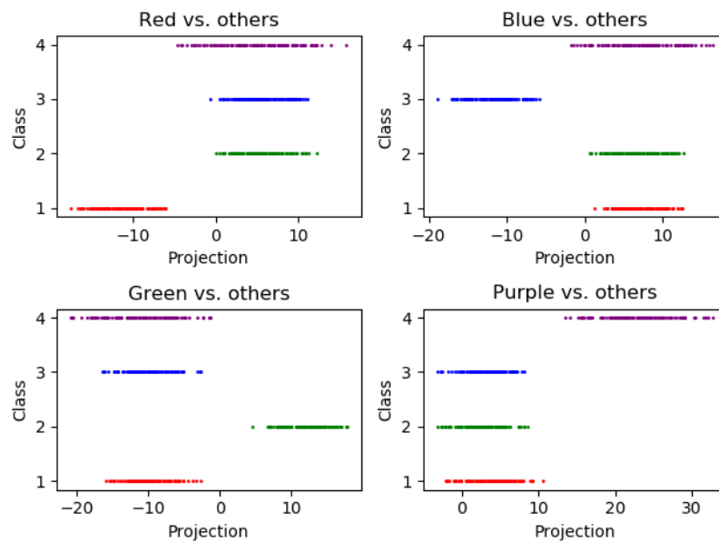
Figure 16.13. Projections along linear discriminant axes for 4 classes
