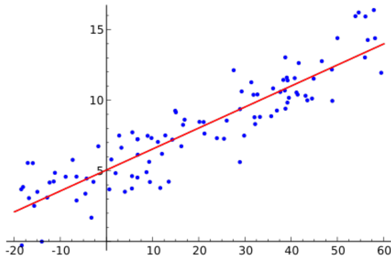
Figure 16.8. Simple Linear Regression
