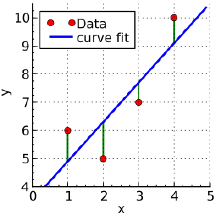
Figure 16.7. Framework of the Linear Regression
