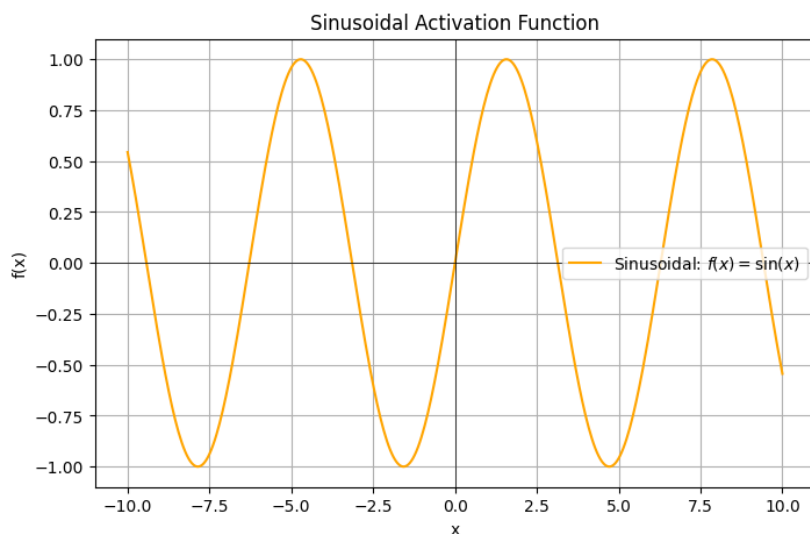
Figure 2.5. Sinusoidal Activation Function \sigma(x) = \sin(x)
