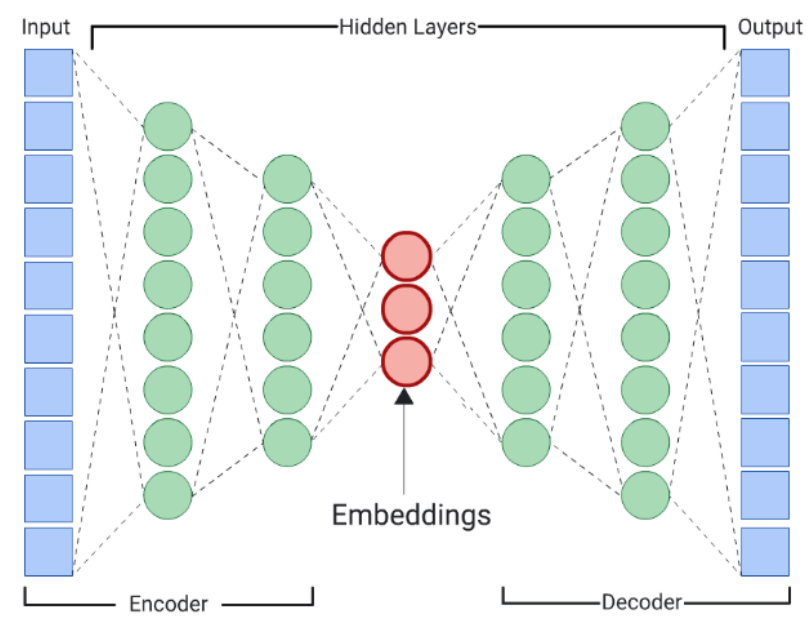
Figure 16.16. Autoencoder architecture
