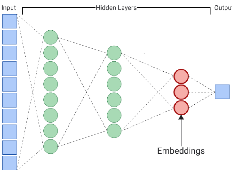
Figure 16.17. Predictor architecture
