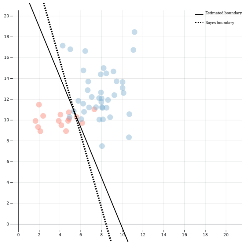
Figure 16.11. Linear discriminant analysis on a two dimensional space with two classes
