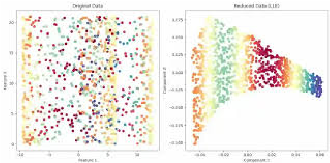
Figure 16.5. Data Reduction in Locally Linear Embedding Image Credit: Locally Linear Embedding in machine learning, geeksforgEEKS.org , https://www.geeksforgEEKS.org/locally-linear-embedding-in-machine-learning/
