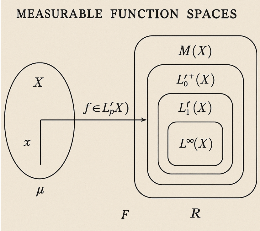
Figure 1.1. Measurable Function Spaces
