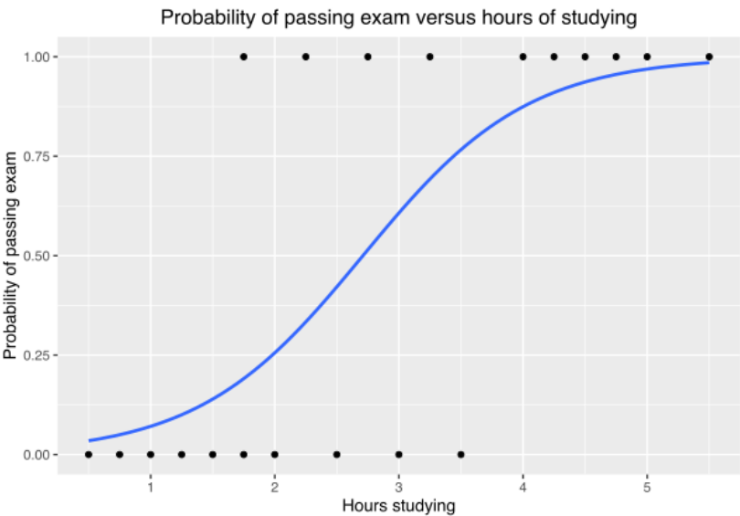
Figure 16.10. Example of a logistic regression curve fitted to data
