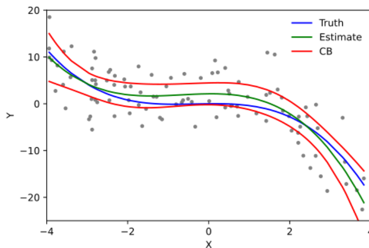
Figure 16.9. Cubic Polynomial Regression
