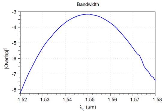
Figure 25. Overlap with the SMF-28 optical fiber TE_{00} mode at the diffracted field monitor, obtained for different wavelengths. The |\text{Overlap}|^2 is given in logarithmic scale, decibel (dB), wavelength in vacuum ( \lambda_0 ) is represented in linear scale.
