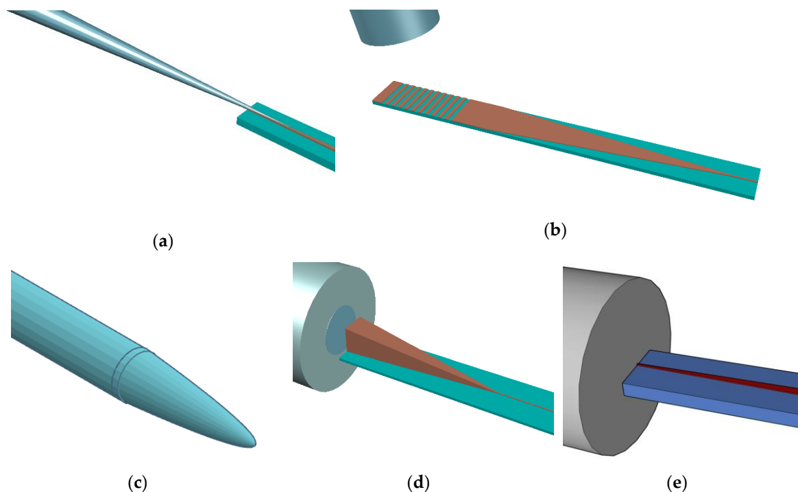
Figure 4. Photonic waveguide light coupling techniques: (a) Adiabatic coupler, consisting of tapered optical fiber termination and waveguide taper; (b) Non-apodized grating coupler, including optical fiber (with only the core and reduced cladding diameter represented), grating and waveguide taper; (c) tapered lensed optical fiber termination; (d) Spot size converter based on 3D taper (optical fiber coating not represented, cladding diameter reduced). (e) Spot size converter based on inverted taper (only the fiber core is represented). Representations not up to scale and not depicting functional devices, designed for demonstration purposes only.
