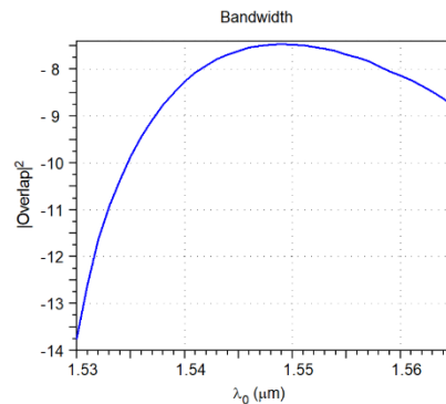
Figure 31. Overlap with the SMF-28 optical fiber TE 00 mode at the diffracted field monitor, obtained for different wavelengths. The |\text{Overlap}|^2 is given in logarithmic scale, decibel (dB), wavelength in vacuum ( \lambda_0 ) is represented in linear scale.
