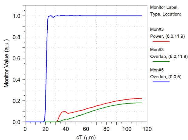
Figure 30. Efficiency test, from top to bottom, the blue line represents the overlap value (with the quasi-TE 00 waveguide's mode) measured at 1 \mu\text{m} before the waveguide's end (diffraction grating beginning). The red and green lines, represent the power and overlap (with the TE 00 mode of a simulated SMF-28 optical fiber) of the diffraction field, respectively, measured at a monitor whose center is at a distance of 6 \mu\text{m} from the grating.
