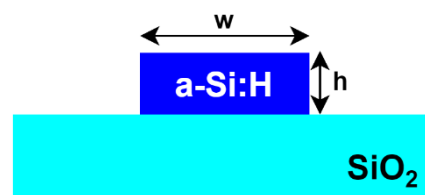
Figure 2. Transversal cut of the proposed strip waveguide, background is air, a 220 nm hydrogenated amorphous silicon (a-Si:H) layer (represented in blue) is deposited over silica (represented in light blue). The \text{SiO}_2 is much thicker (by at least one order of magnitude) than the amorphous silicon layer (figure not up to scale). The waveguide's height (thickness) is h , and the width is w , respectively. Since we are assuming a 2D model the influence of width was not studied.
