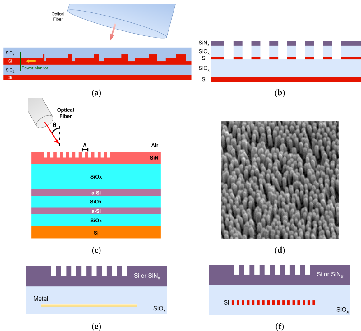
Figure 5. Some of the techniques employed to improve grating coupler efficiency and/or bandwidth. (a) Dual-level grating coupler [43]; (b) Grating coupler featuring stacked layers ( \text{SiN}_x on SOI) [53]; (c) Silicon nitride grating coupler featuring a DBR stack composed of two layers of amorphous silicon (a-Si) [60]; (d) Example of metamaterial (bare gold nanorod), image obtained by scanning electron microscopy (SEM) [64] – originally published by Optica Publishing Group, republished under the terms of the Creative Commons Attribution 4.0 License; (e) Grating coupler featuring a bottom metal reflector layer [61,62]; (f) Grating coupler with silicon bottom grating reflector [56].
