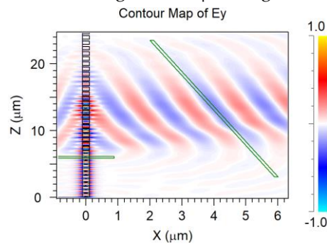
Figure 23. Representation on the XZ plane of the diffracted electric field, the green (transparent filled) horizontal bar is the waveguide's monitor and the slanted green (transparent filled) slanted bar is the diffracted field monitor. Image obtained from 2D-FDTD.
