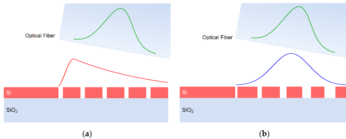
Figure 7. Hypothetical diffracted field intensity distribution of (a) non-apodized and (b) apodized grating couplers, both figures display a theoretical fiber model with a gaussian field distribution. The figures are not up to scale and do not represent functional designs [59].
