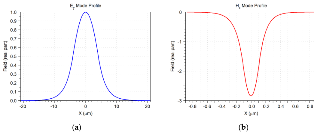
Figure 17. Electric (a) and magnetic (b) field distributions of the fundamental transverse electric mode (TE 00 ) of the single-mode optical fiber.
