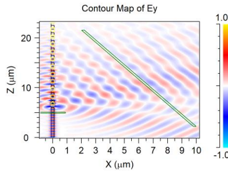
Figure 29. Representation on the XZ plane of the diffracted electric field, the green (transparent filled) horizontal bar is the waveguide's monitor and the slanted green (transparent filled) slanted bar is the diffracted field monitor. Image obtained from 2D-FDTD.
