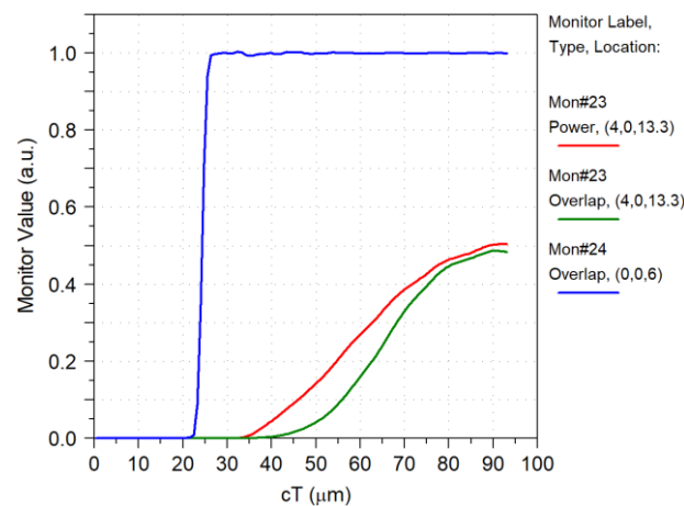
Figure 24. Efficiency test, from top to bottom, the blue line represents the overlap value (with the quasi- \text{TE}_{00} waveguide's mode) measured at 1 \mu\text{m} before the waveguide's end. The red and green
