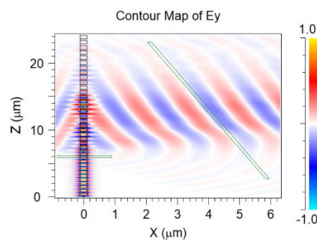
Figure 26. Representation on the XZ plane of the diffracted electric field, the green (transparent filled) horizontal bar is the waveguide's monitor and the slanted green (transparent filled) slanted bar is the diffracted field monitor. Image obtained from 2D-FDTD.
