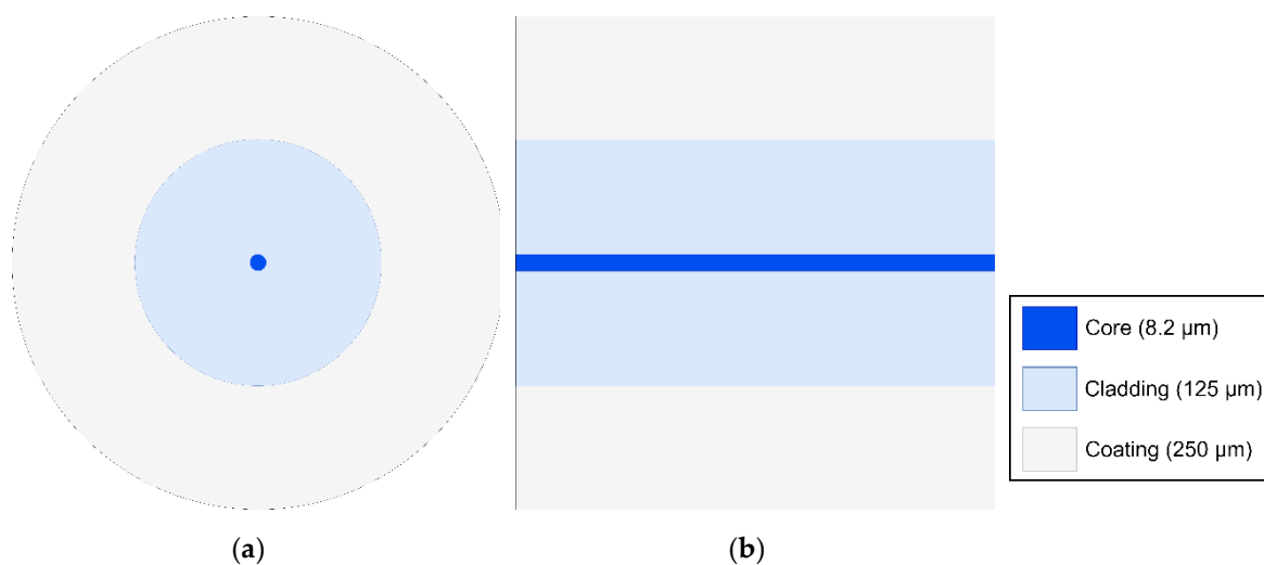
Figure 1. Two-dimensional representations of the SMF-28 optical fiber. (a) Transversal section; (b) Longitudinal cut. Both figures show (from center to periphery), core, cladding and coating. Coating is represented with a + 5 \mu\text{m} deviation from the nominal value.
