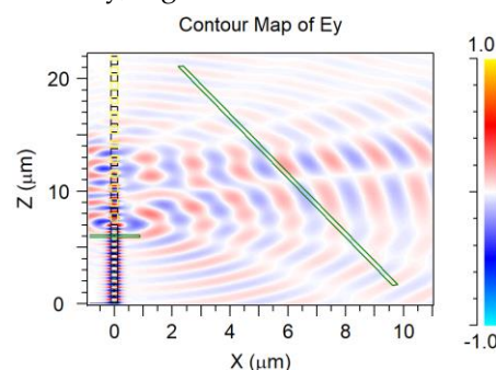
Figure 32. Representation on the XZ plane of the diffracted electric field, the green (transparent filled) horizontal bar is the waveguide's monitor and the slanted green (transparent filled) slanted bar is the diffracted field monitor. Image obtained from 2D-FDTD.
