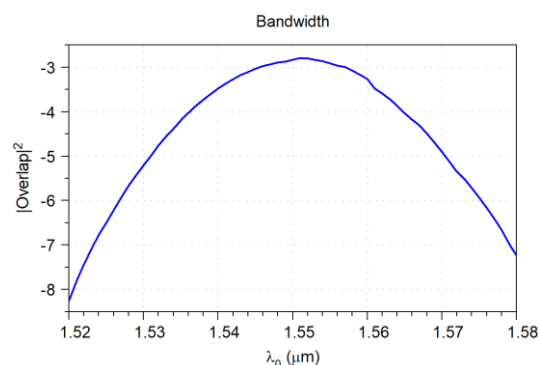
Figure 28. Overlap with the SMF-28 optical fiber TE 00 mode at the diffracted field monitor, obtained for different wavelengths. The |Overlap|^2 is given in logarithmic scale, decibel (dB), wavelength in vacuum (λ 0 ) is represented in linear scale.
