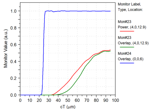
Figure 27. Efficiency test, from top to bottom, the blue line represents the overlap value (with the quasi-TE 00 waveguide's mode) measured at 1 μm before the waveguide's end (diffraction grating starting point). The red and green lines, represent the power and overlap (with the TE 00 mode of a simulated SMF-28 optical fiber) of the diffraction field, respectively, measured at a monitor whose center is at a distance of 4 μm from the grating.
