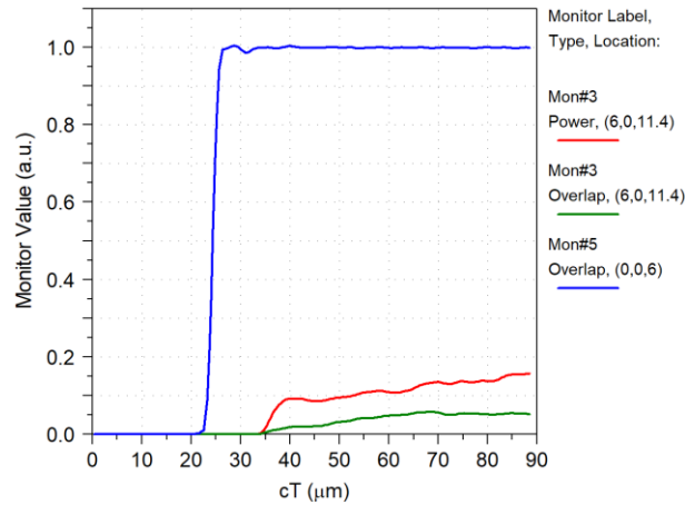
Figure 33. Efficiency test, from top to bottom, the blue line represents the overlap value (with the quasi-TE 00 waveguide's mode) measured at 1 \mu\text{m} before the waveguide's end. The red and green lines, represent the power and overlap (with the TE 00 mode of a simulated SMF-28 optical fiber) of the diffraction field, respectively measured at a monitor whose center is at a distance of 6 \mu\text{m} from the grating's center.
