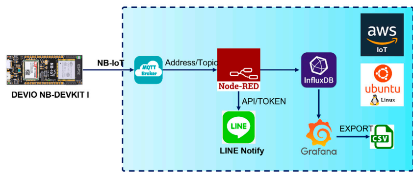
Figure 5. Online monitoring and real-time data logger.
