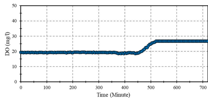
Figure 14. The result of the DO value affected by Automatic Paddle Wheel Aerator.
