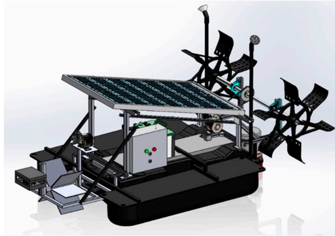
Figure 4. The architectural design of a paddle wheel aerator robot.
