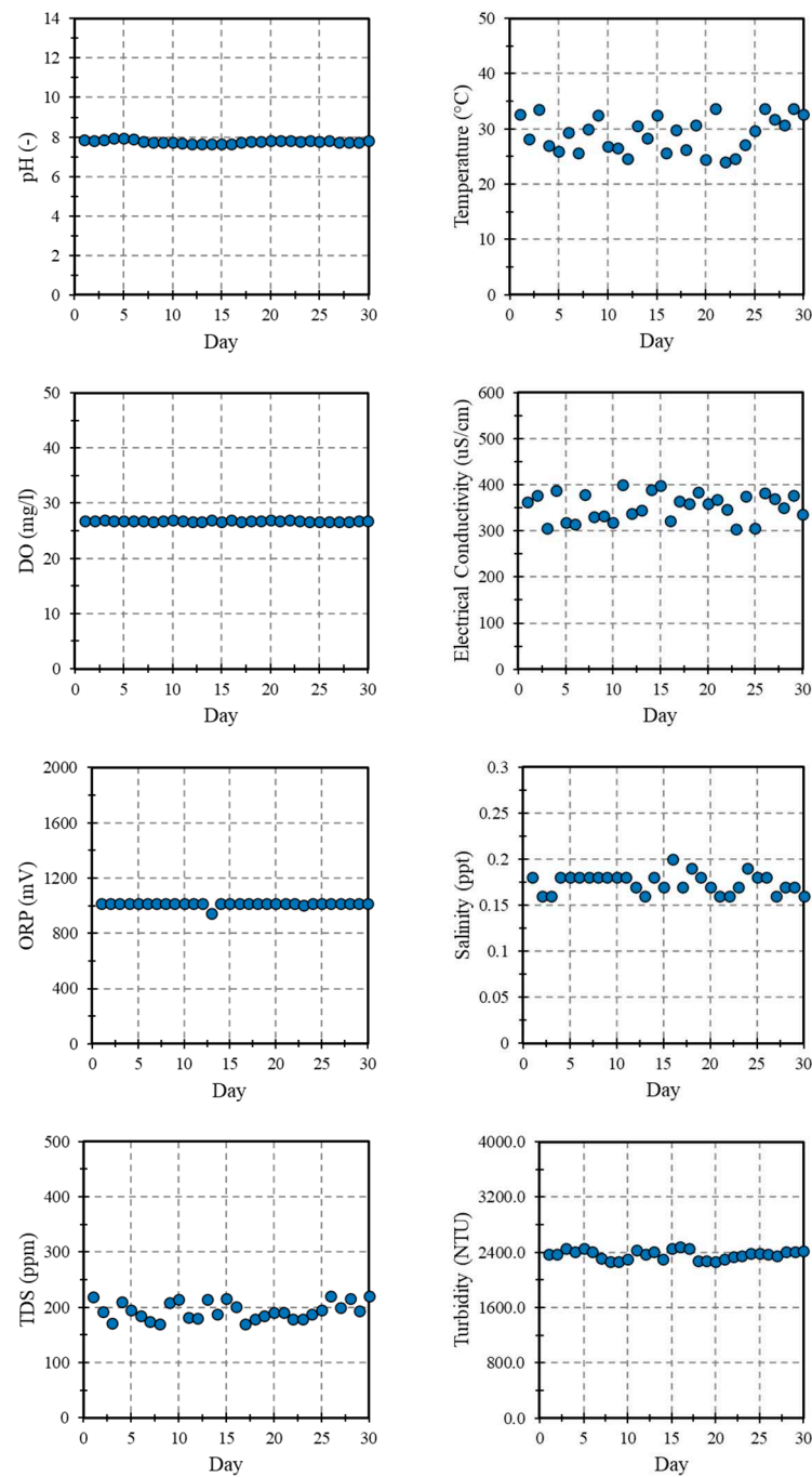
Figure 13. pH, Temperature, DO, Conductivity, ORP, Salinity, TDS, and turbidity at location 3.
