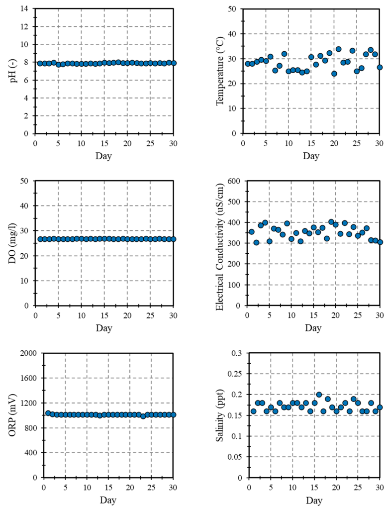
Figure 11. pH, Temperature, DO, Conductivity, ORP, Salinity, TDS, and turbidity at location 1.
