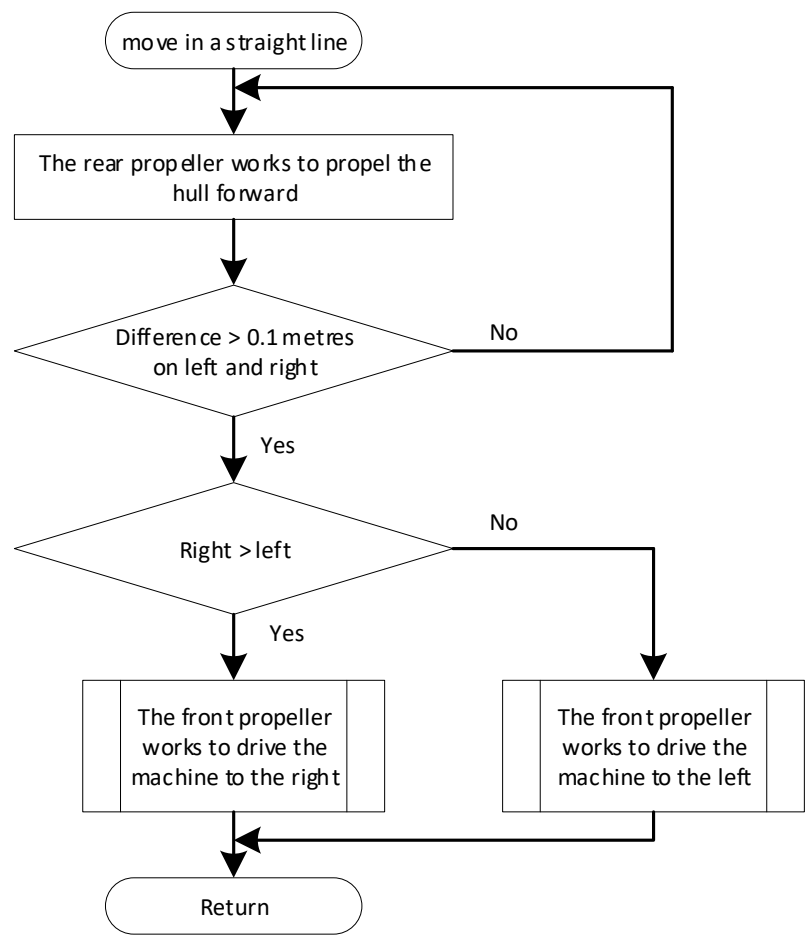
Figure 8. Flowchart of boat movement.
