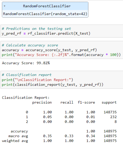
Figure 10. Evaluation of Random Forest Classifier
