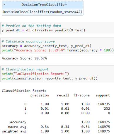
Figure 12. Evaluation Performance of Decision Tree Classifier
