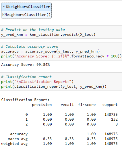
Figure 11. Evaluation of KNN Classifier
