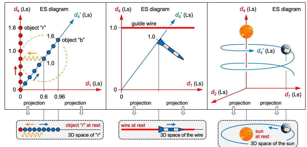
Fig. 5 Solving problems in ER. Left: The orange circle shows where the radio signal is 0.6 s after its emission. In ES, an energy taking a detour (blue and orange arrow) cannot collide with an energy moving straight (red arrow). In 3D space, it can. Center: In ES, the wire escapes from the rocket. In 3D space, it does not. Right: In ES, the sun escapes from Earth's orbit. In 3D space, it does not.
