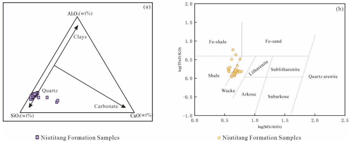
Figure 12. a. Ternary Diagram of Relative Proportions of Major Elements (base map according to Cong He et al., 2016) [44]; Figure 12b. Geochemical Classification of Core Samples from SZY1 Well (base map can refer to MICHAEL M. HERRON 1988; Cong He 2016) [44,45] (note: all data in the figure are from actual measured core samples of the Niutitang Formation shale from SZY1 well).
