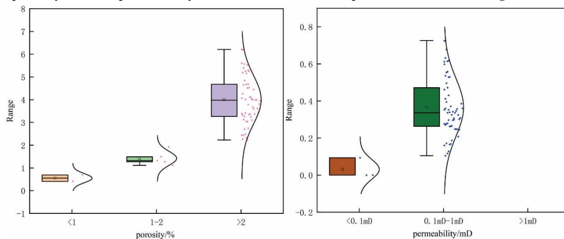
Figure 8. Box Plot of Reservoir Physical Properties of Niutitang Formation in the Study Area (note: all data in the figure are from actual measured core samples of the Niutitang Formation shale from SZY1well).
