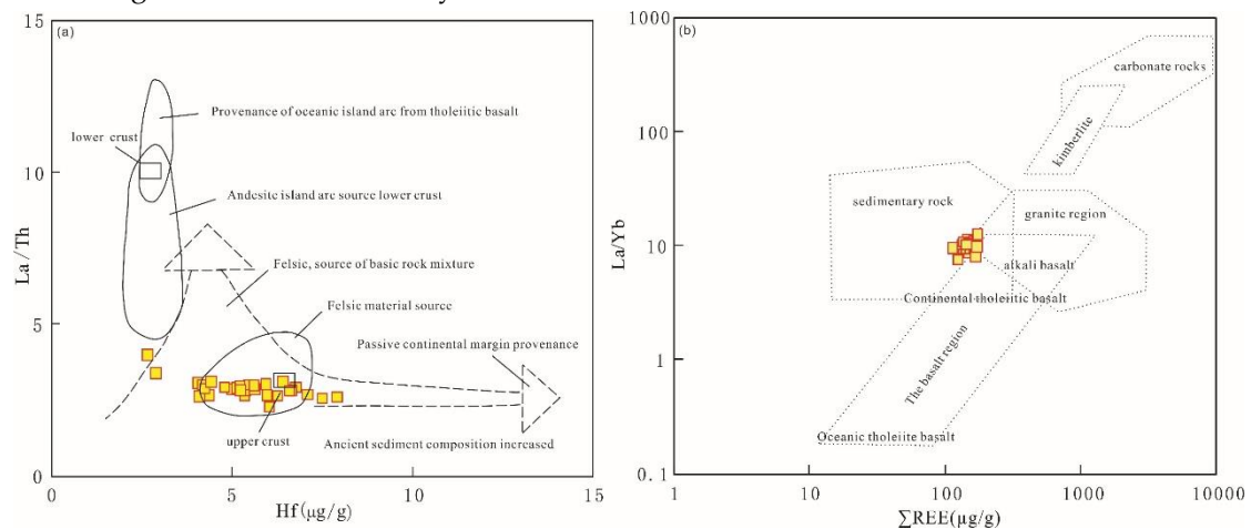
Figure 17. Provenance Rock Attribute Discriminant Diagram for Shale from Niutitang Formation in Zhenba Area (a. Base map according to Floyd P A et al. (1987) [60] b. Base map according to Allègre
