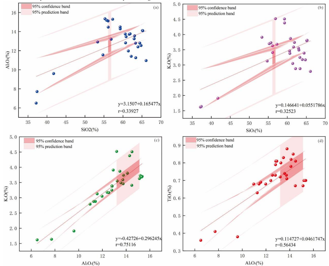
Figure 13. Relationship between SiO 2 , Al 2 O 3 , K 2 O, and TiO 2 Contents in Shale Samples (Note: All samples in the figure are from Niutitang Formation shale, They are the same samples, with different colors used in the figure. Figure 13.a shows the relationship between Al 2 O 3 and SiO 2 , Figure 13.b
