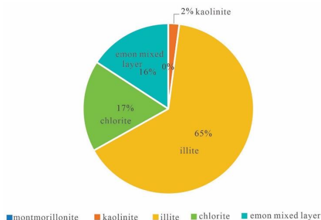
Figure 5. Relative content map of clay minerals in Niutitang Formation shale of the study area. (note: all data in the figure are from actual measured core samples of the Niutitang Formation shale from SZY1well).
