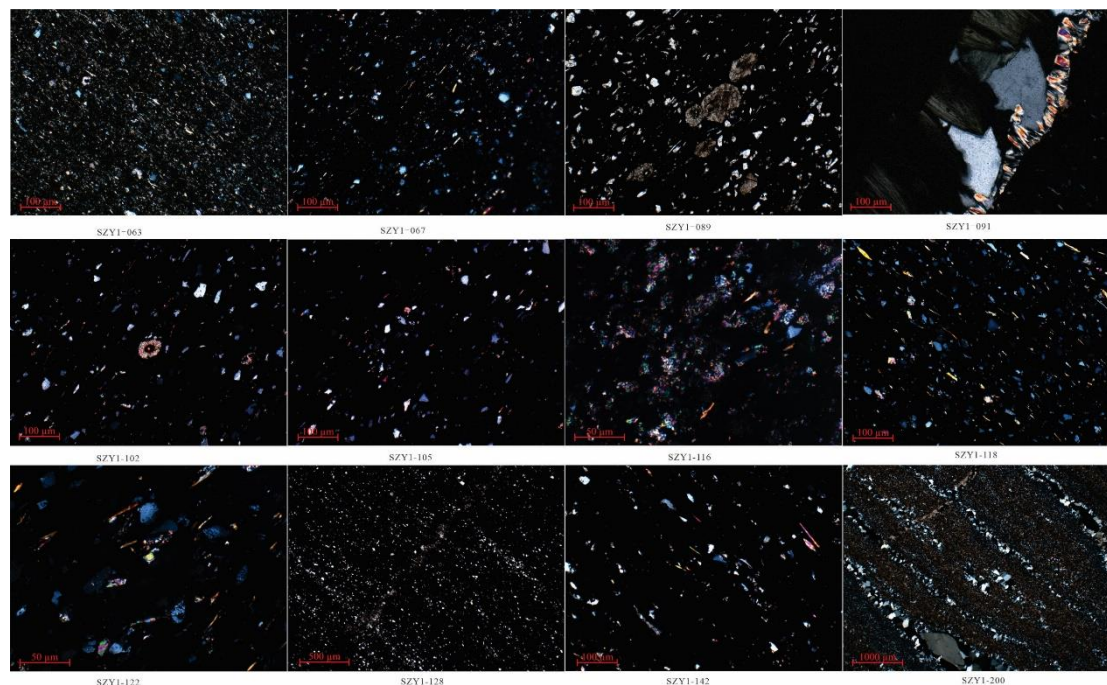
Figure 6. Mineralogical and Petrographic Characteristics of Niutitang Formation in the Study Area.
