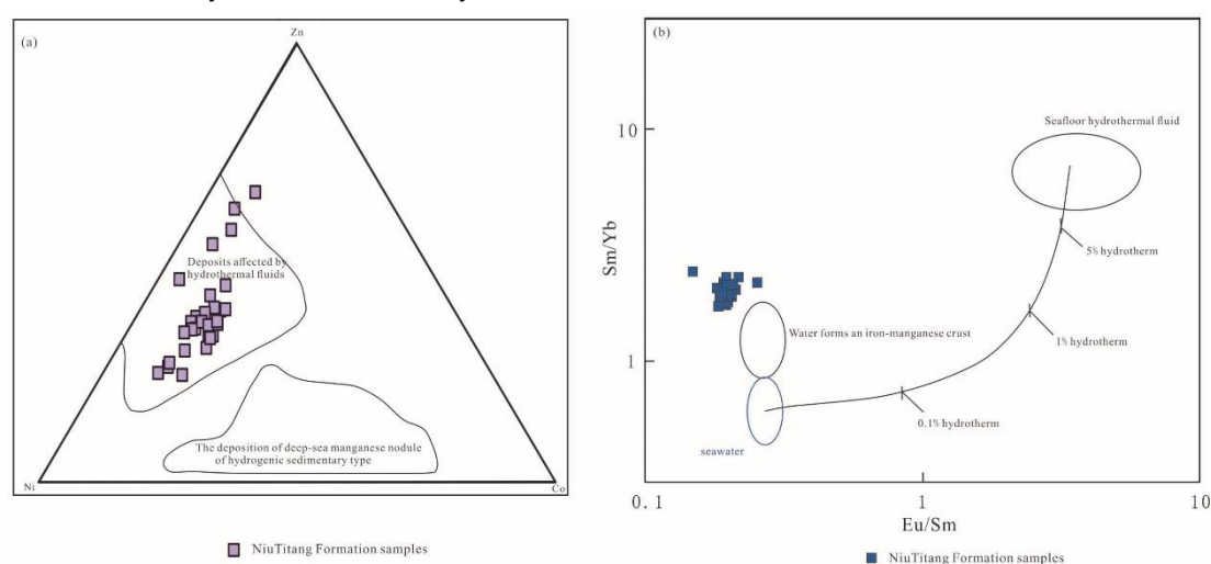
Figure 18. Provenance Discriminant Diagram for Shale from Niutitang Formation in Zhenba Area (a. Base map according to Cronan D S et al. (1980) [64] b. Base map according to Alexander B W et al. (2008) [65]) (note: all data in the figure are from actual measured core samples of the Niutitang Formation shale from SZY1well).
