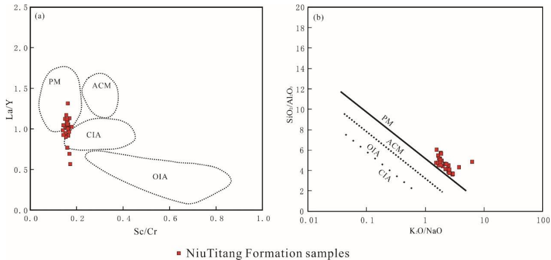
Figure 16. Tectonic Setting Discriminant Diagrams for Shale Samples from Niutitang Formation in the Zhenba Area (a) A plot of Sc/Cr versus La/Y, with the base map according to Roser B P et al. (1988) [56]; (b) A plot of K 2 O/Na 2 O versus SiO 2 /Al 2 O 3 , with the base map according to Bhatia M R et al. (1986) [57]; ACM. Active Continental Margin; PM. Passive Continental Margin; CIA. Continental Island Arc; OIA. Oceanic Island Arc (note: all data in the figure are from actual measured core samples of the Niutitang Formation shale from SZY1 well).
