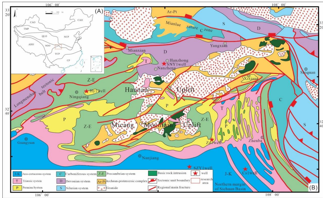
Figure 1. Geologic map of the Zhenba area and its surrounding region (A: Tectonic divisions of China, AHO-Alpine-himalayan orogenic belt, CAO-Central Asian Orogenic Belt, CP-Cathaysia, NCP-North China Plate, QLO-Qinling Orogenic Belt, SGO-Songpan-Ganzi Orogenic Belt, TMP-Tarim Plate, YCP-Yangtze Plate, B: Geologic map of the Zhenba area and its surrounding region).
