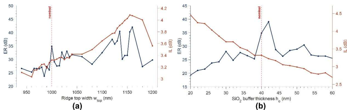
Figure 7. Fabrication tolerance of the polarizer to the two dielectric geometric parameters at the optimized point ( \theta = 78^\circ , h_m = 13 nm, \lambda = 1550 nm, T = 25 °C); PER (left axis, blue) and IL (right axis, orange). (a) Ridge top width w_{top} over 940–1200 nm; (b) SiO 2 buffer thickness h_o over 20–60 nm. The dotted line marks the nominal value.
