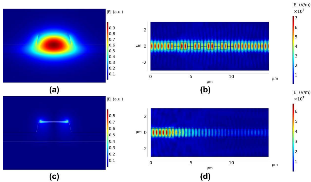
Figure 3. Electric-field distributions of the HPG polarizer at \theta = 78^\circ , h_m = 13 nm, \lambda = 1550 nm, T = 25 °C. (a,c) Two-dimensional cross-sectional mode profiles |E| (normalized) of (a) the TE 0 mode and (c) the hybrid TM mode; (b,d) three-dimensional propagation profiles along Y direction for (b) TE and (d) TM input.
