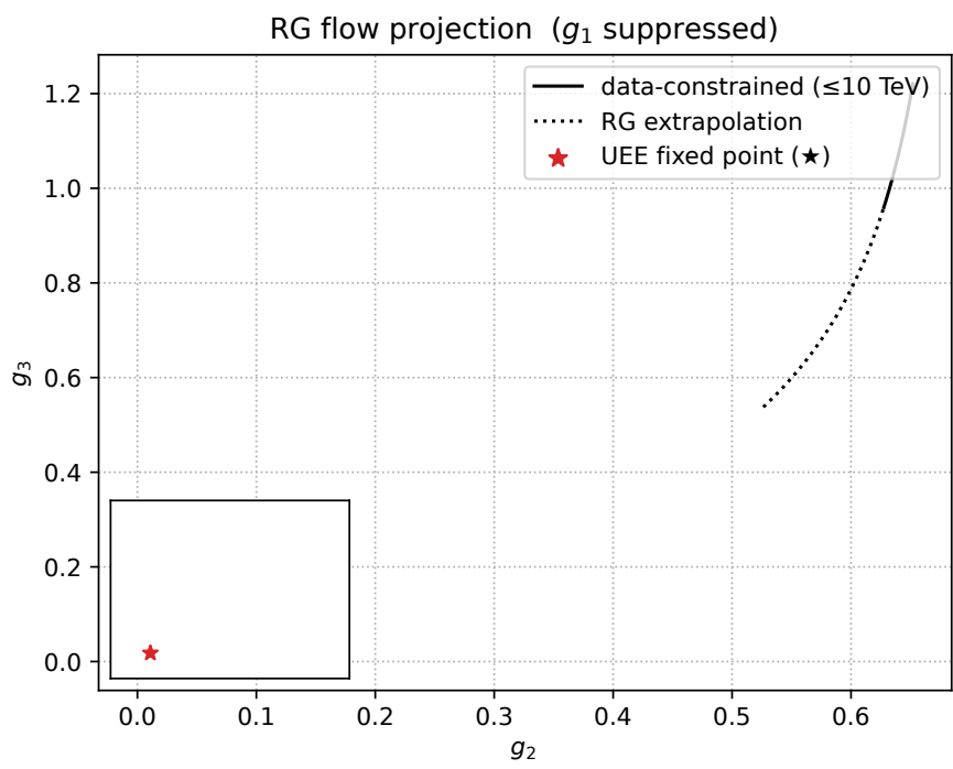
Figure A10. Projection onto the g_2 - g_3 plane. Symbols as in Fig. A9.
