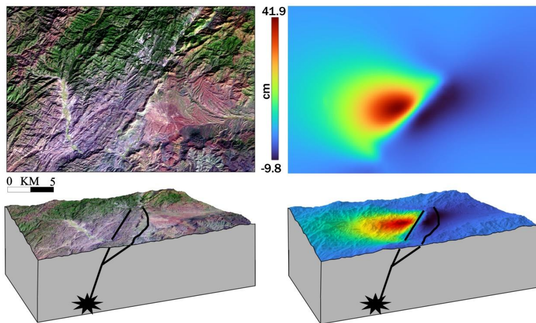
Figure 10. The top panel shows the active fault derived from a) surface topography and b) Co-seismic LOS displacements. The lower panel shows the respective 3-D perspective views of the active fault derived from a) surface topography and b) Co-seismic LOS displacements. The star shows the focus of the earthquake and black bold lines in section view are sub-surface reconstructions of the active faults.
