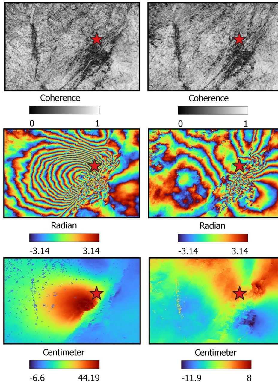
Figure 8. InSAR results for the 21 June, 2022 earthquake, USGS epicentre shown by the red star. Results from the Ascending mode (left panel) and Descending mode (right panel). Coherence maps (top panel), phase change fringes (middle panel) and LOS displacement (bottom panel).
