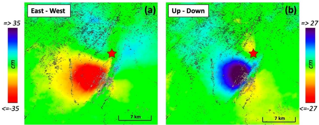
Figure 4. Horizontal (East-West) and Vertical (Up – Down) displacement component of coseismic results relevant to the 21 June 2022 earthquake of Eastern Afghanistan. (a) East – West and (b) Up – Down coseismic displacement maps, respectively.
