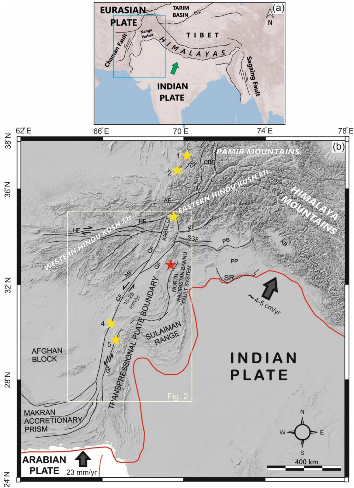
Figure 1. The India-Asia convergence zone a) showing the major thrusts towards the north generating the Himalayan mountain belt and the western and eastern boundary showing the major strike-slip faulting along
