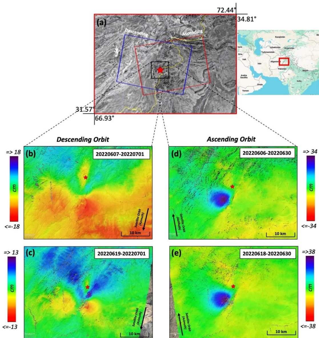
Figure 3. Sentinel-1A coseismic LOS displacement results relevant to the 21 June 2022 earthquake of Eastern Afghanistan. (a) indicates the Sentinel-1A footprints used to cover the area of interest (Ascending orbit red line and Descending orbit blue line). (b) and (c) show the coseismic LoS displacement maps for the descending orbit. (d) and (e) show coseismic LOS displacement maps for the ascending orbit.
