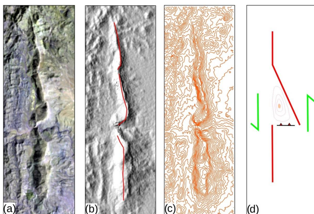
Figure 7. The arrangement of right stepping fault bends forming a segmented ridge topography in a left-lateral environment. a) as seen on Satellite Image b) as seen in DEM, the red lines follow the ridge top c) contours for better visualization and d) Schematic model showing evolution of the observed fault bend and related ridge topography across the fault step-overs. The contours inside the bend show the ridge topography (high in the centre).
