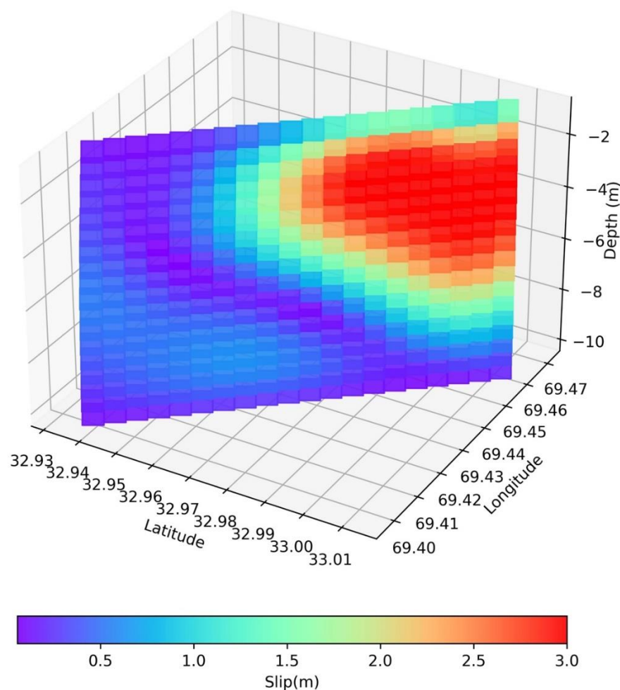
Figure 9. The 21 June, 2022 Afghanistan earthquake fault model showing variable slip distribution along the fault plane.
