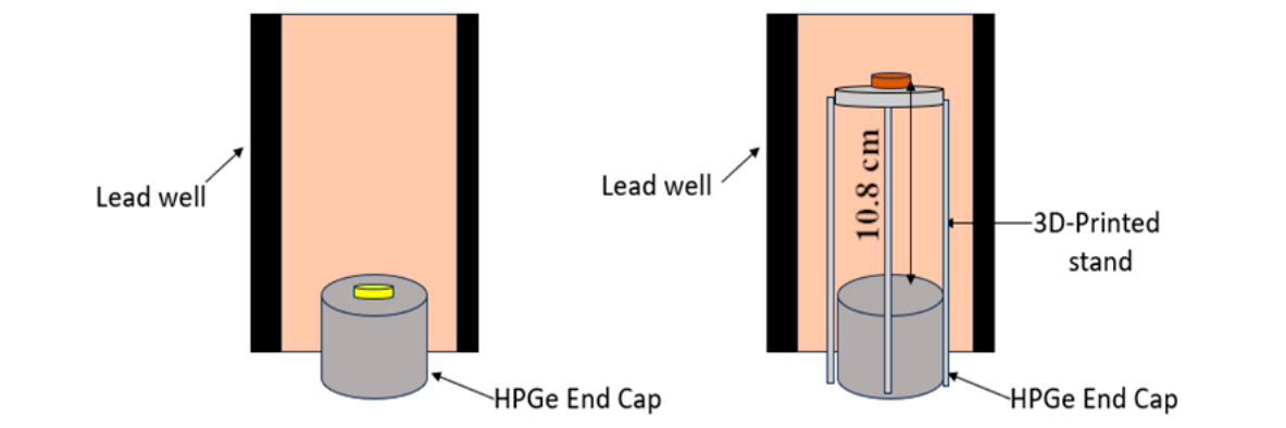
Figure 7. (a) Experimental setup for measuring gold foils. (b) Experimental setup for a 3D printed stand for measuring indium foils.
