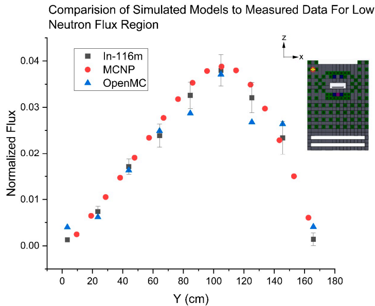
Figure 16. Normalized In-116m foils compared to MCNP and OpenMC at the low neutron flux region within the pile.
