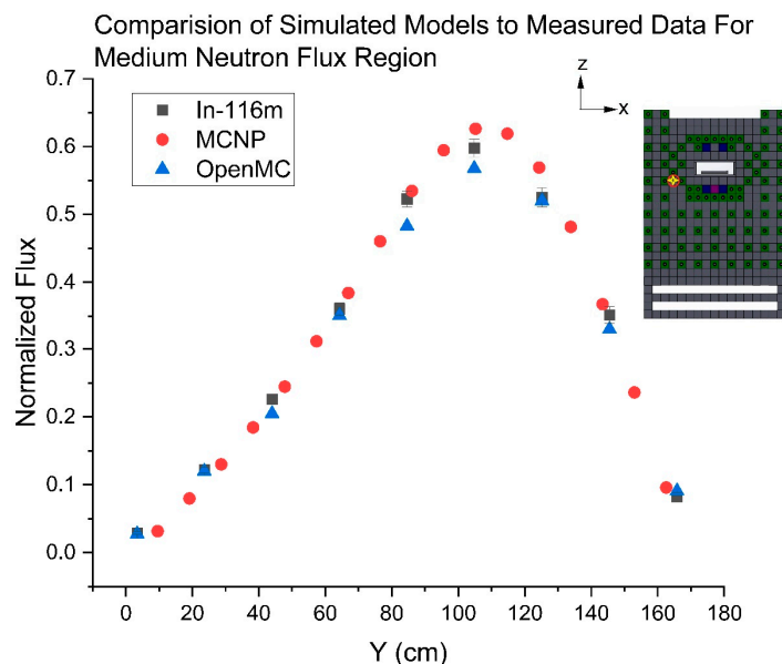
Figure 17. Normalized In-116m foils compared to MCNP and OpenMC at the medium neutron flux region within the pile.
