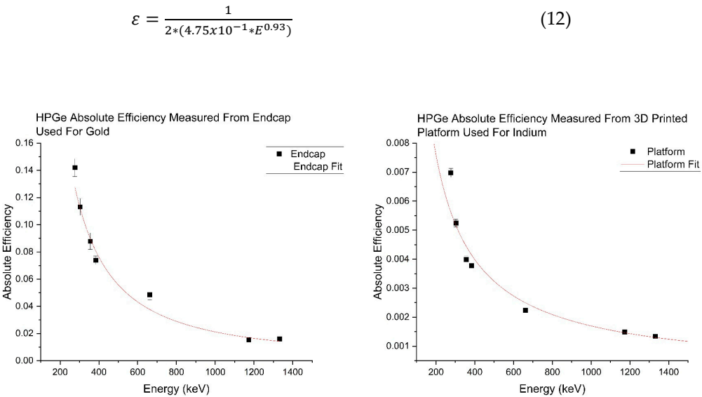
Figure 9. Absolute Photopeak Efficiency for HPGe Detector used for gold and indium experiments using Ba-133, Co-60, Cs-137.
