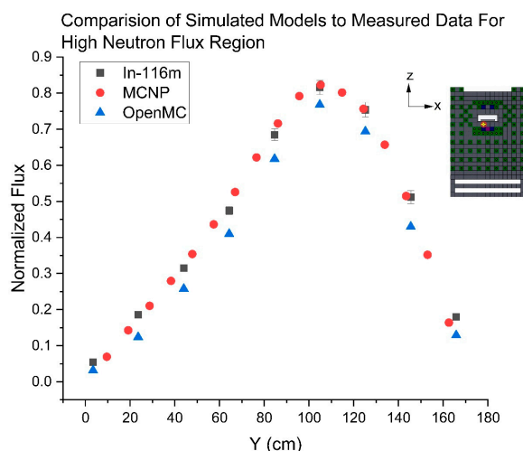
Figure 18. Normalized In-116m foils compared to MCNP and OpenMC at the high neutron flux region within the pile.
