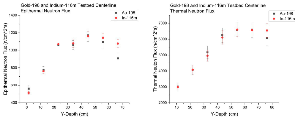
Figure 12. (a) Average epithermal neutron flux along testbed centerline. (b) Average thermal neutron flux along testbed centerline.
