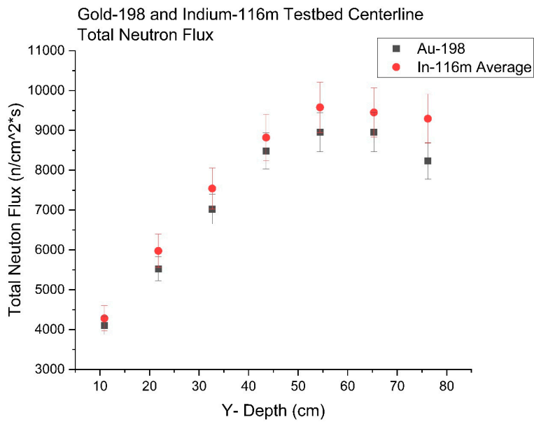
Figure 10. Comparison of average neutron flux in the testbed calculated by gold and indium foils. Error bars represent 1σ uncertainty.
