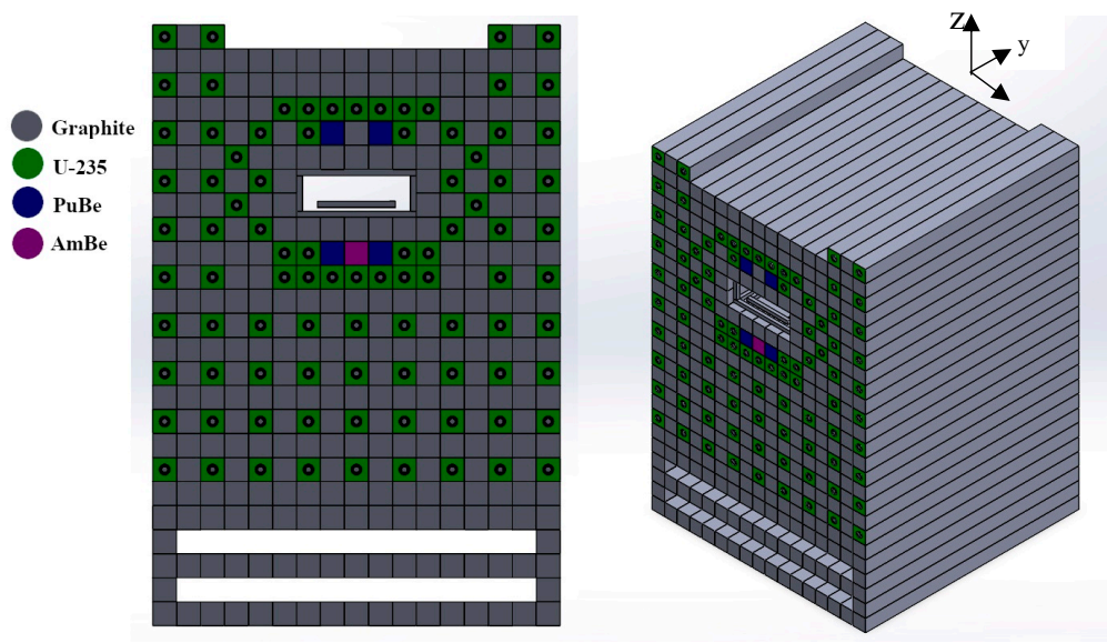
Figure 1. 3D SolidWorks of subcritical pile with testbed integration.
