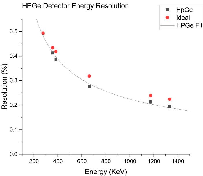
Figure 8. Comparison of HPGe Energy resolution to ideal resolution. Fit: y = 13.6(x)^{-0.6} .
