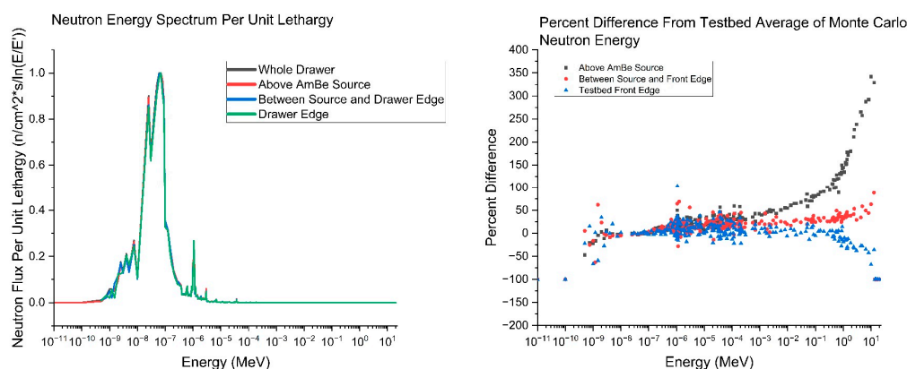
Figure 19. (a) Neutron energy spectrum within the testbed region. (b) Percent difference in neutron energy compared to the testbed average.
