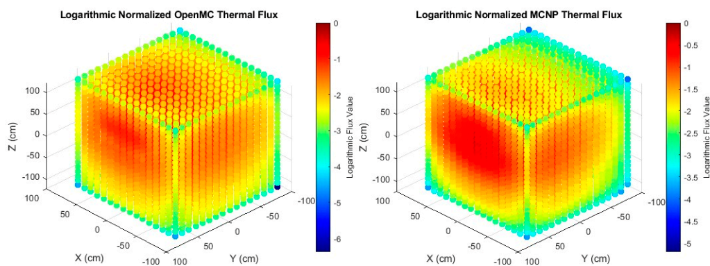
Figure 6. (a) Normalized neutron flux for the OpenMC model. (b) Normalized neutron flux for the MCNP model.
