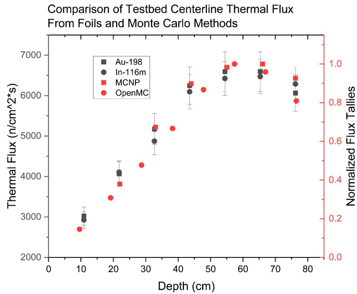
Figure 15. Comparison of measured thermal flux to normalized OpenMC and MCNP tallies within the testbed region.
