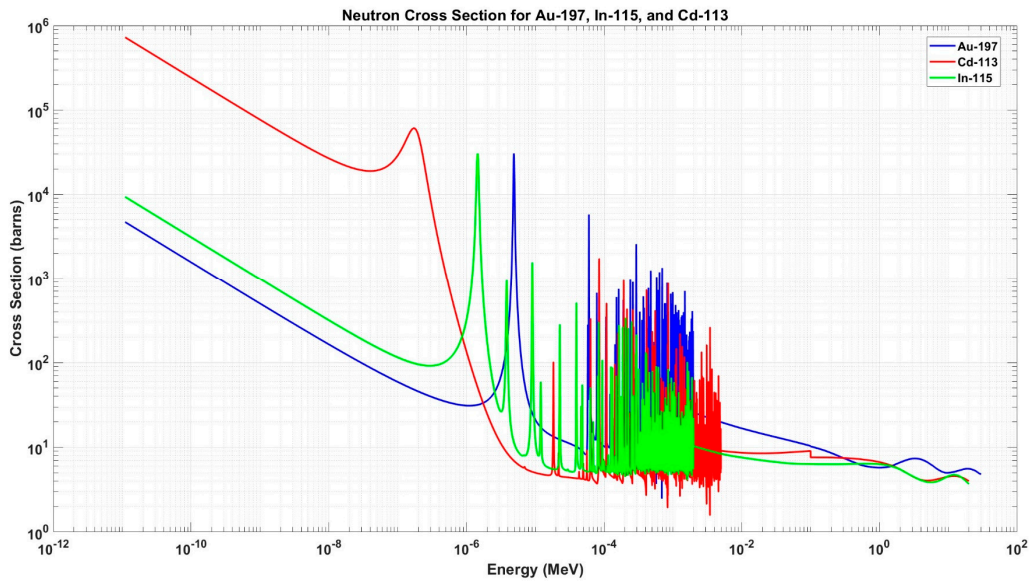
Figure 5. Neutron capture cross-section data for Au-197, In-115, and Cd-113. [20] [21] [22].
