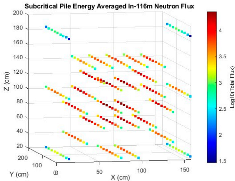
Figure 13. Flux map of the entire pile as measured by indium foils.
