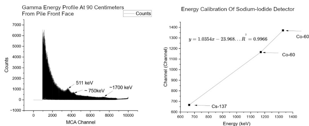
Figure 14. (a) The gamma energy spectrum measured at 90 centimeters from the front face of the pile. (b) Energy calibration for the sodium-iodide detector.
