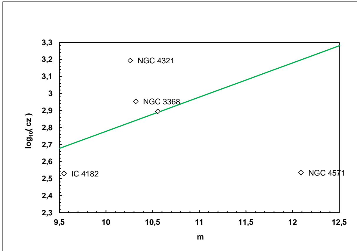
Figure 4. Magnitude-redshift diagram for the galaxies NGC 4321, NGC 4571, NGC 3368 and IC 4182
