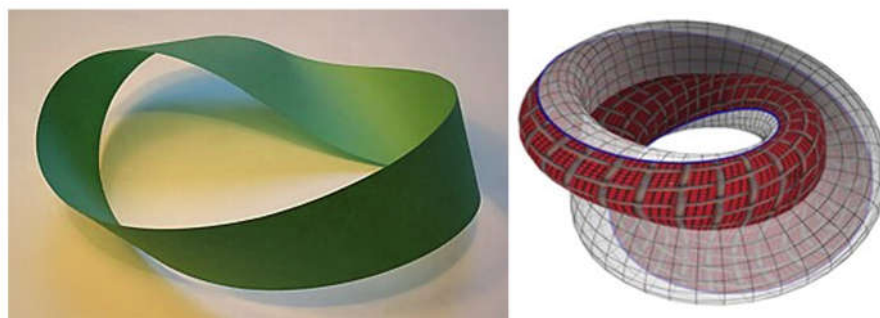
Figure 4. Mobius Band (left) and figure-8 Klein Bottle (right). The bottle may be called a Mobius Doublet since it's formed from the union of two bands. Trillions of bands/bottles may respectively form photons/gravitons which Albert Einstein suspected might interact to produce elementary particles. (Mobius figure from https://upload.wikimedia.org/wikipedia/commons/thumb/7/79/M%C3%B6bius_Strip.jpg/320px-M%C3%B6bius_Strip.jpg . Klein fig. from http://plus.maths.org/content/os/issue26/features/mathart/index ).
