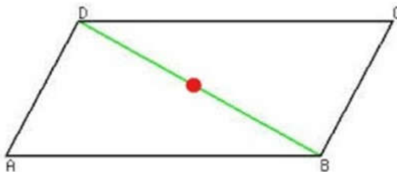
Figure 1. Vector-Tensor-Scalar Geometry: Parallelogram With Diagonal and Central Higgs Boson (Horizontal Direction = Graviton Vector; Vertical = Photon Vector). The deep link between geometry and
