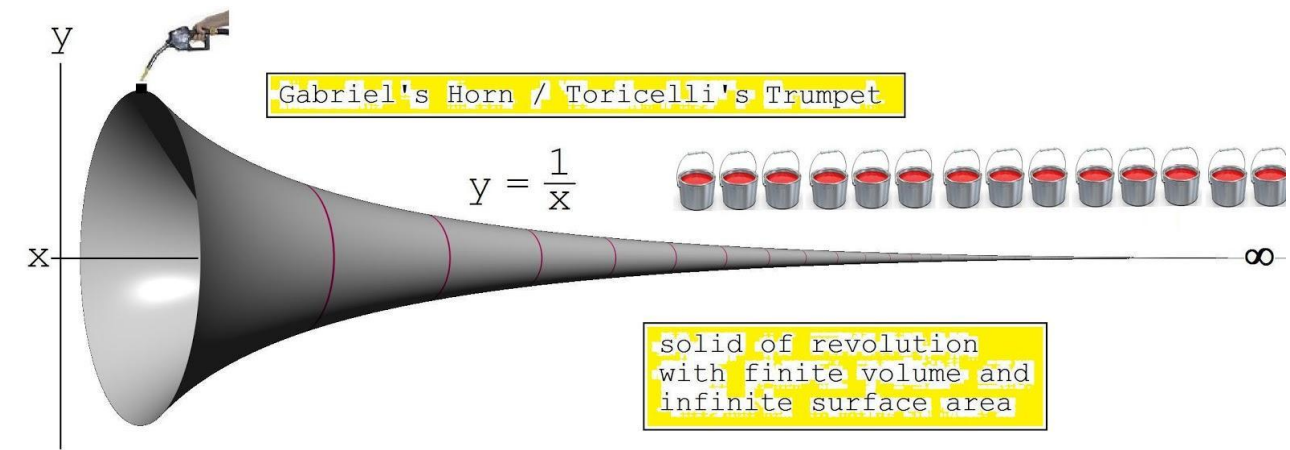
Figure 1. Gabriel’s Horn / Toricelli’s Trumpet.
