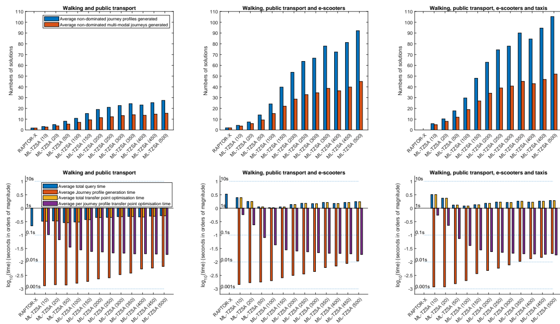
Figure 7. Average numbers of solutions and query times for ML-TZSA and RAPTOR methodologies for different sets of available modes, based on 2000 example commuter queries.
