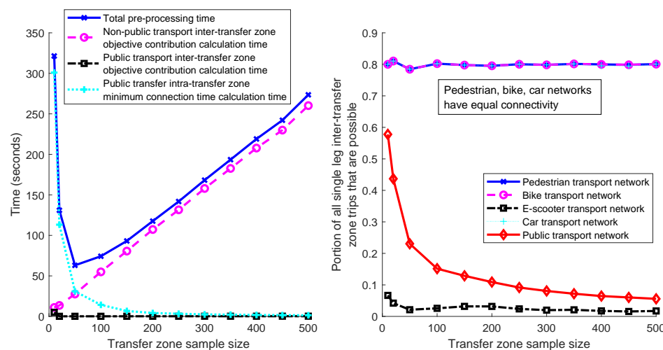
Figure 6. Left: Pre-processing times and their components. Right: The connectivity of different transport networks measured as the portion of all single leg inter-transfer zone trips that are possible.
