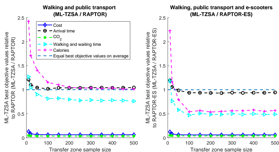
Figure 8. Left: Average best ML-TZSA objectives relative to RAPTOR for the case of walking and public transport being available. Right: Average best ML-TZSA objectives relative to RAPTOR-ES for the case of walking, public transport and e-scooters being available.
