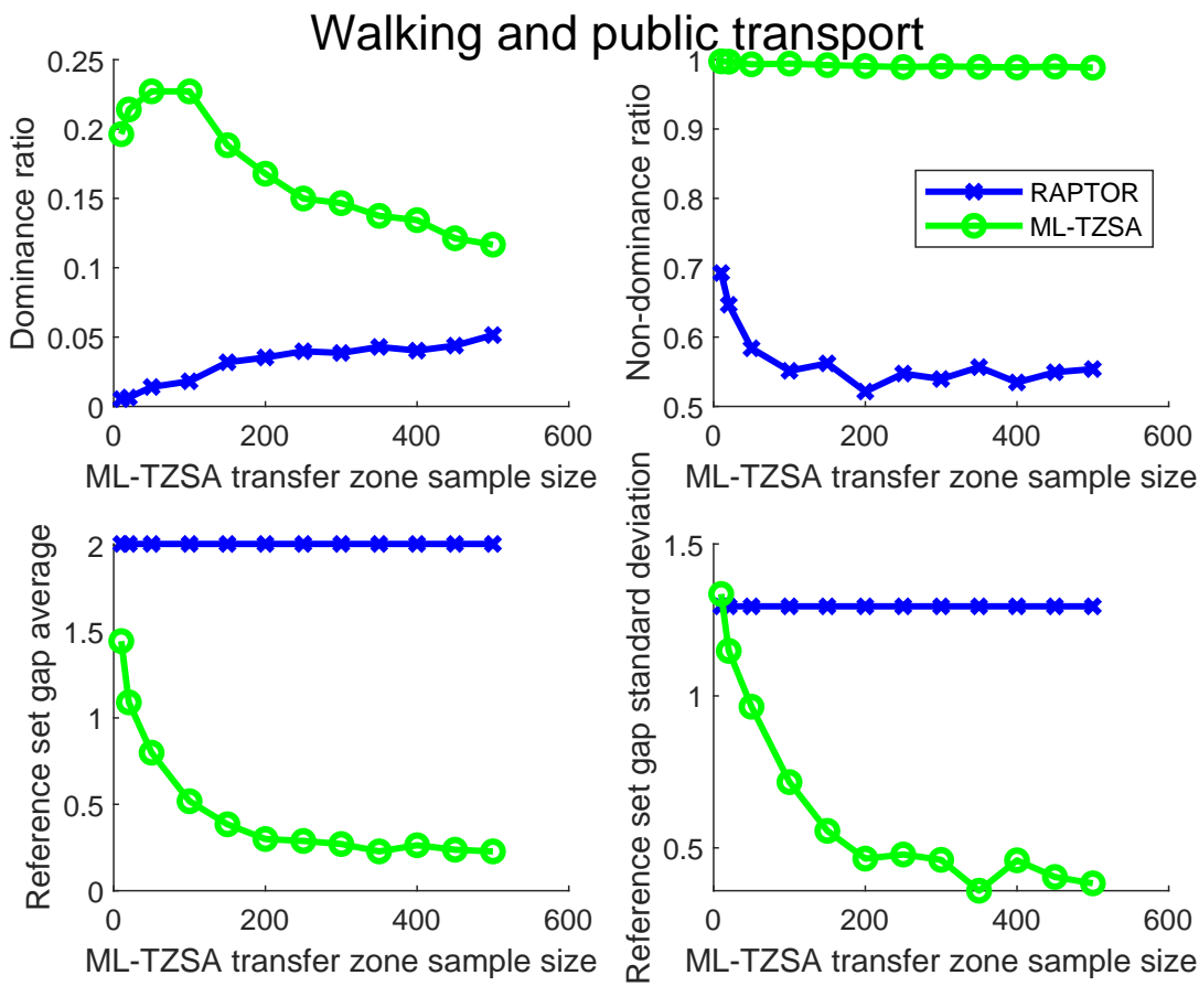
Figure 10. Dominance ratio, non-dominance ratio, reference set gap average and standard deviation results for the case of walking and public transport.
