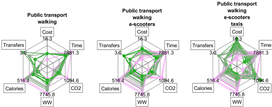
Figure 13. Spider plots of pareto fronts for different sets of available transport modes, with individual solutions coloured according to travel time.
