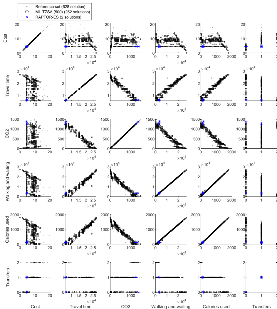
Figure 12. Pareto front objective criteria scatter plots for ML-TZSA (500), RAPTOR and the reference set for the query depicted in Figure 9 displaying the nature of the trade-offs between each criterion.
