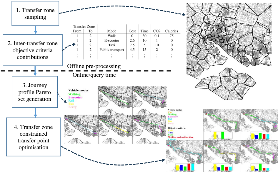
Figure 1. Overview of ML-TZSA.
