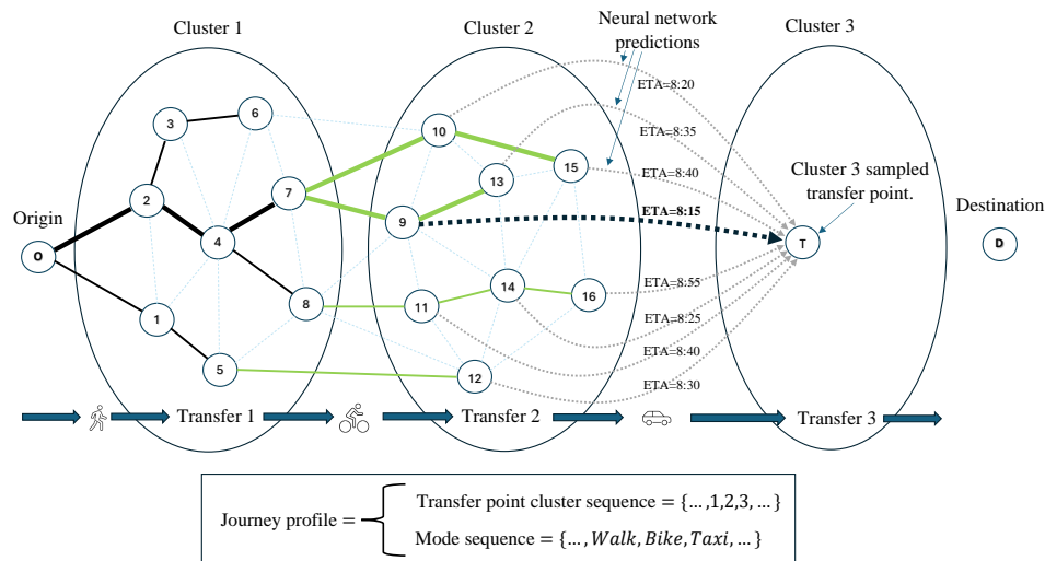
Figure 5. Diagram illustrating how machine learning predictions of travel times of the subsequent leg of a multi-modal journey, starting from different possible transfer zones, are used to select the transfer point of the previous leg.
