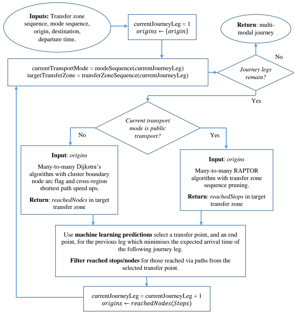
Figure 3. Flow chart for the machine learning prediction guided transfer point optimisation procedure.
