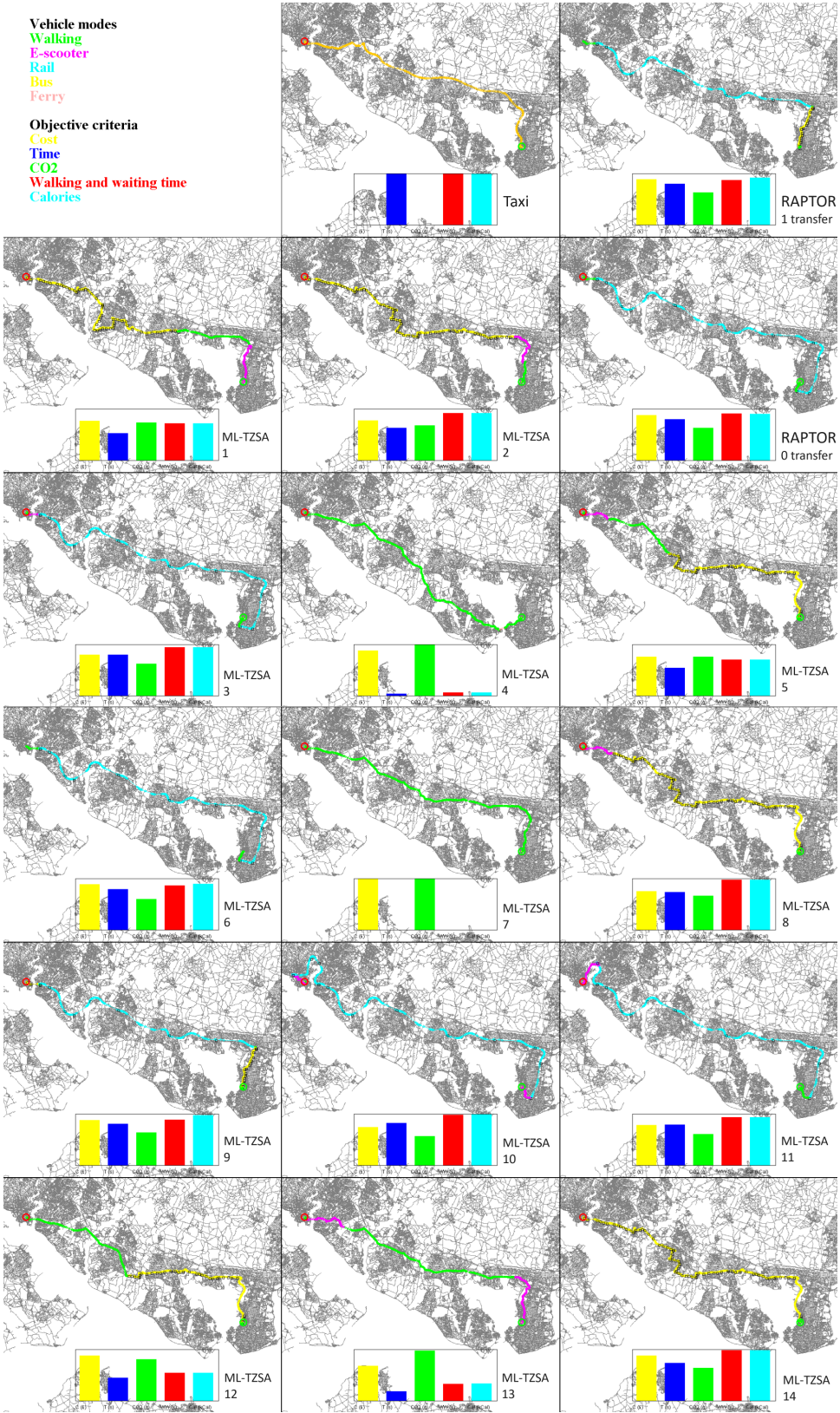
Figure 9. A sample of the 252 non-dominated journeys generated by ML-TZSA (500), RAPTOR-ES’s two non-dominated journeys, plus a taxi journey for an example query.
