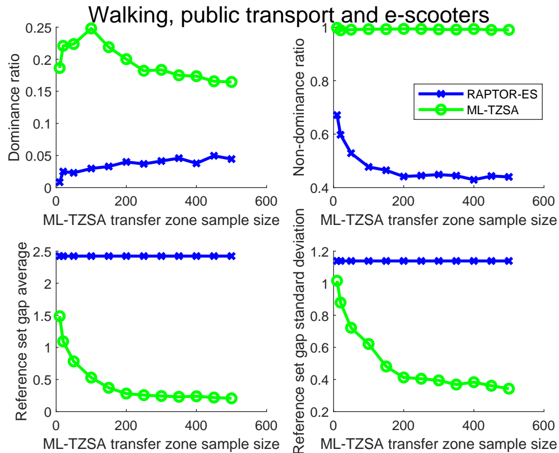
Figure 11. Dominance ratio, non-dominance ratio, reference set gap average and standard deviation results for the case of walking, public transport and e-scooters.
