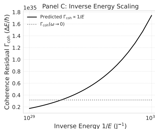
Figure 3. Panel C presents the inverse energy scaling relationship, plotting the coherence residual linewidth \Gamma_{\text{coh}} against the inverse energy scale 1/E . The linear dependence demonstrates that the cost of maintaining coherence decreases as structural complexity increases, consistent with the dimensional identity \Delta C_T = J^{-1} . This scaling law provides a quantitative validation of Mode 2 coherence [11] and confirms the dimensional consistency of the First Law of Coherence Thermodynamics. The plot thus operationalizes the principle that residual linewidths encode the energetic footprint of structural learning in complex systems.
