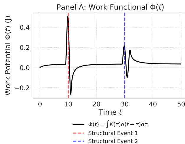
Figure 1. Panel A illustrates the time-domain accumulation of the coherence restructuring work \Phi(t) obtained by convolving the non-Markovian memory kernel K(\tau) with the restructuring rate \dot{a}(t) . The curve shows how discrete restructuring events (marked by vertical dashed lines) contribute to the cumulative potential, demonstrating that the field's work is conditioned by its entire history. This accumulated memory proves that residual coherence work is not instantaneous but a learning process of the infinite field, consistent with the First Law of Coherence Thermodynamics.
