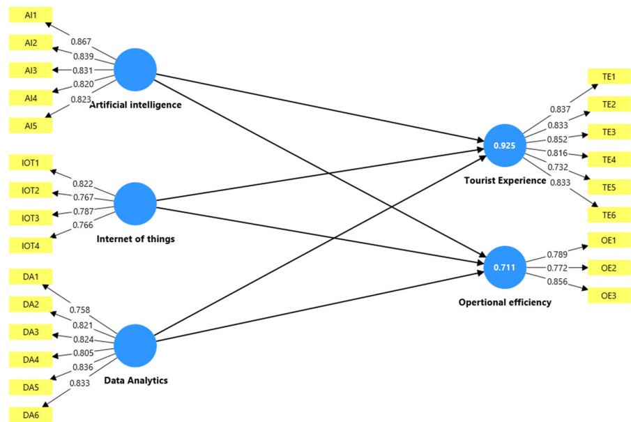
Figure 1. Measurement Model.
