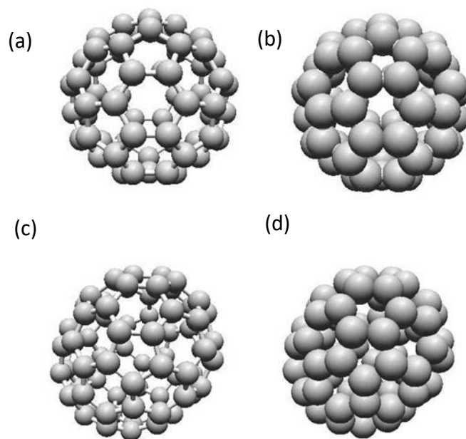
Figure 5. (a) Ball-and-stick model of fullerene C_{60} , (b) Sphere-in-contact model of fullerene C_{60} , (c) Ball-and-stick model of fullerene C_{70} 5Dh and (d) Sphere-in-contact model of fullerene C_{70} 5Dh. Image produced in Nanotube Modeler Software.
