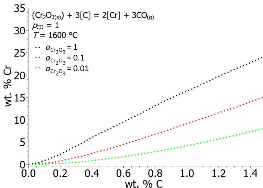
Figure 6. Equilibrium solubility of Cr and C in liquid iron at different activity of chromium oxide.
