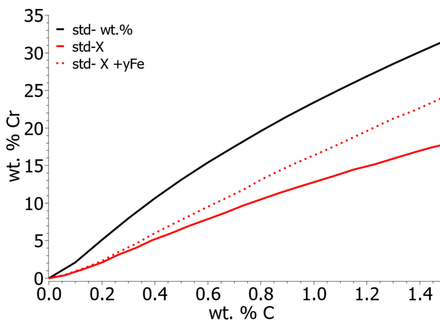
Figure 3. Equilibrium solubility of Cr and C in liquid iron calculated according to different standard states.
