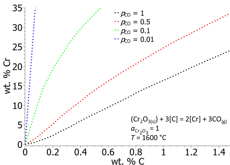
Figure 7. Equilibrium solubility of Cr and C in liquid iron at different partial pressures of carbon monoxide.
