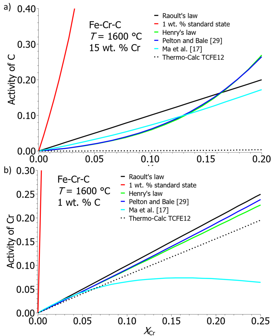
Figure 4. a) Activity of carbon in iron solution with 15 wt. % Cr, b) activity of chromium in iron solution with 1 wt. % C.
