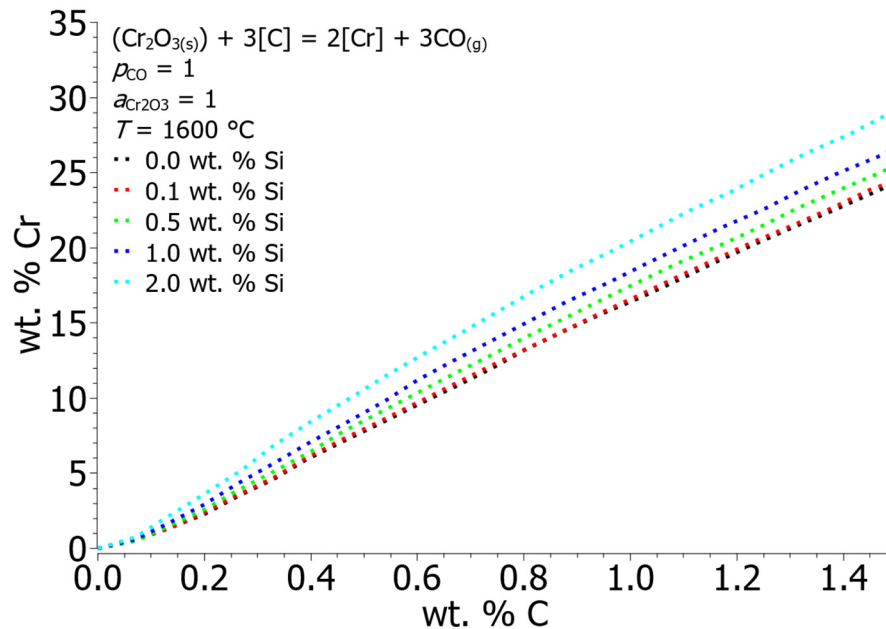
Figure 8. Equilibrium concentrations of Cr and C at different concentrations of Si in iron liquid solution at a temperature of 1600 °C.
