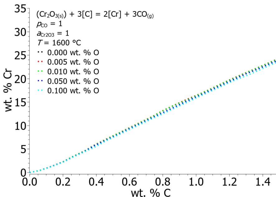
Figure 9. Equilibrium concentrations of Cr and C at different concentrations of O in iron liquid solution at a temperature of 1600 °C.
