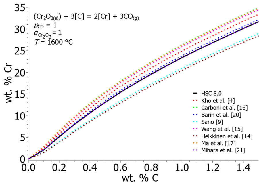
Figure 1. Equilibrium solubility of Cr and C in liquid iron considering different Gibbs free energies.
