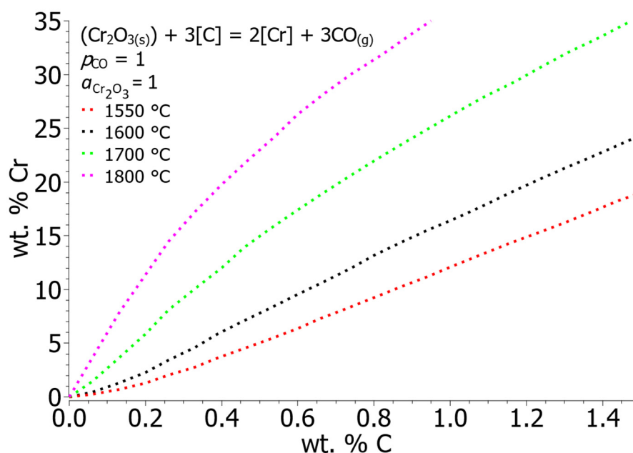
Figure 5. Equilibrium solubility of Cr and C in liquid iron between 1550 and 1800 °C.
