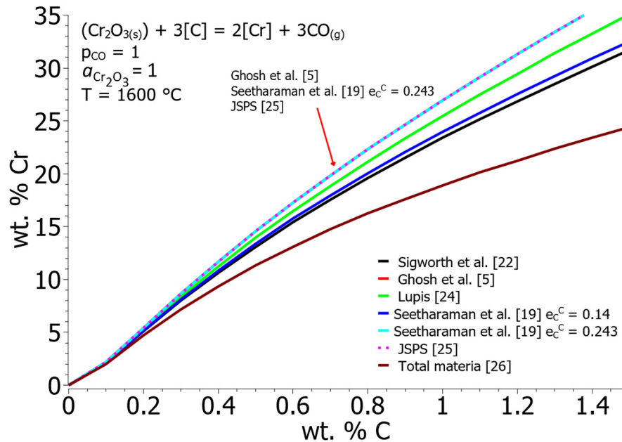
Figure 2. Equilibrium solubility of Cr and C in liquid iron considering different interaction parameters.
