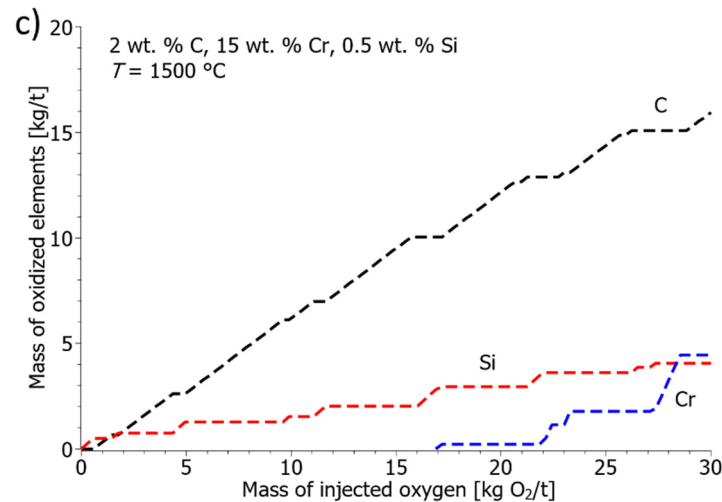
Figure 11. Oxidation of C, Cr, and Si in steel melt with 15 wt. % Cr and 2 wt. % C. a) Oxidation start temperature 1500 °C, b) oxidation start temperature 1650 °C and c) oxidation start temperature 1500 °C with 0.5 wt. % Si.
