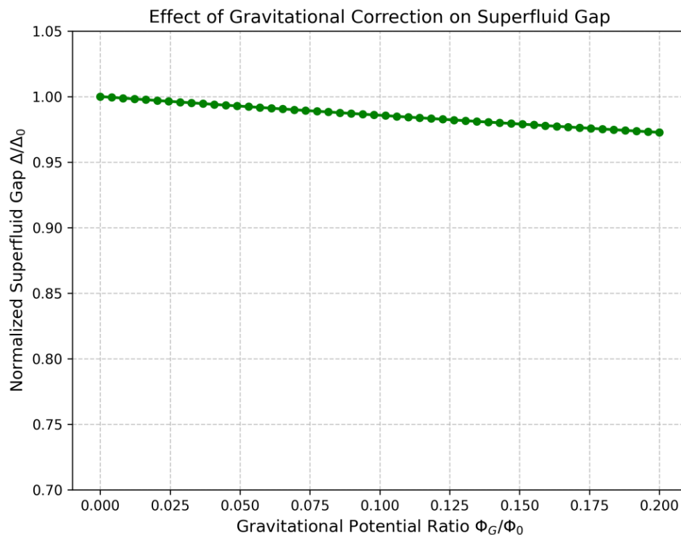
Figure 2. The influence of gravitational correction \Phi_G\Delta/\Delta_0 on the energy gap distribution curve, with the horizontal axis as and the vertical axis as.
