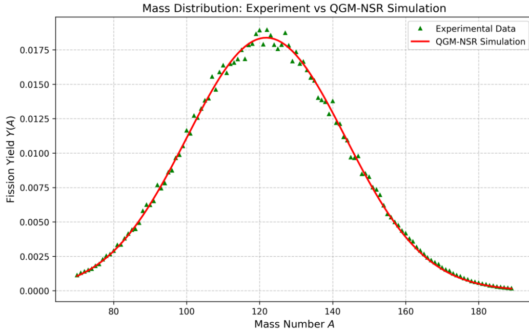
Figure 10. The comparison of the quality distribution curves between the experimental value and the simulated value shows that the two curves almost coincide.
