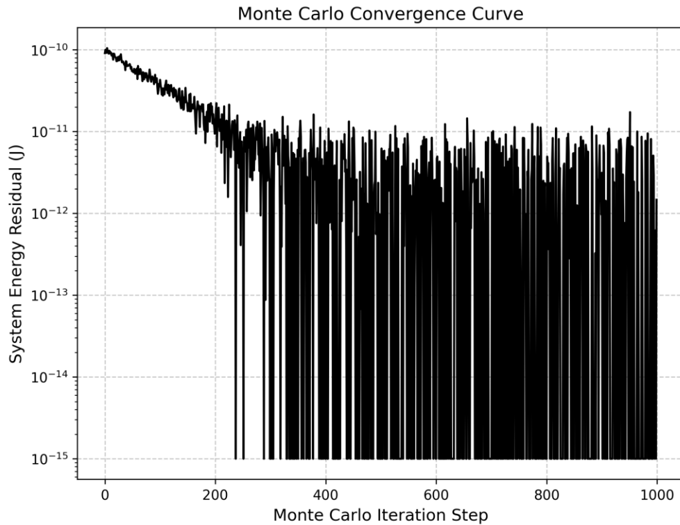
Figure 3. Monte Carlo convergence curve, with the number of iterations on the x-axis and the energy residual of the system on the y-axis.
