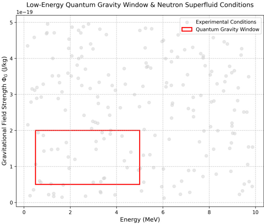
Figure 14. Schematic diagram of the intersection region between low energy quantum gravity window and neutron superconductivity experimental conditions.
