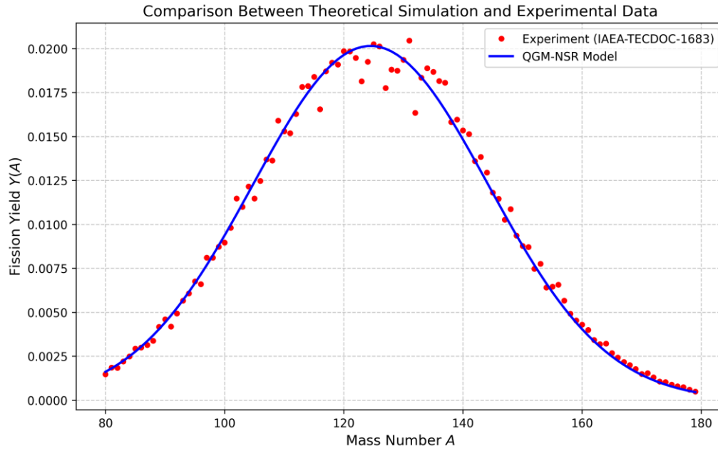
Figure 6. The comparison curve between theoretical simulation results and experimental data. The two curves should be highly coincident to show the accuracy of the model.
