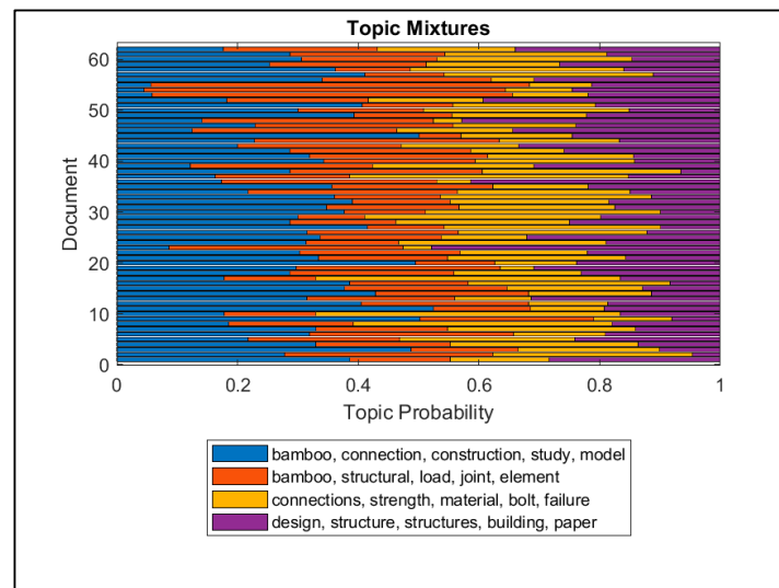
Figure 5. Topic mixtures.
