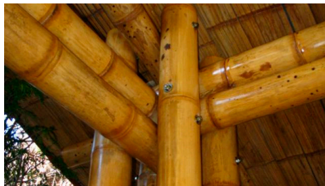
Figure 13. Bolted connections [72].
