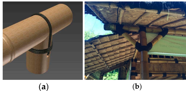
Figure 11. Lashing joints: (a) Notched and pierced with lashing [21]; (b) lashing joint using palm rope [71].
