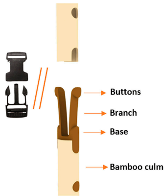
Figure 15. 3D printed removable connection [69].
