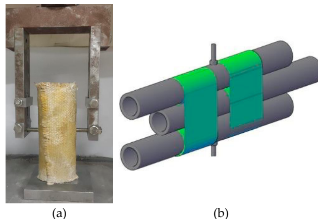
Figure 17. Combination of bolted connection and emerging technologies in bamboo connection: (a) Bolted connection wrapped in GFRP [74]; (b) Bolted connection wrapped in natural fiber “ijuk” [23].
