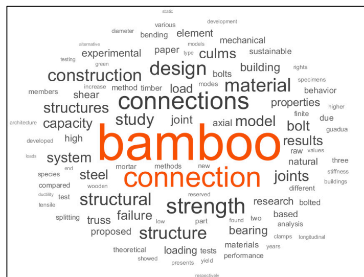
Figure 2. Word cloud.
