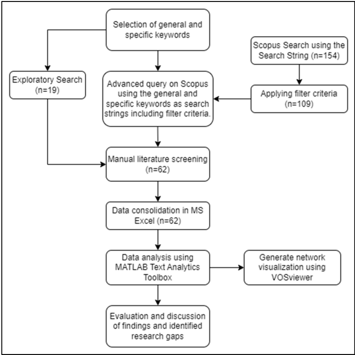
Figure 1. Methodology flowchart.
