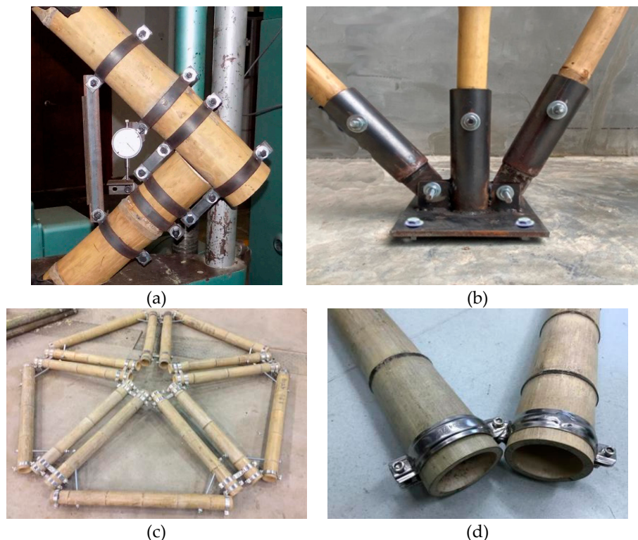
Figure 14. Clamped and capped connections: (a) Steel clamp [17]; (b) Pre-fabricated steel connector attached at the end of bamboo culm (capped connection) [44]; (c) Spatial structure of raw bamboo connected by BHC [76]; (d) Connected by steel hoops [76].
