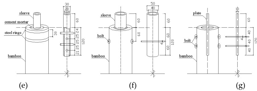
Figure 18. Combination of modern connections with supplementary connection components: (a) Parallel bolted mortar infill connection [49]; (b) Bamboo culms connected by wooden block (sleeve) and steel hose-clamp [66]; (c) Connected by wooden clamp, wooden gusset plate and steel bolts [16]; (d) Connected by bamboo sleeve and nails [68]; (e) Sleeve-cement connection [67]; (f) Sleeve-bolt connection [67]; (g) Groove-plate connection [67].
