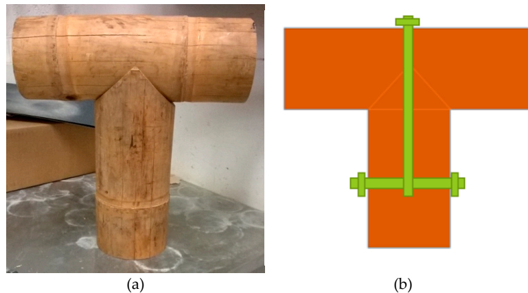
Figure 16. Combination of fish-mouth and bolted connection: (a) Fish-mouth T-connection without the bolts [51]; (b) Schematic view including bolts [51].
