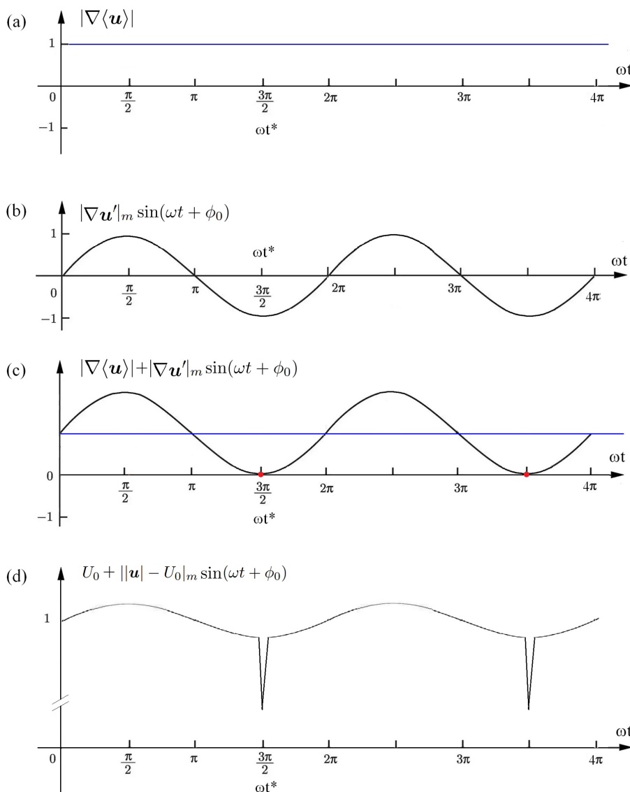
Figure 3. Schematic of appearance of velocity discontinuity (spike) at the position of x_0 and the phase angle \omega t^* . All the variables at the ordinate are normalized, \phi_0 is the initial phase angle, and the subscript m represents the amplitude. (a) The mean velocity gradient; (b) The disturbance velocity gradient; (c) The instantaneous velocity gradient; (d) The instantaneous velocity. Note: In the evolution of flow from the initial flow state to the formation of velocity discontinuity, we take two periods of phase angle variation near the critical time t^* of singularity at x_0 , which is shown in this figure. The phase angle \omega t^* = 3\pi/2 in the figure is the first appearance of the velocity discontinuity. For all 0 \leq t < t^* , \|\nabla \mathbf{u}(x_0, t^*)\|_{L^2(\psi)} > 0 ; At t = t^* , \|\nabla \mathbf{u}(x_0, t^*)\|_{L^2(\psi)} = 0 for the first time, as accessed by the Poincaré inequality Equation (15).
