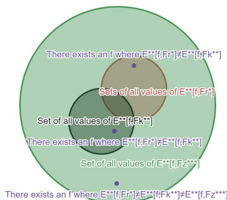
Figure 1. Below F_r^\star, F_k^{\star\star}, F_z^{\star\star\star} are non-equivalent starred sequences of sets, where V' is all circles and E^{**} is the generalized expected value of f w.r.t either \star -sequence of sets (def. 8)
