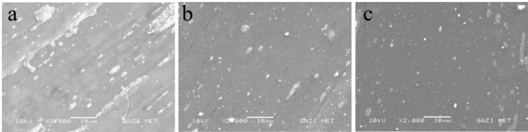
Figure 3. SEM micrographs of PMMA and nanocomposites: (a) PMMA, (b) PMMA-6, (c) PMMA-12.
