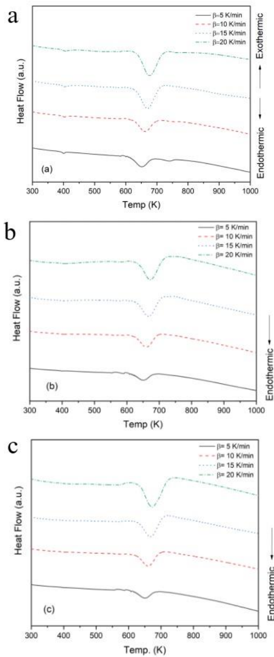
Figure 4. DTA graphics of the samples (a) PMMA, (b) PMMA-6 and (c) PMMA-12.
