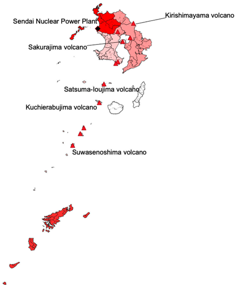
Figure 1. Relationship between response rate and geographic information Diamond symbol: Sendai Nuclear Power Plant, Triangle symbol: Volcano.
