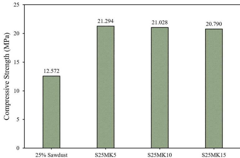
Figure 6. Compressive Strength of Concrete Samples with Varying Metakaolin Content (25% Sawdust).
