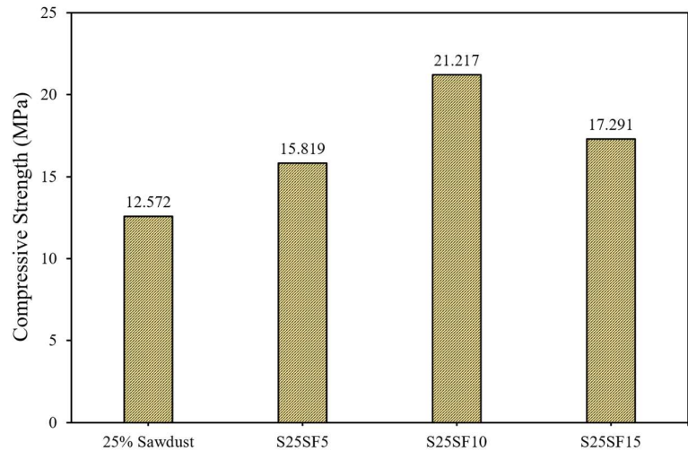
Figure 5. Compressive Strength of Concrete Samples with Varying Silica Fume Content (25% Sawdust).
