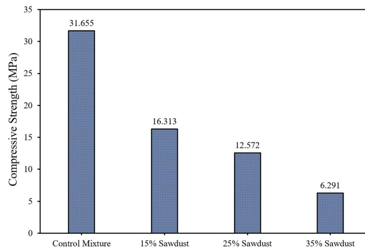
Figure 4. Compressive Strength of Concrete Samples with Varying Sawdust Content.
