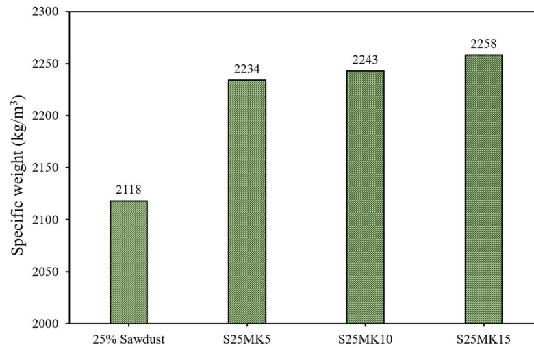
Figure 10. Density of Concrete Samples with Varying Metakaolin Content (25% Sawdust).
