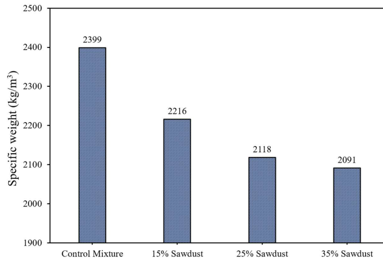
Figure 8. Density of Concrete Samples with Varying Sawdust Content.
