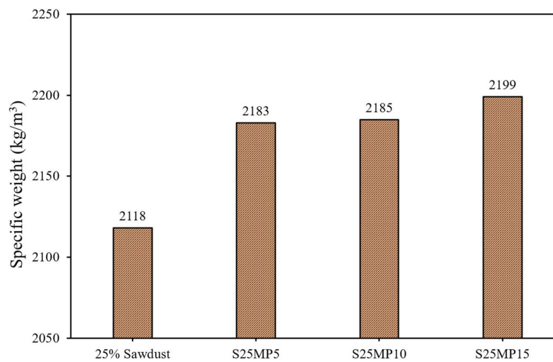
Figure 11. Density of Concrete Samples with Varying Marble Powder Content (25% Sawdust).
