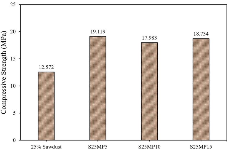
Figure 7. Compressive Strength of Concrete Samples with Varying Marble Powder Content (25% Sawdust).
