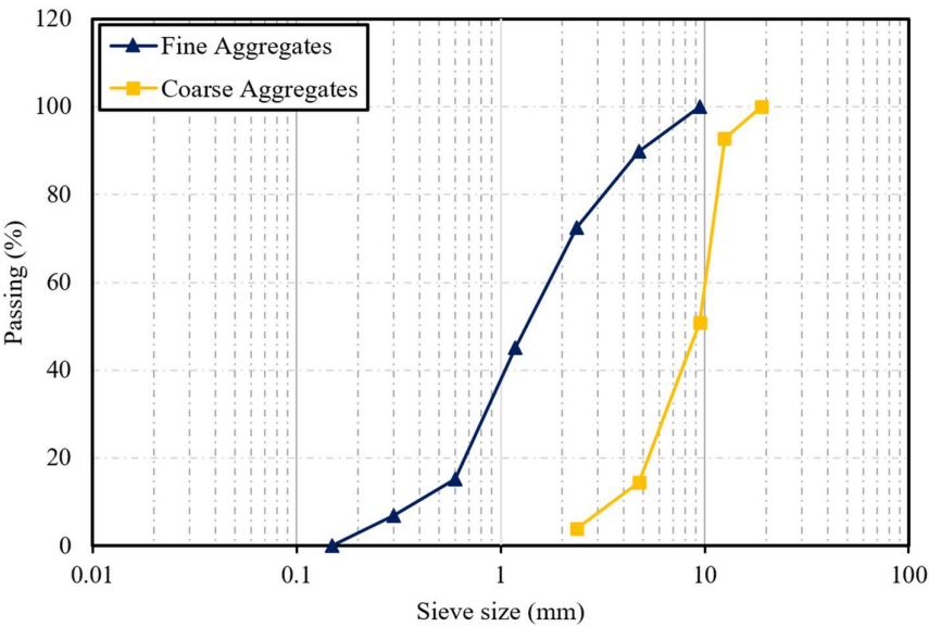
Figure 1. Distribution of particle sizes in fine and coarse aggregates.
