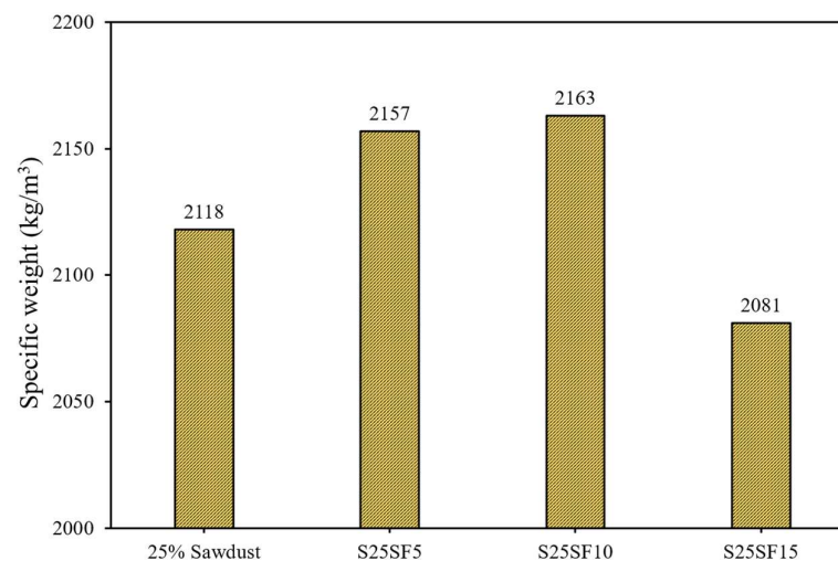
Figure 9. Density of Concrete Samples with Varying Silica Fume Content (25% Sawdust).
