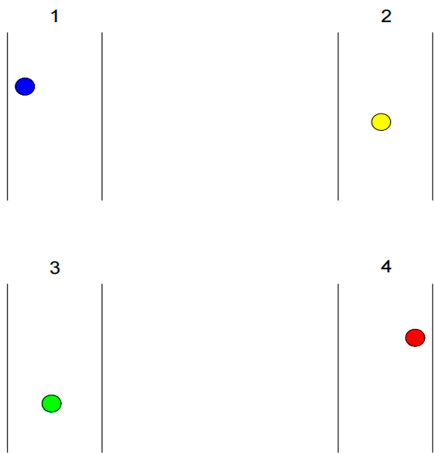
Figure 5. Two-slit interference experiment.
