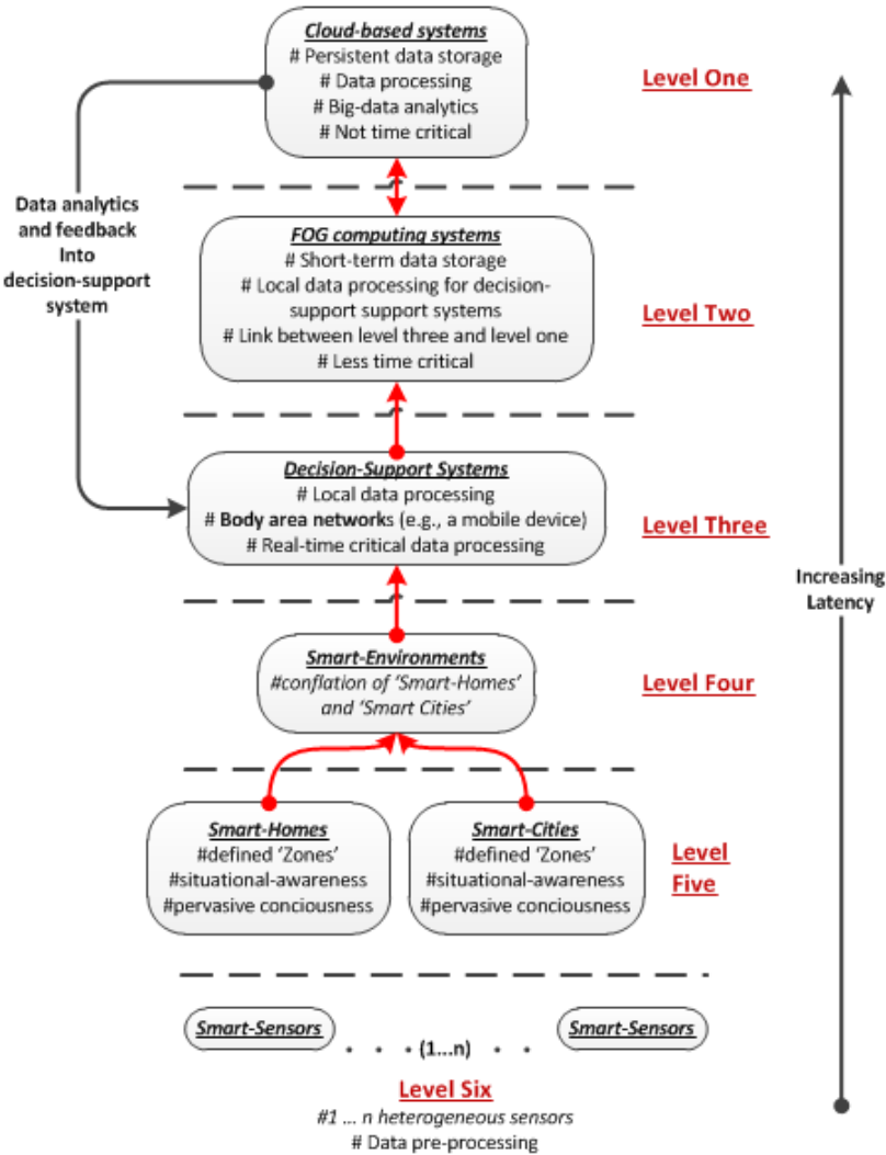
Figure 4. The Fog Computing Model (FCM): is a conceptual model showing the architectural relationships between heterogeneous ‘smart-sensors’, the ‘smart-home’ with data processing in a BAN, fog computing systems, and cloud-based systems. The model shows the deployment of a homogeneous system comprising data capture, computing, storage, and networking components along with decision-support systems. Source [34].
