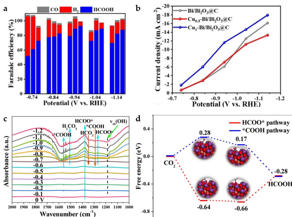
Figure 16. (a) FE of H 2 , CO, HCOOH for Cu x -Bi/Bi 2 O 3 @C (x = 0, 0.5, 1). (b) Partial current density of HCOOH of different catalysts [16]. Copyright 2022, Wiley-VCH. (c) The in situ FT-IR spectra on CuBi75 catalyst at different applied potential from 0 V to -1.2 V. (d) The free energy diagrams of different pathway for CO 2 electroreduction to HCOOH on CuBi75 (211) plane [51]. Copyright 2021, Elsevier.
