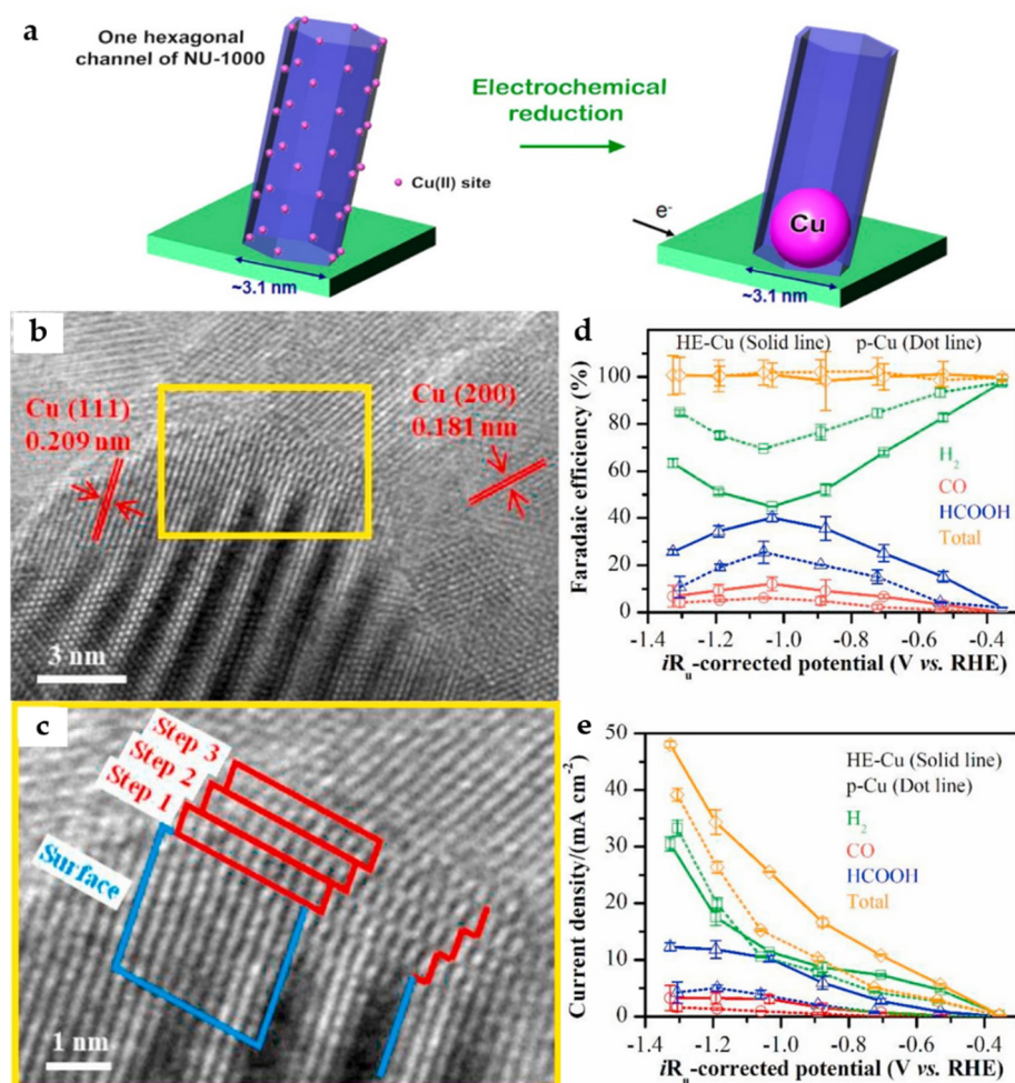
Figure 9. (a) Schematic representation of the electrochemical reduction of Cu 2+ to generate metallic Cu NPs [36]. Copyright 2017, ACS. (b) The HRTEM images of the HE-Cu and (c) stepped Cu (211) surface of the selected area. (d) Faradaic efficiency and (e) current density of the ECO 2 RR products for the HE-Cu and p-Cu electrodes in CO 2 -saturated 0.1 M KHCO 3 solution [37]. Copyright 2021, Elsevier.
