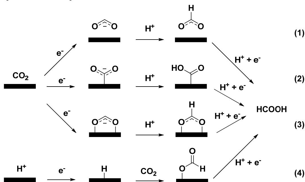
Figure 1. Proposed reaction pathways of \text{ECO}_2\text{RR} to \text{HCOOH} .
