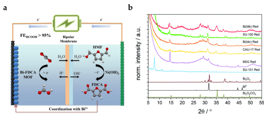
Figure 6. (a) Diagrammatic sketch for coupling system of ECO 2 RR in cathode and oxidation reaction of HMF in anode [31]. Copyright 2022, Wiley-VCH. (b) Grazing incidence XRD data collected using Co Kα radiation ( \lambda = 1.79 \text{ \AA} ) on coordination polymers (CPs) deposited on glassy carbon electrodes after reduction for 30 min at -0.97 V. The diffraction patterns are compared with calculated patterns for Bi 2 O 3 , Bi, and Bi 2 O 2 CO 3 [32]. Copyright 2021, RSC.
