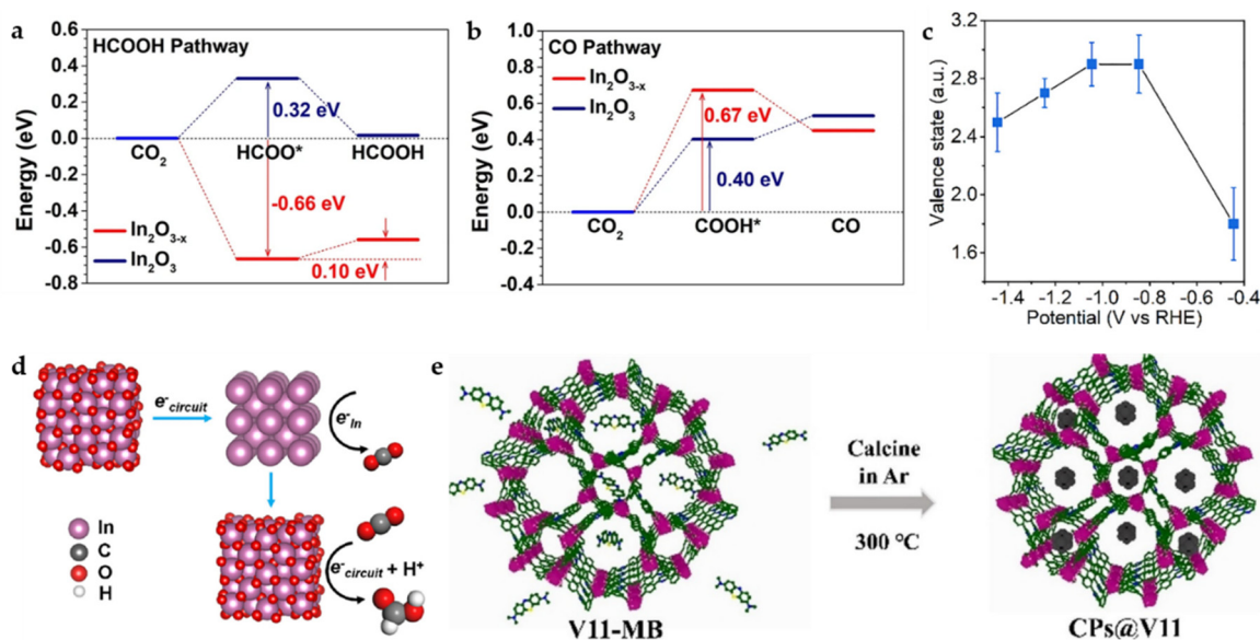
Figure 14. (a) Free energy diagrams for \text{CO}_2 electroreduction to \text{HCOOH} and (b) \text{CO} on \text{In}_2\text{O}_3 and \text{In}_2\text{O}_{3-x} . (c) Changes of In valence state in MIL-68- \text{N}_2 under different applied potentials, which are examined by using the K-edge energy shift with respect to the commercial \text{In}_2\text{O}_3 sample. (d) The proposed reaction mechanism based on the operando measurements [47]. Copyright 2022, Springer Nature. (e) Illustration of the preparation process of \text{CPs@V11} [48]. Copyright 2021, Wiley-VCH.
