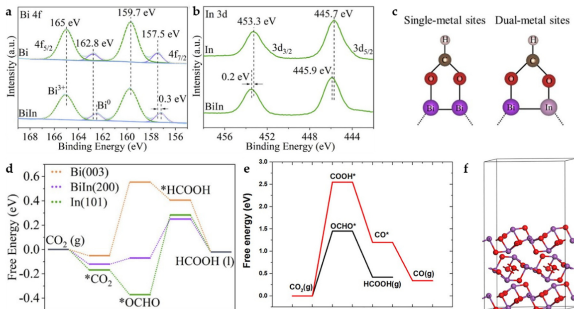
Figure 17. (a) Bi 4f XPS spectra of Bi-In alloy NPs and Bi NPs. (b) In 3d XPS spectra of Bi-In alloy NPs, and In NPs. (c) ^*\text{OCHO} adsorption in single-metal (left) and dual-metal (right) catalytic systems through side-on configurations. (d) Calculated free energy diagrams for \text{CO}_2 electroreduction to \text{HCOOH} on Bi (003), BiIn (200), and In (101) [52]. Copyright 2022, Elsevier. (e) Free energy diagrams for \text{CO}_2 electroreduction to \text{HCOOH} and \text{CO} on \text{Bi}_2\text{O}_3(010) . (f) Optimized structures of \text{Bi}_2\text{O}_3(010) [53]. Copyright 2021, Elsevier.
