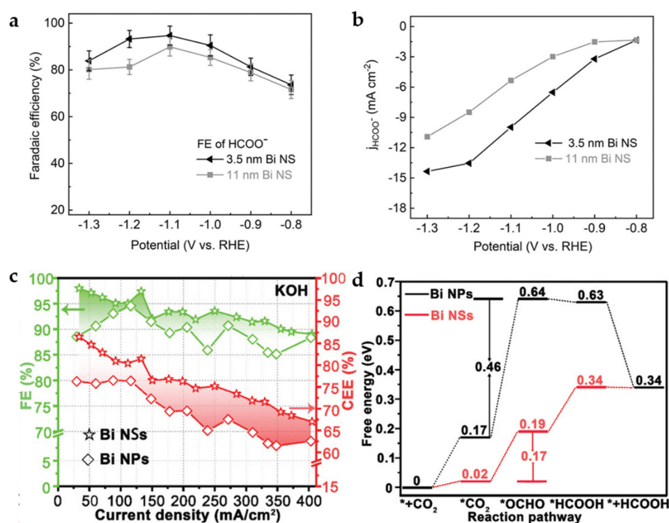
Figure 10. (a) \text{FE}_{\text{HCOO}^-} of 3.5 nm and 11 nm Bi NSs in \text{CO}_2 -saturated 0.1 M \text{KHCO}_3 . (b) Partial current densities for \text{HCOO}^- of 3.5 nm and 11 nm Bi NSs [38]. Copyright 2021, Wiley-VCH. (c) FEs and CEEs for HCOOH of Bi NPs and Bi NSs in 1 M KOH. (d) Gibbs free energy diagrams for \text{CO}_2 electroreduction to HCOOH on Bi NPs and Bi NSs [39]. Copyright 2020, Wiley-VCH.
