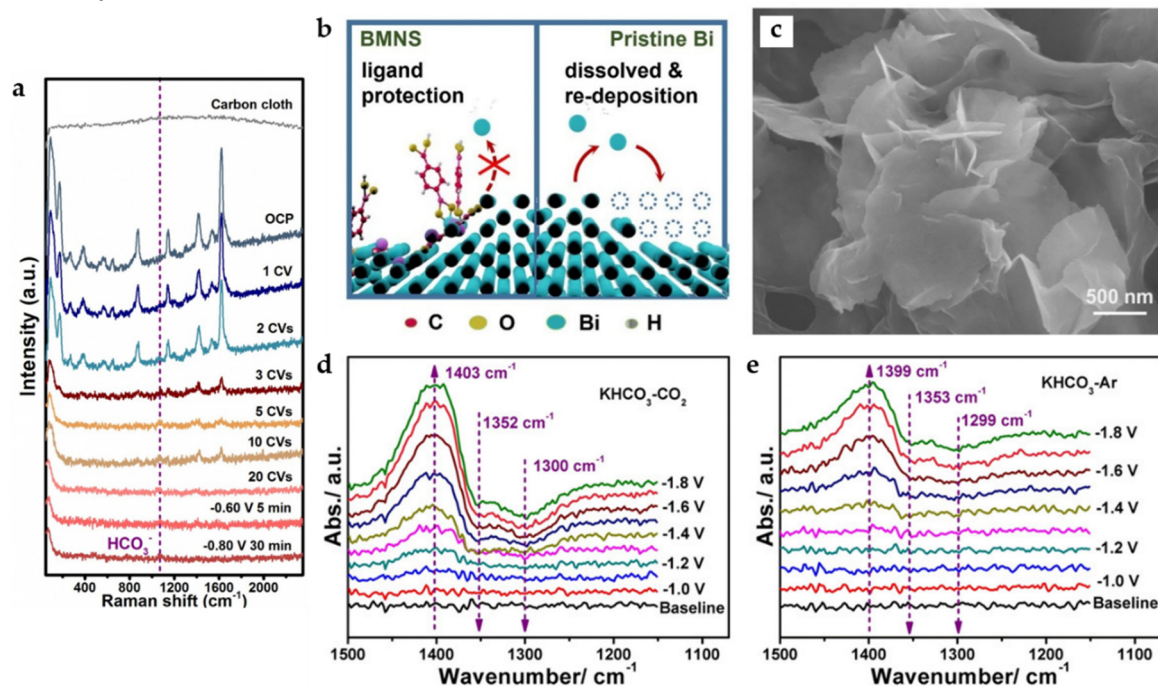
Figure 11. (a) In situ Raman spectra for showing the transformation from Bi-MOF to BMNS. (b) Proposed mechanism of action for ligands adsorbed on the surface of BiMNS preventing the deactivation of active sites [41]. Copyright 2021, Elsevier. (c) Scanning electron microscopy (SEM) images of Bi-ene. In situ ATR-IR spectra collected under different applied potentials in (d) \text{CO}_2 and (e) Ar-saturated 0.5 \text{ M KHCO}_3 (all applied potentials are vs. Ag/AgCl in this part) [42]. Copyright 2020, Wiley-VCH.
