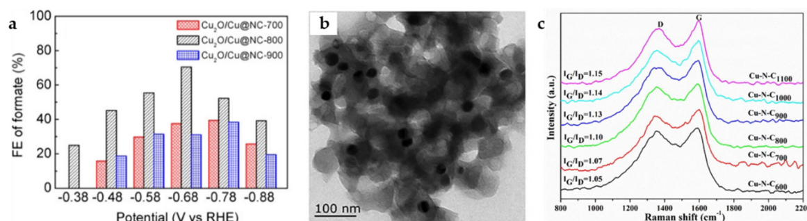
Figure 12. (a) FE_{HCOO^-} for ECO 2 RR of Cu 2 O/Cu@NC-700, Cu 2 O/Cu@NC-800, and Cu 2 O/Cu@NC-900 [23]. Copyright 2020, ACS. (b) TEM image for Cu-N-C 1100 . (c) Raman spectra of Cu-N-C r composite catalyst [45]. Copyright 2021, Elsevier.
