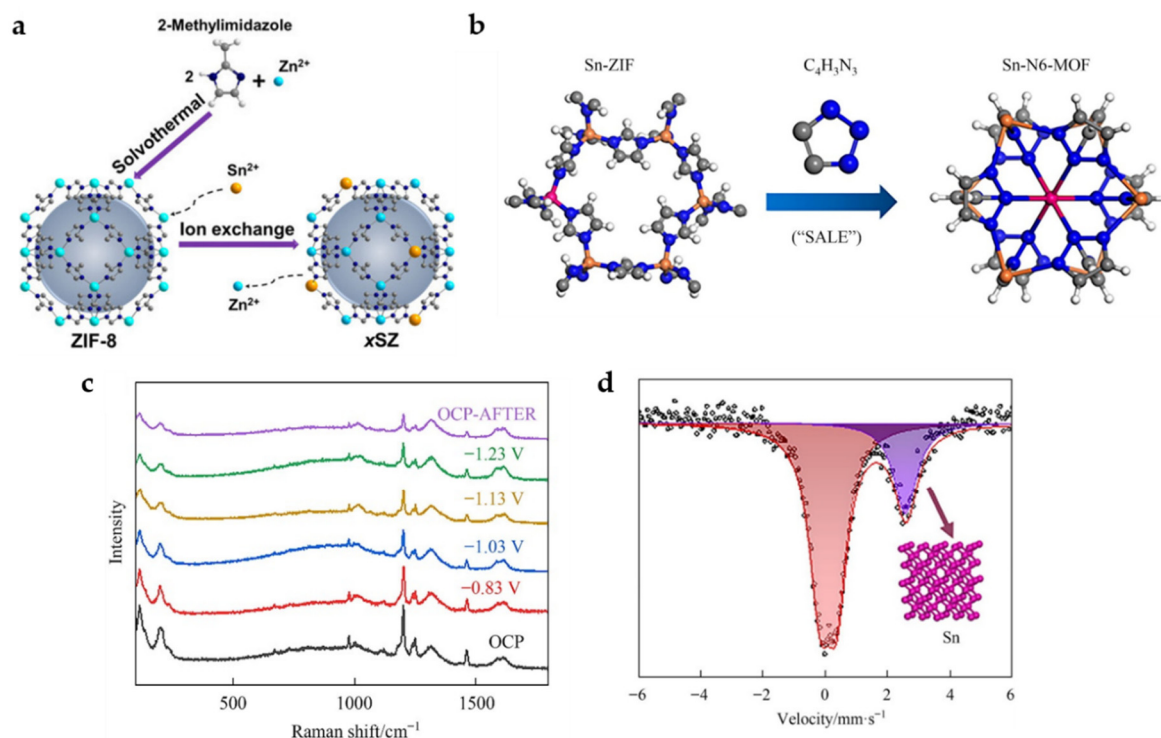
Figure 8. (a) Schematic illustration showing the preparation of Sn-doped ZIF-8 catalysts [17]. Copyright 2020, Wiley-VCH. (b) Diagram of the synthetic procedures for Sn-N6-MOF. (c) The in-situ Raman spectra measured with varying the applied potential at -1.23 V in CO 2 -saturated 0.5 M KHCO 3 electrolyte. (d) Room temperature 119 Sn Mössbauer spectra acquired after maintained at -1.23 V in CO 2 -saturated 0.5 M KHCO 3 electrolyte for 1 h [34]. Copyright 2022, Elsevier.
