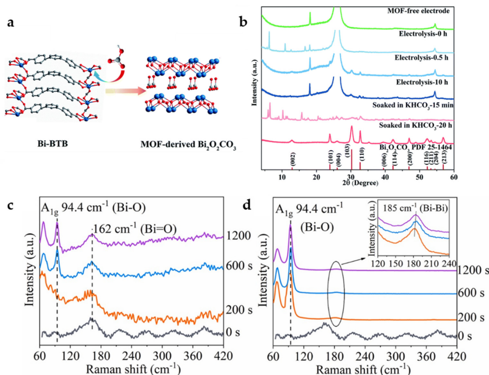
Figure 4. (a) Proposed mechanism for the formation of MOF-derived \text{Bi}_2\text{O}_2\text{CO}_3 . (b) XRD patterns of carbon paper electrode (green), Bi-BTB/carbon paper electrode before electrolysis (sky blue), after 0.5 h electrolysis (steel blue) and after 10 h electrolysis (dark blue), and Bi-BTB soaked in \text{KHCO}_3 after 15 min (salmon) and after 20 h (firebrick) [29]. Copyright 2020, RSC. In situ Raman spectra of Bi-BTC during the catalytic process under various potentials: (c) -0.5 \text{ V} and (d) -0.7 \text{ V} at 0.1 \text{ M KHCO}_3 [30]. Copyright 2022, Elsevier.
