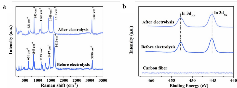
Figure 7. (a) Raman spectra of the In-BDC catalyst before and after electrolysis. (b) In 3d XPS spectra of the In-BDC catalyst before and after electrolysis [33]. Copyright 2020, ACS.
