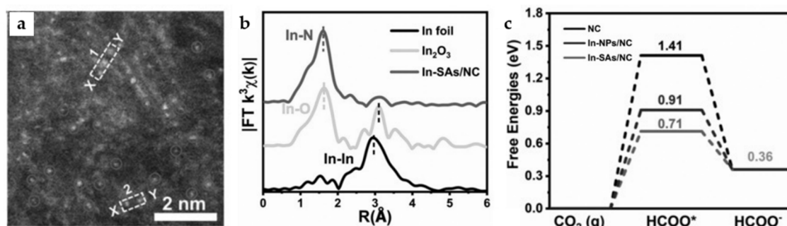
Figure 15. (a) High angle annular dark-field scanning transmission electron microscope (HAADF-STEM) image of In-SAs/NC. (b) In K-edge FT-EXAFS spectrum of In-SAs/NC. (c) The calculated potential free-energy diagrams for CO 2 electroreduction to formate [49]. Copyright 2022, Wiley-VCH.
