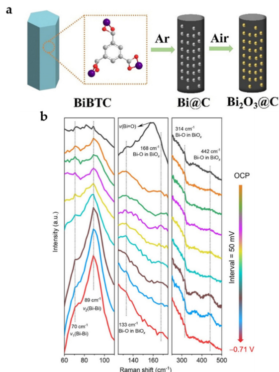
Figure 13. (a) Preparation of Bi@C and Bi 2 O 3 @C catalysts [25]. Copyright 2020, Wiley-VCH. (b) In situ Raman spectra of the (surface-oxygen-rich) SOR Bi@C NPs catalyst as a function of the applied potential in 1.0 M KOH electrolyte at various potentials [46]. Copyright 2022, ACS.
