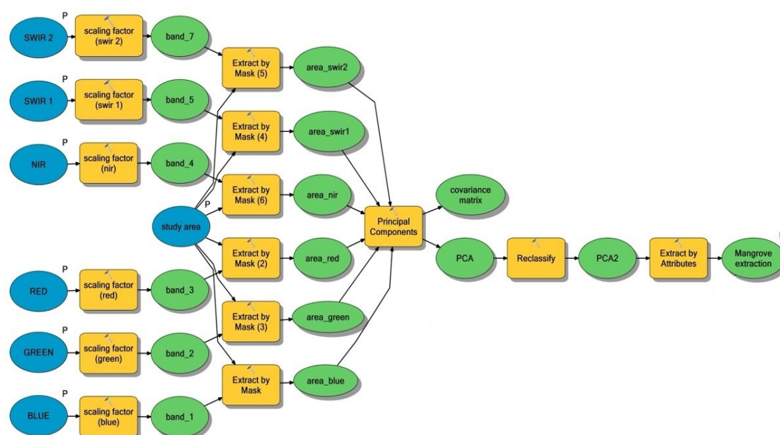
Figure 2. Automation model for extraction of mangrove cover and corresponding LST values. Blue ovals have a P superscript indicating that users only have to load the spectral bands of their site of interest. Yellow squares are geospatial processes and green ovals are the result of each geoprocess.
