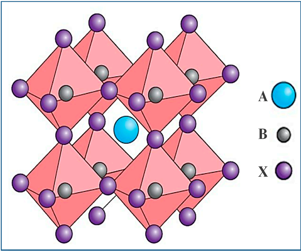
Figure 1. Model of the ideal crystal structure of perovskite ABX_3 .
