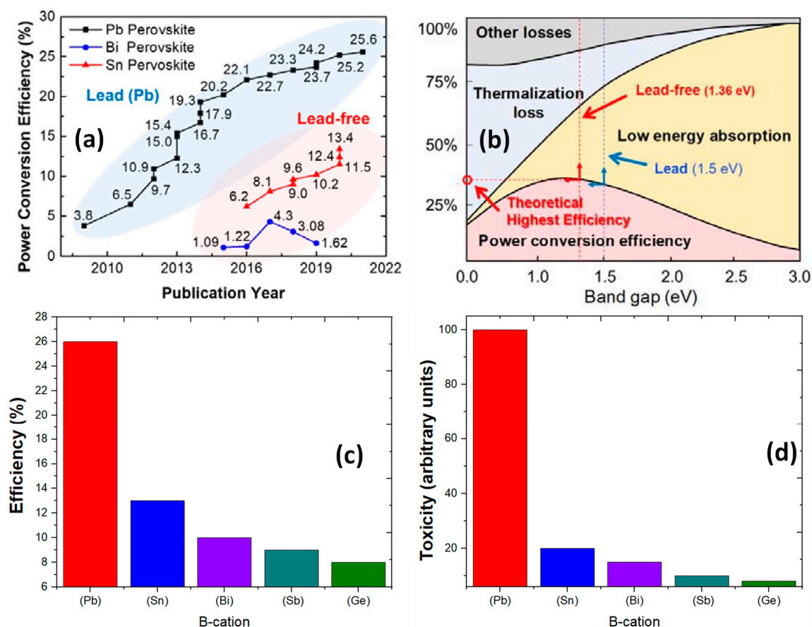
Figure 4. Comparison of efficiencies and other key characteristics of lead-based and lead-free solar cells: (a) Reported PCEs of Pb-based, Bi-based, and Sn-based PSCs from the initial stage of development to date [44]; (b) Shockley–Queisser limit graph showing the PSC type that has a relatively high ideal bandgap [55]; (c) Growth chart of PCEs based on lead and lead-free perovskites [30,39,41,42,45,53,55–57]; (d) Comparative toxicity levels of elements used in perovskites [41,45,50,52–54]. .
