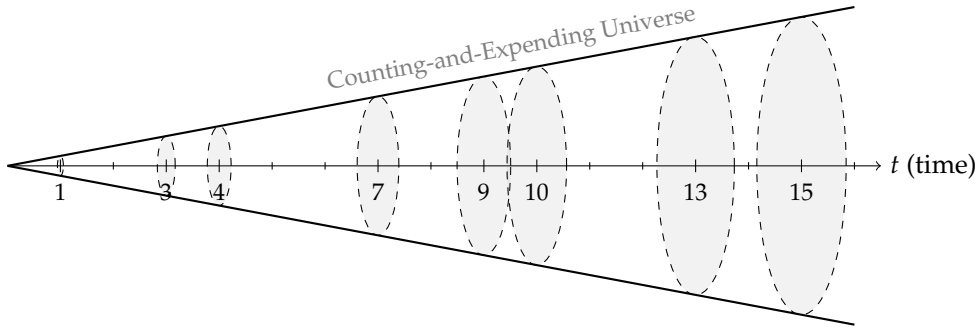
Figure 1. Schematic of the first 16 counts of the counting universe cone of radius t and cardinality q = 4t + 1 . The gray circles indicate the “reset” events, when the cardinality q is prime thus degenerating the underlying mathematical construct to a field \mathbb{F}_p and the corresponding universe morphology from a 3D manifold to an S^2 spheroid.
