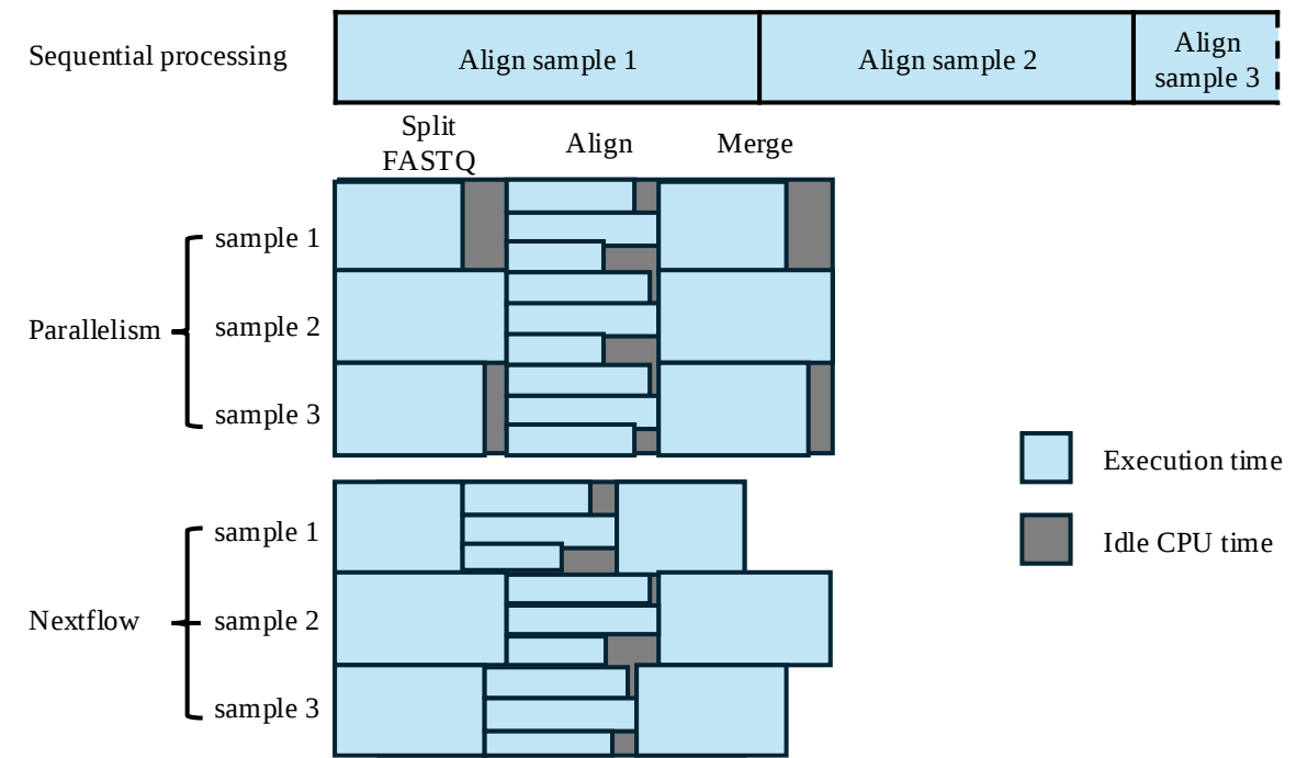
Figure 4. Schematic comparisons of African data processing in the alignment step using sequential processing, simple parallelisation and automated workflow.
