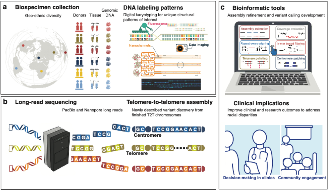
Figure 5. Overarching schematic of cancer genomics with a focus on diversity and inclusion. a Starting with the global collection of biospecimens chosen with unique patterns of digital karyotyping as exemplified by Chan et al [68]. b an innovative reference-free cancer genomics pipeline can be built based on the foundation of long-read technologies and telomere-to-telomere assembled chromosomes, followed by c a new ecosystem of analysis tools for their use in clinical applications.
