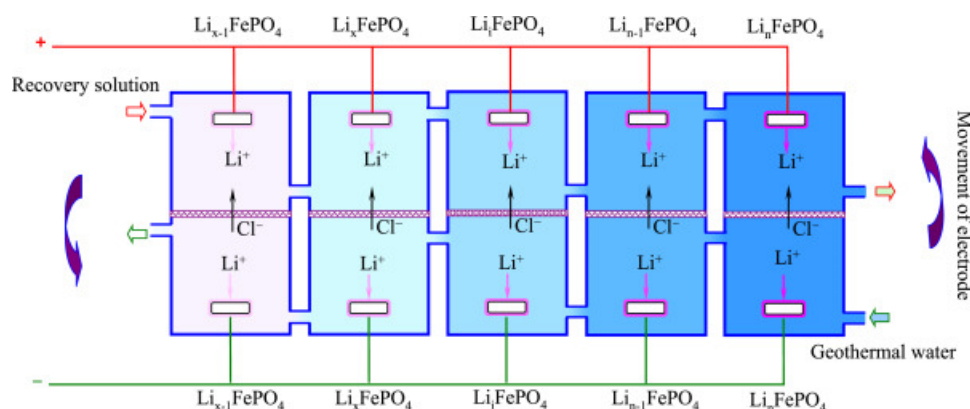
Figure 2. The schematic diagram of continuous electrochemical device proposed for \text{Li}^+ recovery from geothermal water [30].
