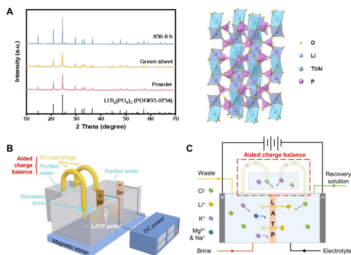
Figure 9. (A) XRD pattern and the crystal structure of LATP, and the schematic illustration of (B) LES and (C) the extraction process [49].
