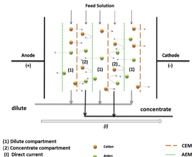
Figure 6. The schematic of electrodialysis [45].
