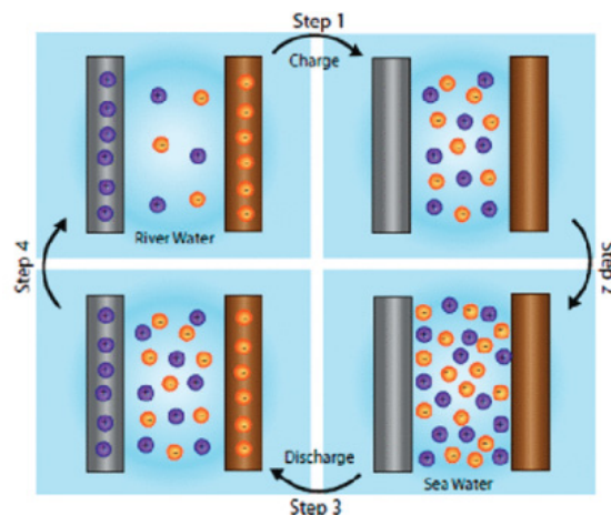
Figure 3. The schematic diagram of electrochemical extraction lithium by ion pump [33].
