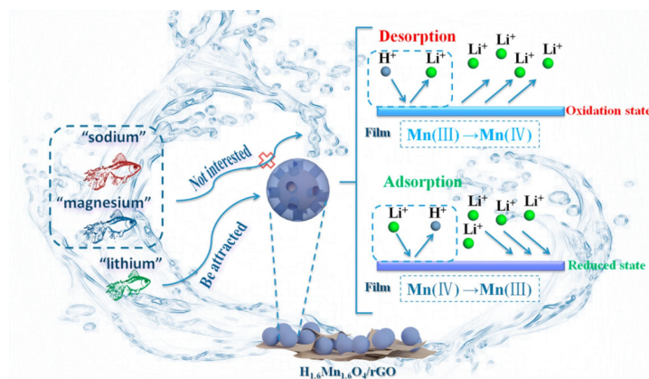
Figure 7. Schematic of the adsorption and desorption on the \text{H}_{1.6}\text{Mn}_{1.6}\text{O}_4/\text{rGO} composite film [47].
