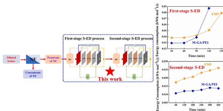
Figure 8. The configuration of the designed selective electro dialysis [48].
