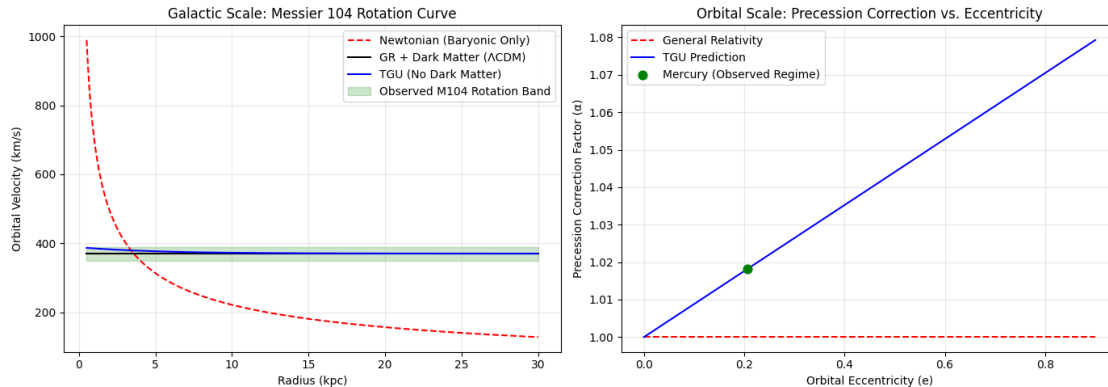
Figure 2. Cross-scale technical comparison between the Unified Theory of Informational Spin (TGU) and General Relativity. Left: Galactic rotation curve of Messier 104 showing that TGU reproduces the observed velocity plateau using baryonic matter only, without dark matter. Right: Orbital coherence correction factor \alpha as a function of eccentricity, illustrating convergence to GR at low eccentricity and predictive deviations in high-eccentricity systems.
