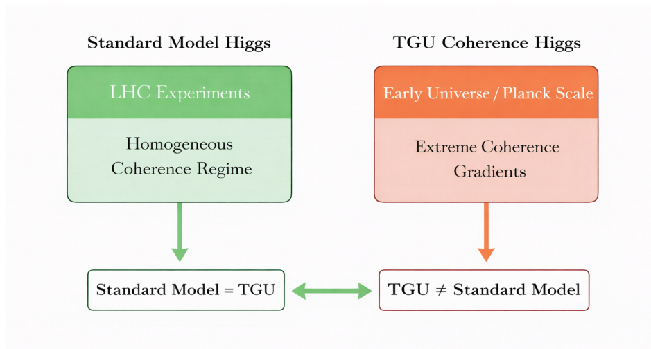
Figure 3: Regime map illustrating the domains of equivalence and deviation between the Standard Model Higgs mechanism and the TGU coherence-based formulation. Collider experiments operate deeply within the homogeneous coherence regime, while coherence-induced deviations are predicted only
