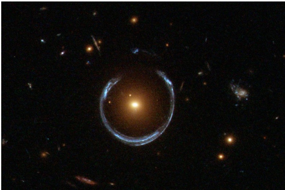
Figure 4. Comparative Analysis. (a) Hubble Space Telescope observation of LRG 3-757. (b) TGU synthetic reconstruction using only two parameters. The morphology of the deflection demonstrates that coherence-based geodetic deviation is indistinguishable from mass-induced curvature in the optical regime.
