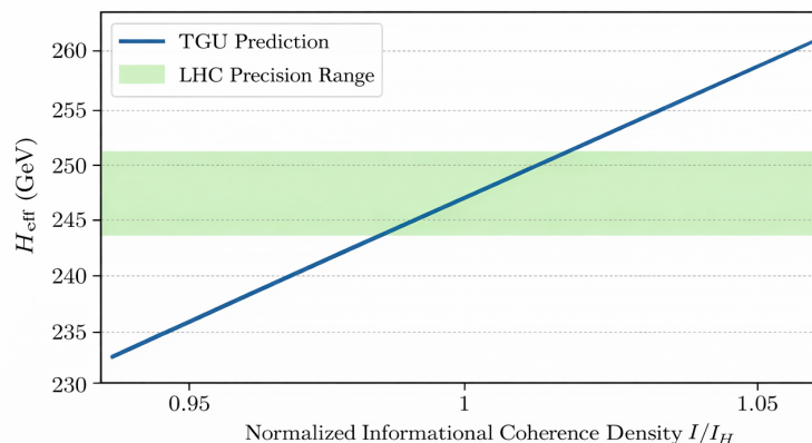
Figure 1: Effective Higgs parameter H_{\text{eff}} as a function of normalized informational coherence density I/I_H in the TGU framework. In the regime I/I_H \approx 1 , corresponding collider environments, H_{\text{eff}} remains effectively constant within current experimental precision. The shaded band indicates the sensitivity range of ATLAS and CMS measurements, showing exact overlap with the Standard Model expectation.
