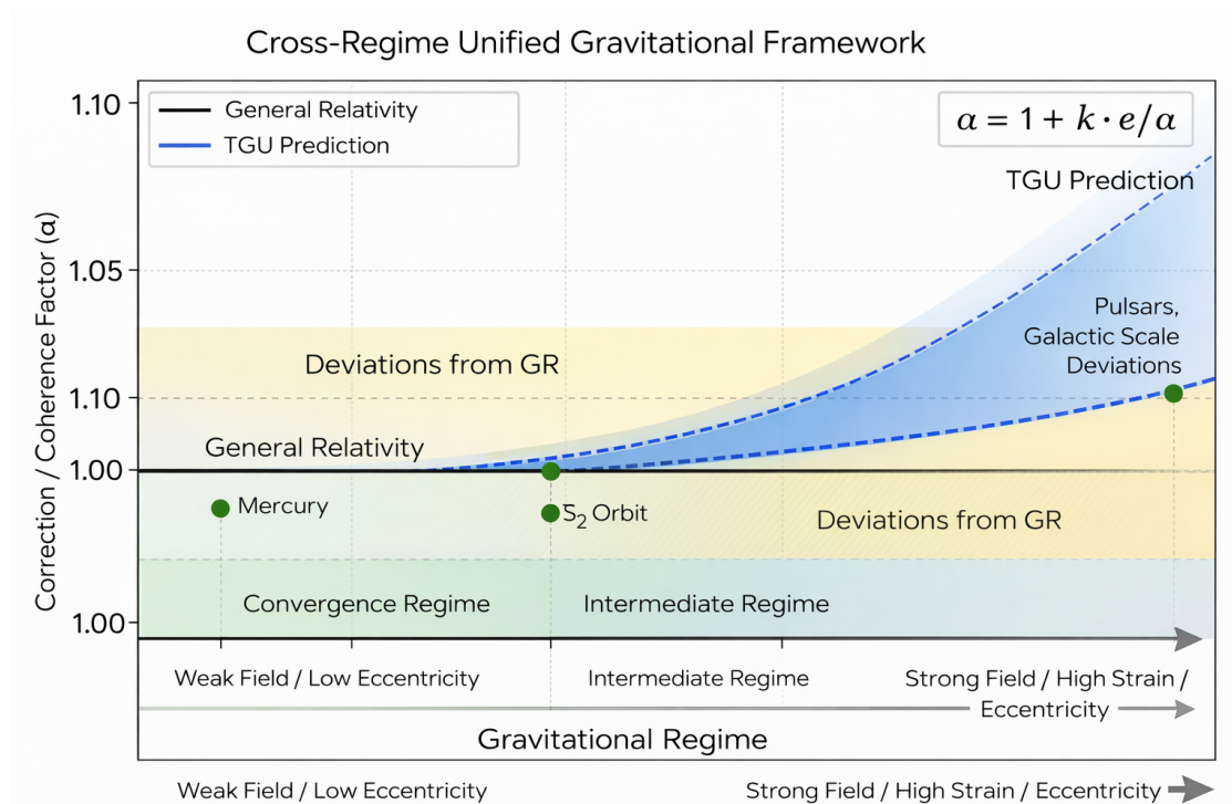
Figure 1. Cross-regime conceptual comparison between General Relativity and the Unified Theory of Informational Spin (TGU). The diagram illustrates how General Relativity (GR) provides accurate descriptions in weak- and intermediate-field regimes but requires additional components such as dark matter and dark energy at galactic and cosmological scales. In contrast, TGU introduces a coherence-based formulation that converges to GR in low-strain regimes while naturally extending across orbital, galactic, and cosmological domains through informational coherence gradients, without invoking unseen matter components. General relativistic reference values from [Ref. 11].
