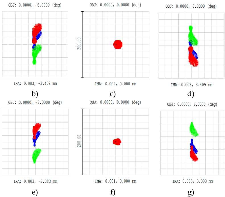
Figure 1. Galilean telescopes a) Zemax ray tracing. Spot diagrams fields b) and e) -6 degrees, c) and f) 0 degrees, and d) and g) 6 degrees, for glass and resin telescopes, respectively. Wavelengths: 486.1 nm (blue), 587.6 nm (green), and 656.3 nm (red).
