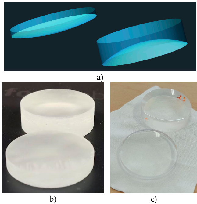
Figure 2. Design and fabrication. a) CAD design, b) Lens' curing, and c) Polished lens.
