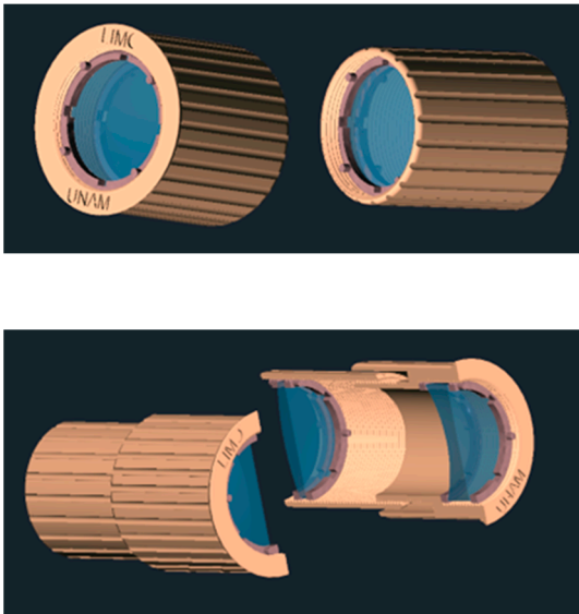
Figure 6. Telescope’s tube render.
