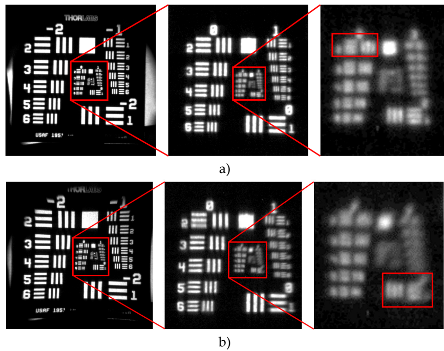
Figure 8. Telescopes' resolution analysis. a) BK-7 Glass lenses, and b) resin lenses.
