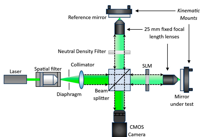
Figure 4. Roughness measurement in the Linnik interferometer.
