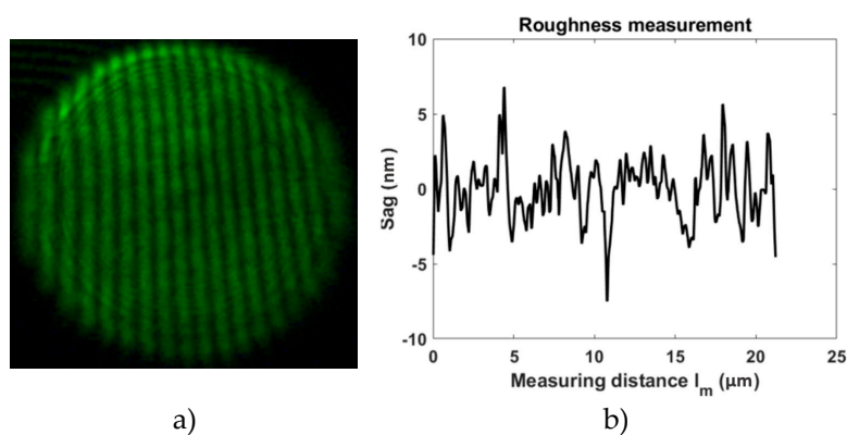
Figure 5. Roughness. a) Interferogram, and b) roughness profile.
