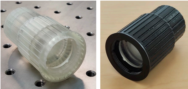
Figure 7. Low-Vision Galilean Telescope fabricated 100% with Clear resin.
