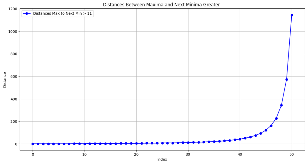
Figure 2. Distances between maxima and the following minima, greater than a given threshold.
