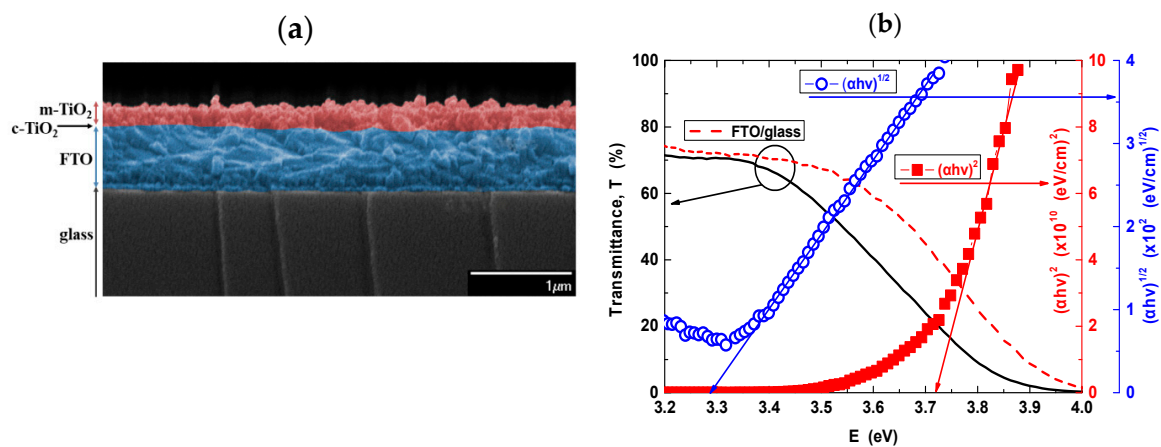
Figure 2. (a) SEM cross-sectional image of TiO 2 /FTO/glass. (b) UV-Vis-NIR transmittance of TiO 2 /FTO/glass (black solid line) and FTO/glass (red dash lines). The Tauc plots for determining the optical energy gap of effective TiO 2 are also shown in (b): blue open circles for indirect band gap ((αhν) 1/2 -vs-E) and red solid squares for direct band gap ((αhν) 2 -vs-E) analysis.
