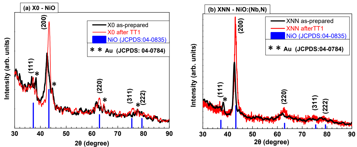
Figure 4. XRD graphs of (a) undoped NiO -X0 film and (b) doped NiO:(Nb,N) -XNN films deposited on glass substrates just after fabrication and after thermal treatment (TT1).
