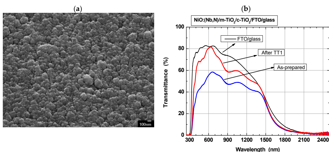
Figure 7. \text{NiO}:(\text{Nb},\text{N})/\text{TiO}_2 heterostructure: (a) Topography at 30^\circ tilted view and (b) UV-Vis-NIR transmittance before and after TT1, along with the transmittance of substrate (FTO/glass).
