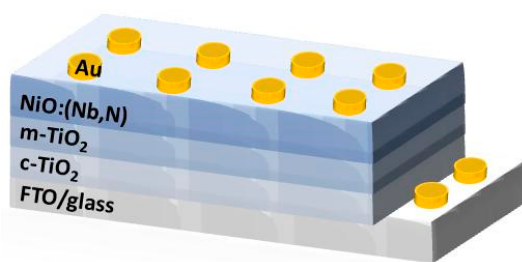
Figure 1. Schematic representation of the fabricated NiO:(Nb,N)/TiO 2 heterodiodes [NiO:(Nb,N)/m-TiO 2 /c-TiO 2 /FTO/glass]. Thicknesses are not to scale.
