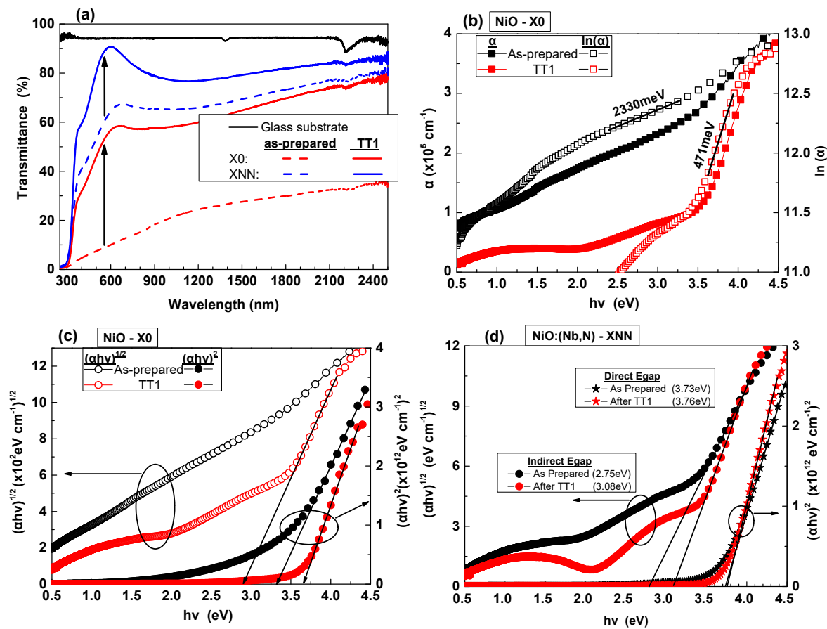
Figure 6. Optical properties of NiO –X0 and NiO:(Nb,N) –XNN films just after deposition and after thermal treatment (TT1): (a) UV-Vis-NIR transmittance of X0 and XNN films (the arrows indicate the increase of transmittance at \lambda = 550 nm after TT1). (b) Absorption coefficient, \alpha and \ln(\alpha) , and (c) Tauc plots of X0 film. (d) Tauc plots of XNN film.
