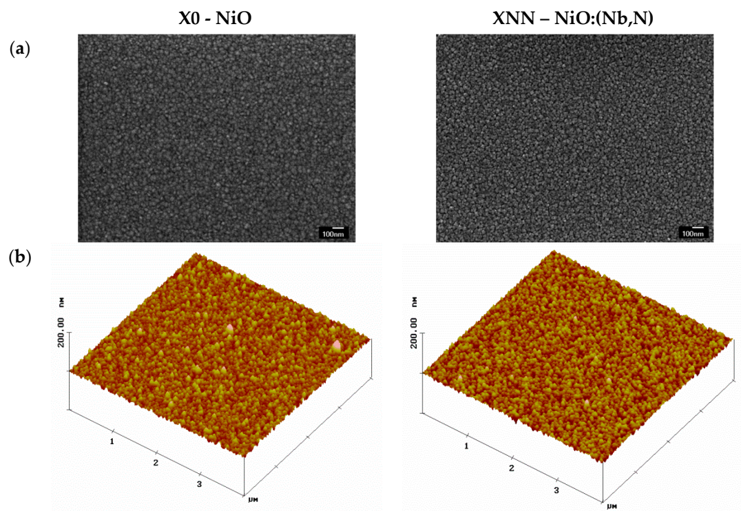
Figure 5. Topography on the same scale of undoped NiO and double-doped NiO:(Nb,N) films deposited on Si substrates: (a) SEM and (b) AFM images.
