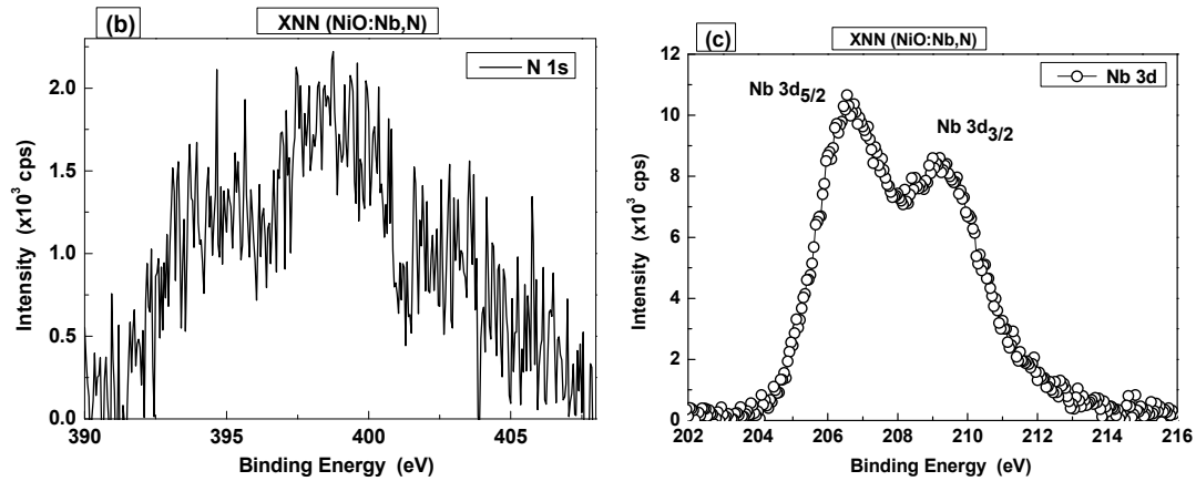
Figure 3. (a) Wide-scan XPS spectra of undoped NiO -X0 film and double-doped NiO:(Nb,N) -XNN film. (b) and (c) High-resolution N 1s and Nb 3d core levels spectra of double-doped NiO: (Nb,N) -XNN film, respectively.
