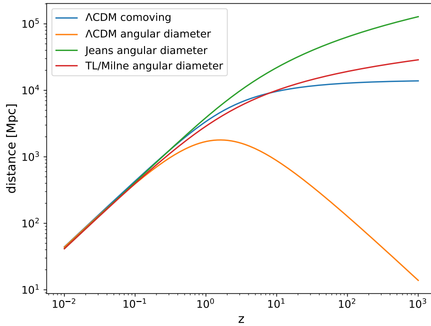
Figure 5. Redshift-distance relations for different cosmological models
