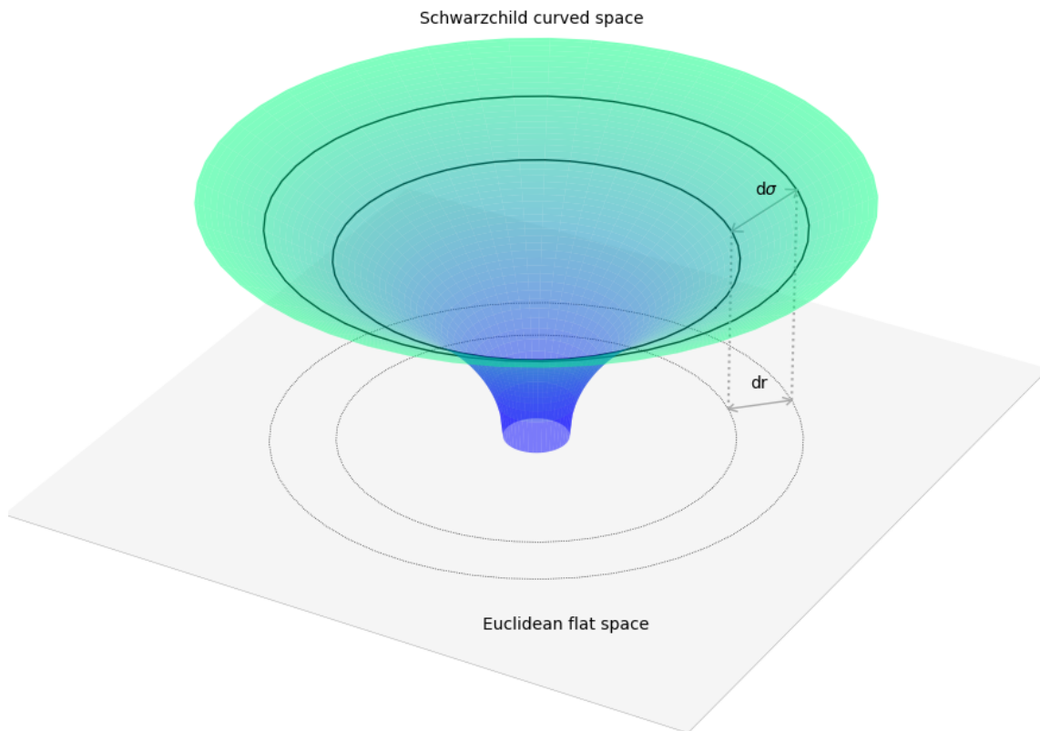
Figure 2. Schwarzschild metric
