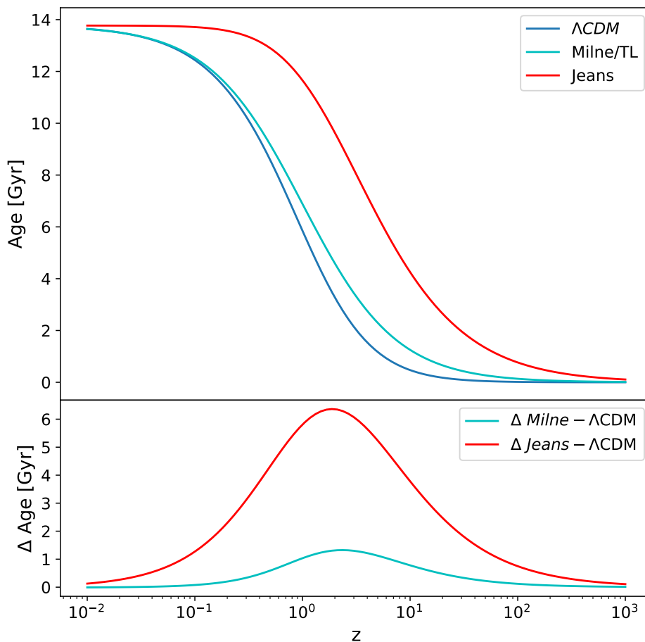
Figure 7. Age—redshift relation
