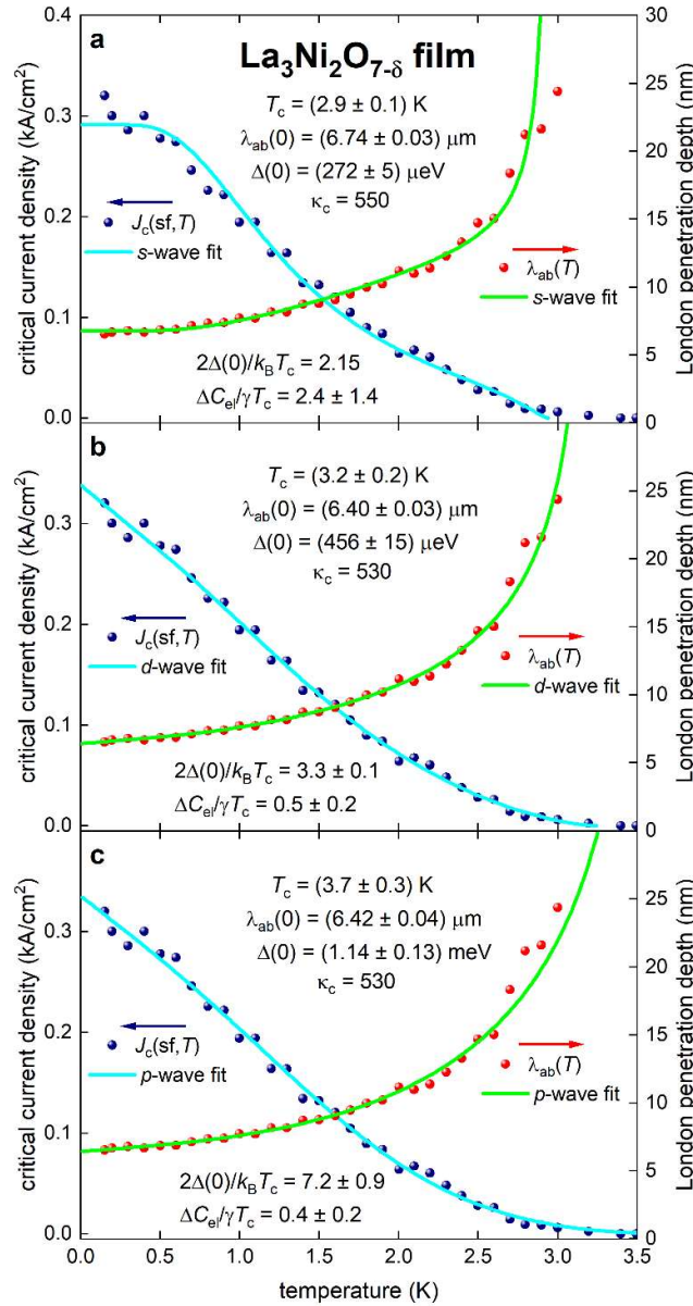
Figure 2. The self-field critical current density, J_c(sf, T) , for the ambient pressure \text{La}_3\text{Ni}_2\text{O}_{7-\delta} film 1 (reported by Ko et al 1 in their Figure 3,a 1 ) and data fit to the single band model (Eq. 16) with symmetry of (a) s -wave (Eqs. 17,18, fit quality R = 0.9575 ); (b) d -wave (Eqs. 18-20, fit quality R = 0.9810 ); and (c) polar \vec{A} \perp \vec{l} p -wave (Eqs. 22-25, fit quality R = 0.9849 ). Derived parameters are shown in each panel. \xi_{ab}(0) = 12 \text{ nm} was assumed for all fits.
