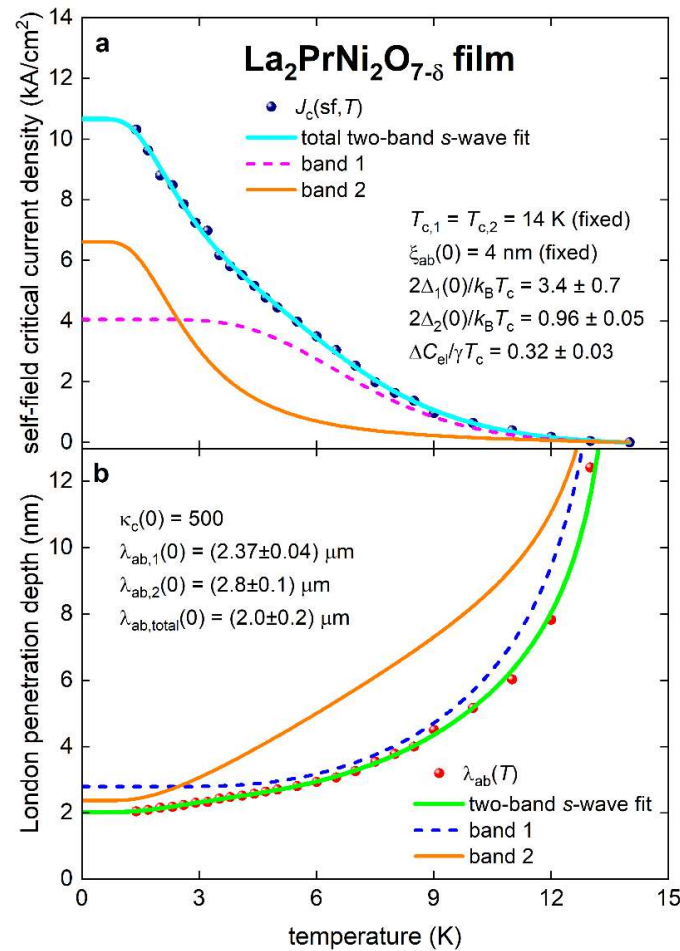
Figure 6. The self-field critical current density, J_c(sf, T) , in the ambient pressure \text{La}_2\text{PrNi}_2\text{O}_{7-\delta} film 3 (reported by Liu et al 3 in their Figure 1,b 3 ) and data fit to two-band ( s - + s -) wave model (Eq. 29). The assumptions are:
