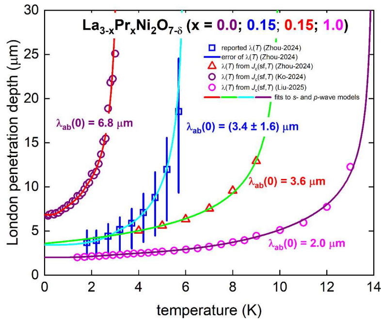
Figure 16. Derived London penetration depth, \lambda_{ab}(T) , for all ambient pressure \text{La}_{3-x}\text{Pr}_x\text{Ni}_2\text{O}_{7-\delta} ( x=0.0; 0.15; 1.0 ) thin films 1-3 studied in this work.
