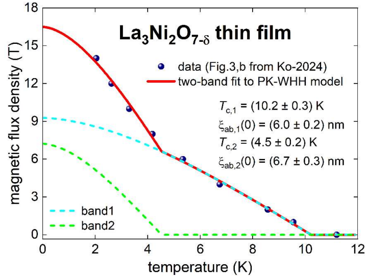
Figure 13. B_{c2}(T) data deduced from R(T, B) curves reported for the ambient pressure \text{La}_3\text{Ni}_2\text{O}_{7-\delta} film reported in Figure 3,b 1 by applying criteria of \frac{R(T=T_{c,0.29})}{R(T=60\text{ K})} = 0.29 . Data fits to two-band model (Eqs. 3,32). Fit quality is R = 0.9973 . Derived parameters are shown.
