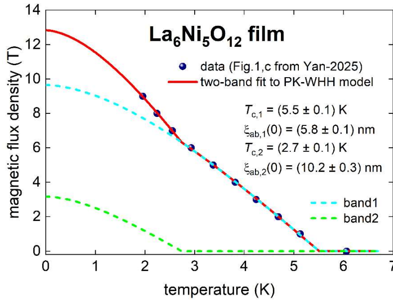
Figure 14. B_{c2}(T) data deduced from R(T,B) curves reported for the ambient pressure single-unit-cell \text{La}_6\text{Ni}_5\text{O}_{12} film reported in Figure 1, c98 and by applying criteria of \frac{R(T=T_{c,0.50})}{R(T=30 \text{ K})} = 0.50 . Data fits to two-band model (Eqs. 3,32). Fit quality is R = 0.9973 . Derived parameters are shown.
