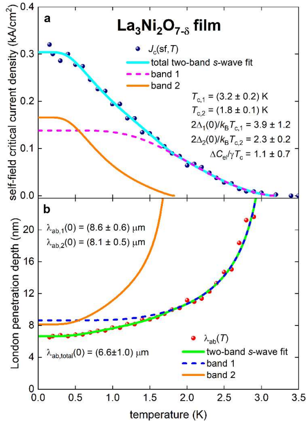
Figure 3. The self-field critical current density, J_c(sf, T) , for the ambient pressure \text{La}_3\text{Ni}_2\text{O}_{7-\delta} film 1 (reported by Ko et al 1 in their Figure 3,a 1 ) and data fit to two-band ( s^- + s^- )-wave model (Eq. 29). The restriction of \left(\frac{\Delta C_{el}}{\gamma T_c}\right)_{\text{band}} = \left(\frac{\Delta C_{el}}{\gamma T_c}\right)_{\text{band2}} has been implemented. Fit quality is R = 0.9674 . Derived parameters are shown.
