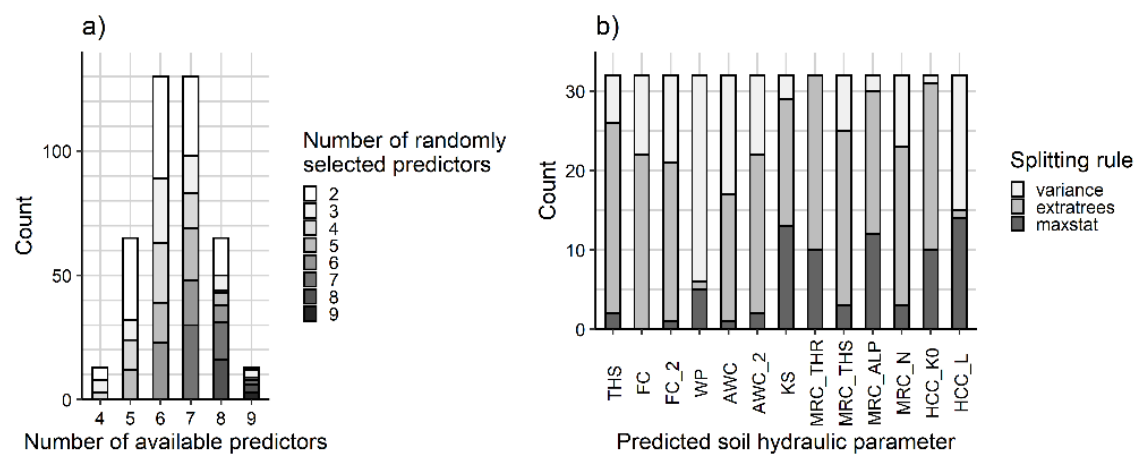
Figure 1. Results of parameter tuning of the random forest: optimization of a) the number of randomly selected predictors at each split by number of available predictors and b) splitting rule applied to build the trees in the random forest.
