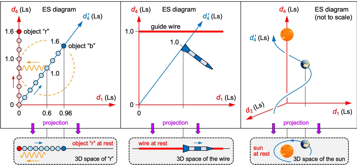
Fig. 4 Three problems. Left: Two objects move through ES. The circle shows where a signal emitted by “b” at d_4 = 1.0 Ls is when another 0.6 s have elapsed in \theta . In ES, the signal and “r” do not collide. In the 3D space of “r”, they do. Center: In ES, the wire escapes from the rocket. In the 3D space of the wire, it does not. Right: In ES, the sun escapes from Earth. In the 3D space of the sun, it does not
