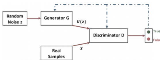
Fig. 9: Schematic structure of a generative adversarial network (GAN).
