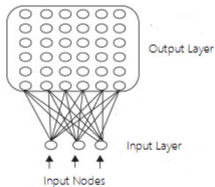
Fig. 5: The self-organizing map (SOM) architecture.
