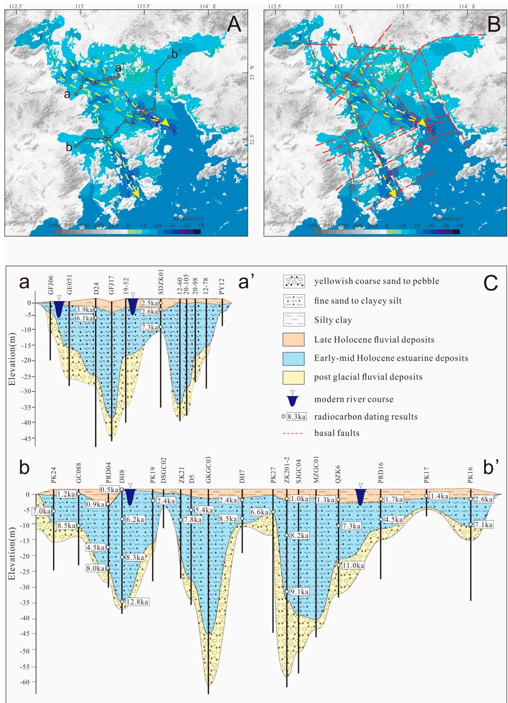
Figure 4. Major paths of the incised valleys (A) and faults (B) in the PRD and cross-sections across the deltaic plains (C).
