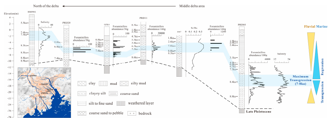
Figure 3. Representative records indicating the interval of maximum marine transgression. The key indicators of a sedimentary environment (e.g. foraminifer, diatom and Sr/Ba ratio) are shown [6,40,43–45].
