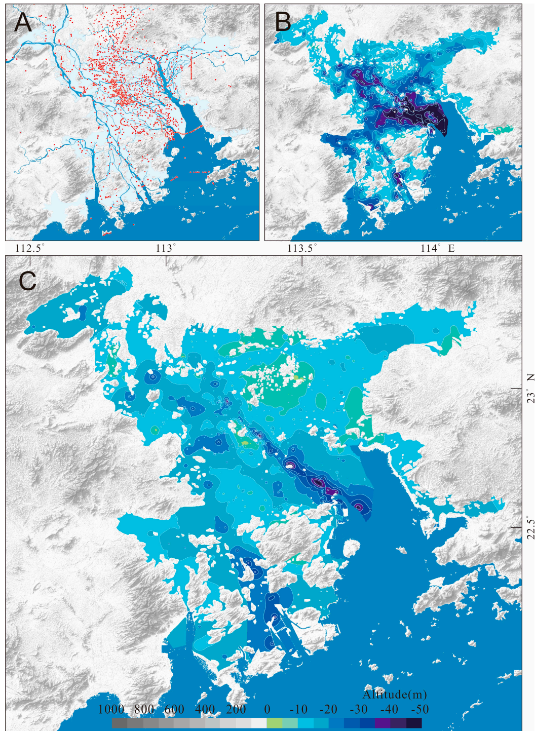
Figure 2. Quaternary isobath maps based on the dataset of 2800 cores. A) Site locations of cores in the database (red dots are core locations); B) Integral isobath map of the Quaternary deposits; C) isobath map of the Holocene deposits.
