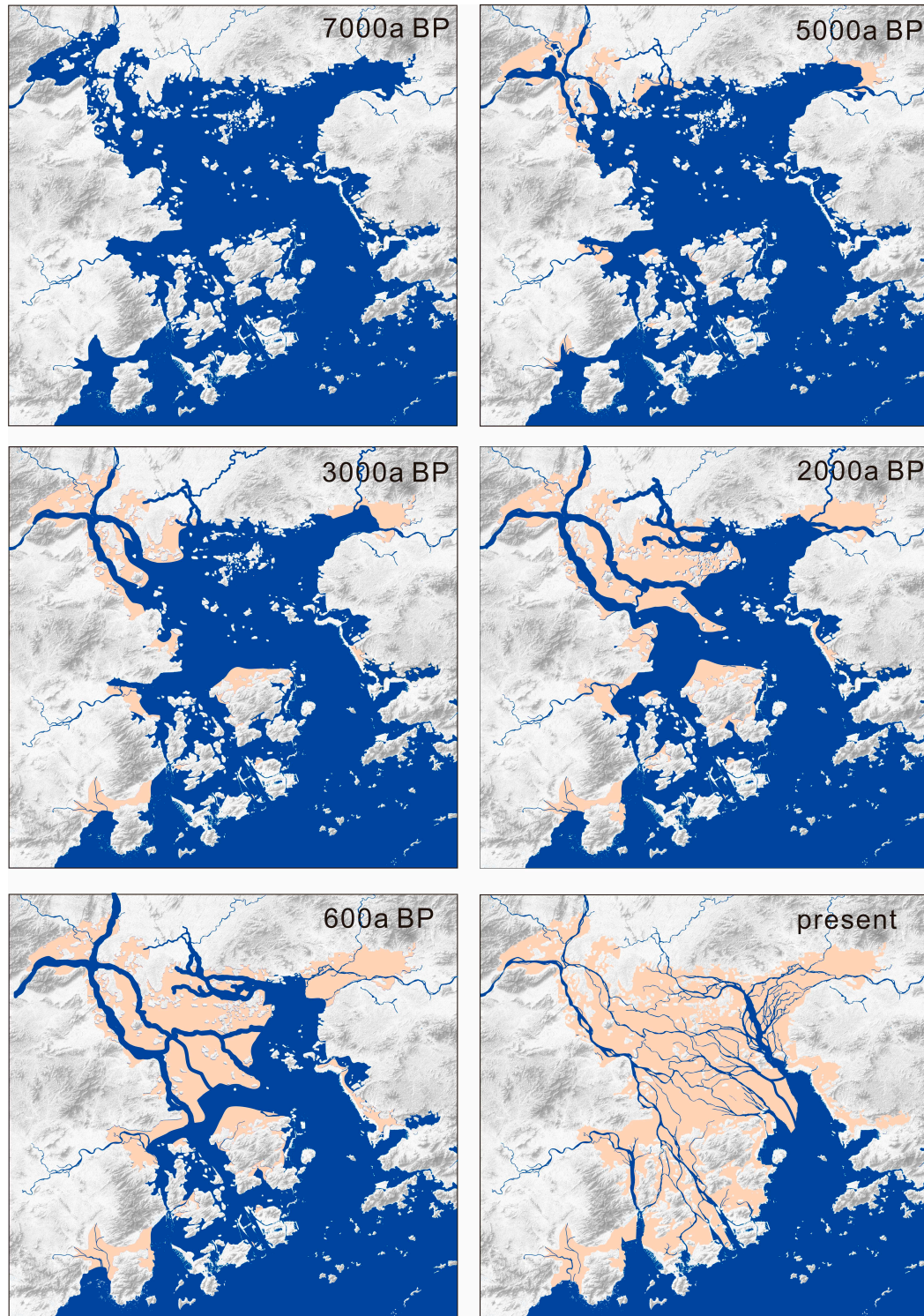
Figure 6. Maps of the paleo-coastline changes reconstructed according to the sediment isobaths taking into consideration evidence including intertidal facies, archaeological and historical records [6], and simulation by millennial-scale morphodynamic models [54].
