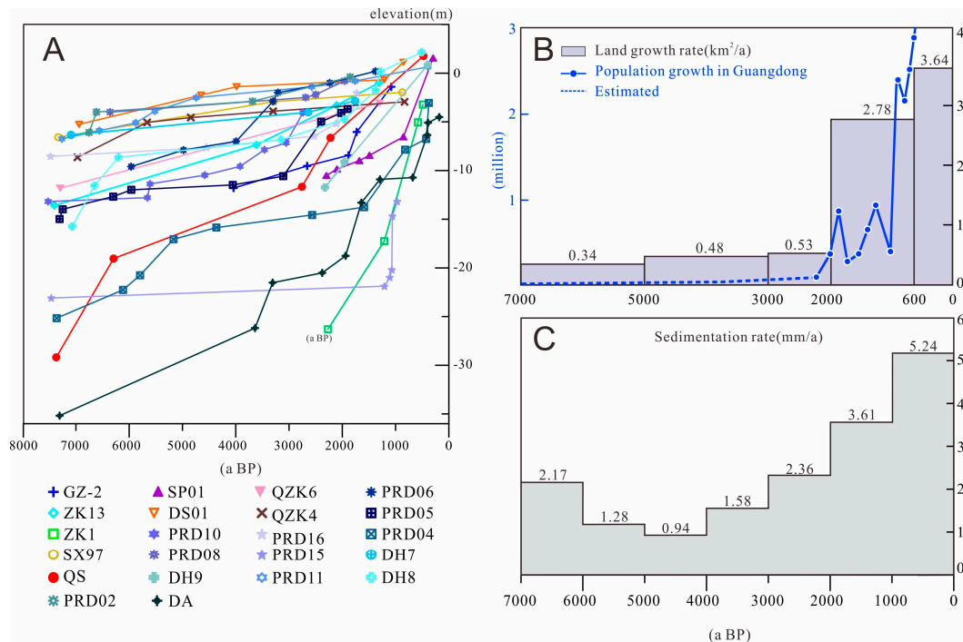
Figure 7. Sedimentation rate and land growth rate compared with regional population growth. A) age-altitude changes in Holocene sediments in the PRD; B) Land growth rate and population in Guangdong [59]; C) Average sedimentation rate in the PRD.
