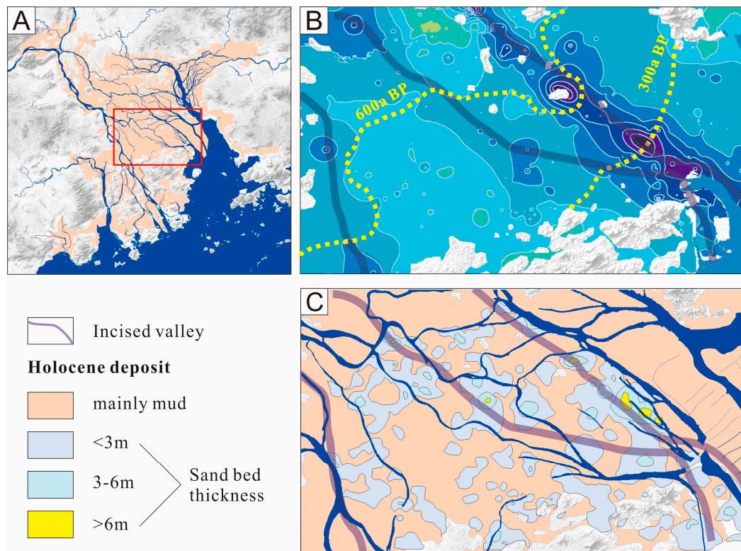
Figure 8. Comparison of incised valleys and present major river courses, and scattered sandy body distribution in an area of the central PRD. A) location of the example area; B) Holocene deposit basement indicating the location of deep incised valleys; C) Overlapping of the deep incised valley with modern river channels, and the distribution of Holocene sandy beds (modified from Yang et al. [60]).
