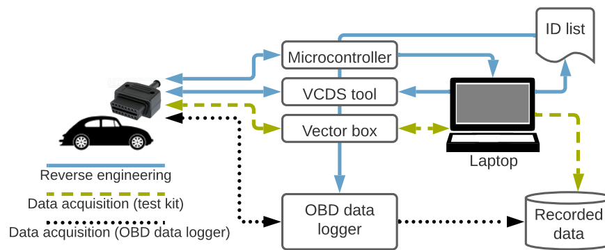
Figure 1. Setup for data acquisition (green: test kit, black OBD logger) and reverse engineering wiring (blue).
