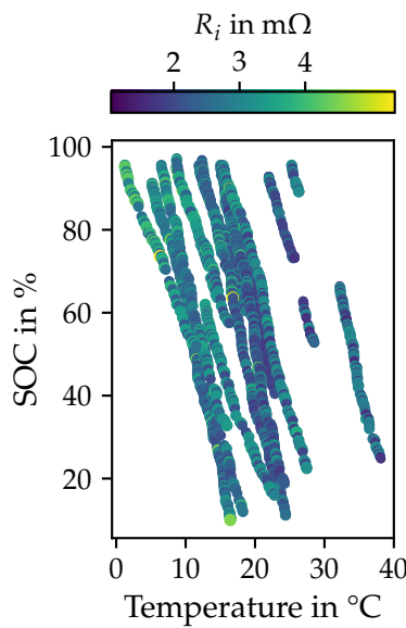
Figure 8. The inferred resistances of all cells as indicated by the color, plotted over the environmental variables SOC and temperature.
