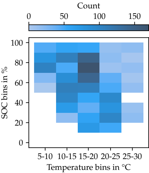
Figure 11. Distribution of all data points in the temperature-SOC plane.
