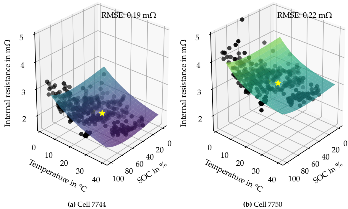
Figure 13. Curve fit of all samples of cell 7744 and 7750 over temperature and SOC. The SOC-axis is modeled by a polynomial and the temperature axis is modeled by an exponential relationship as Equation (4) shows. The reference point R_i is marked in yellow.
