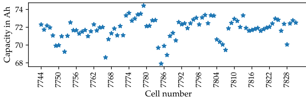
Figure 7. All cells and their capacities derived from one charging record.
