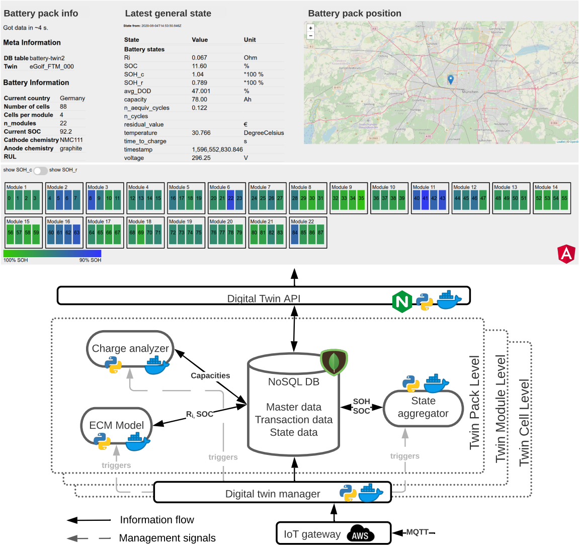
Figure 14. Architecture of the digital twin system. For this work, the system was hosted in the AWS cloud. Individual twins share the same resources as models, aggregators and APIs.
