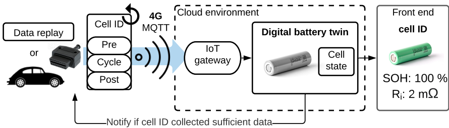
Figure 3. Toolchain to acquire and process the OBD data in a cloud-based digital twin and display on a web front end.
