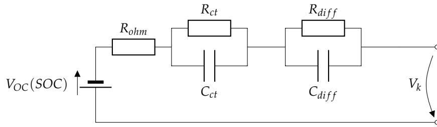
Figure 4. Used ECM containing two RC elements and a SOC-dependant OCV. All parameters in the schema are estimated using least-squares method. V_k and the current serve as reference for the fit.
