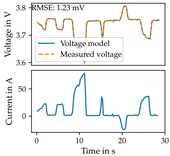
Figure 9. Example fitting result of one 30 s cycle measurement. A RMSE of 1.23 mV indicates a good model fit with the original data. Positive currents correspond to a discharge of the battery.
