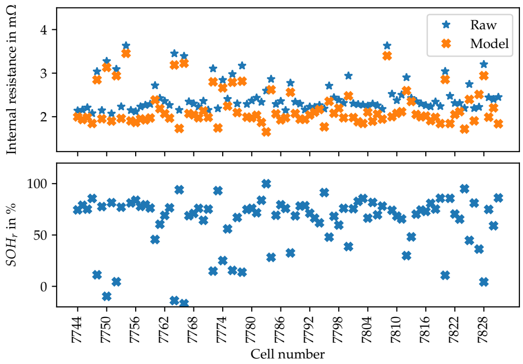
Figure 10. Top: Internal resistance of all cells. The raw values are the average values of all samples passed through the ECM. The model data are the results of the ECM fitted over SOC and temperature, and evaluated at 18 °C and a SOC of 60 %. Bottom: SOH r of the cells. The SOH r cannot be compared to the SOH c . Reference for SOH r : SOH r = 0 at 60 % increase of R_{bol} .
