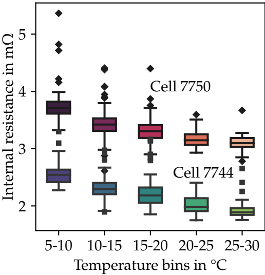
Figure 12. Internal resistance for cell 7744 and 7750 over the temperature. As expected, lower temperatures yield to higher impedance.
