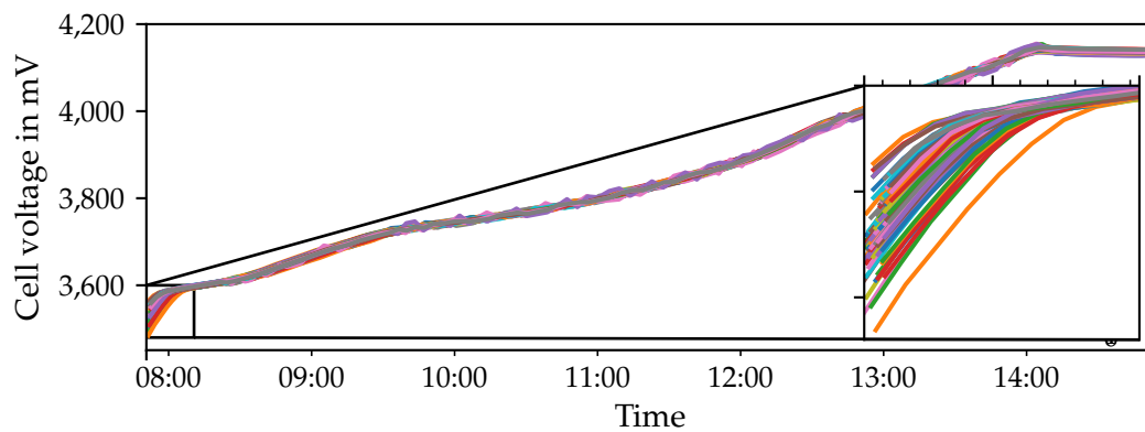
Figure 5. Charging measurement of all cells in the vehicle. Due to cell rotation, we record each cell once every 250 s. We can see that in the lower SOC region deviations are highest.
