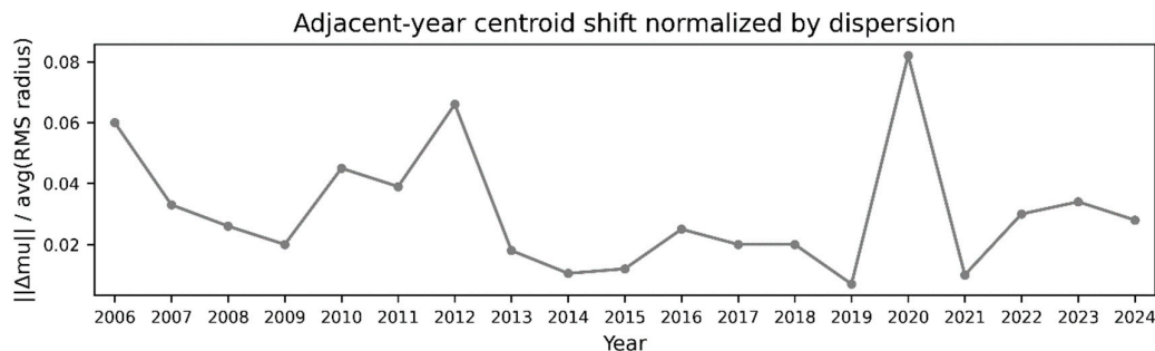
Figure 4. Centroid shift results.
