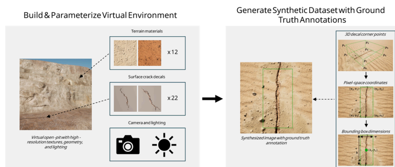
Figure 3. High-level overview of the UE5 synthetic dataset generation pipeline. A parameterized open-pit mine environment is constructed using virtualized geometry exhibiting realistic benches and haul roads, slope faces, and weathered rock surfaces. Domain randomization is applied across variables such as illumination, camera parameters, surface appearance, and crack decal morphology. For each randomized scene instance, high resolution images are captured and annotated by projecting the 3D decal corner points into image space to compute ground-truth bounding box dimensions. Image and label pairs are then exported for downstream generative modelling using StyleGAN2-ADA.
