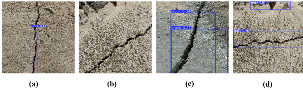
Figure 13. UE5O surface crack detection performance on real-world open-pit test images, showing low-confidence and missed detections across subplots (a-d). Fragmented and inconsistent spatial coverage is observed in subplots (a) and (c), while subplot (d) highlights a false positive triggered by background debris and shadowing effects.
