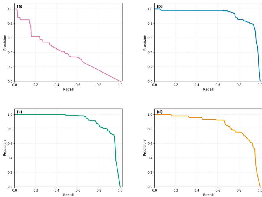
Figure 14. Precision-recall characteristics for the four YOLOv11 dataset configurations evaluated on the real-world open-pit surface crack test set. The curves demonstrate the trade-off between precision and recall across confidence thresholds, for (a) UE5O, (b) UE5O + SG2, (c) UE5O + SG2-FFHQ, and (d) UE5O + SG2-DTD, highlighting the improved robustness and extended high-precision regions of the SG2-adapted variants relative to the UE5O baseline.
