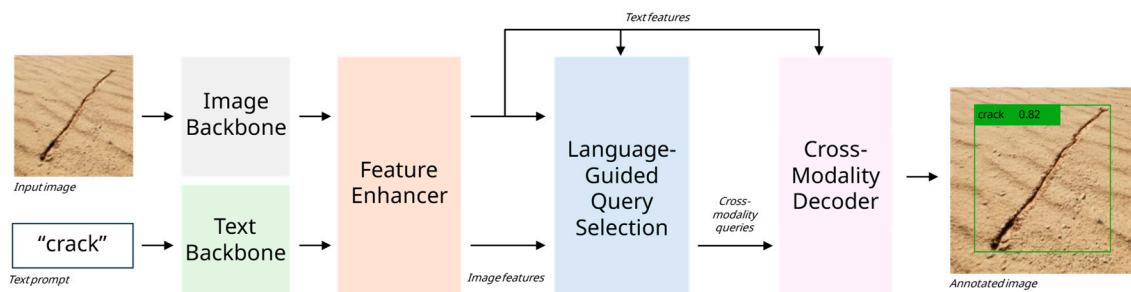
Figure 5. High-level overview of the Grounding DINO pipeline used for pseudo-labelling the images generated by StyleGAN2-ADA. The input image and text prompt are encoded by their respective backbones and fused in the feature enhancer, which injects semantic text information into the visual features via cross-attention. The resulting language-conditioned object queries, together with multi-scale image features, are processed by the cross-modality decoder. The decoder outputs are then linearly projected into bounding-box coordinates and text-region alignment scores, yielding detections corresponding to the text prompt used, in this case, “crack”.
