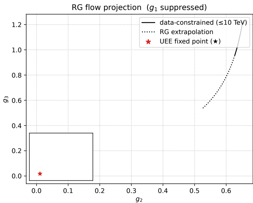
Figure A10. Projection onto the g_2 – g_3 plane. Symbols are the same as in Figure A9.
