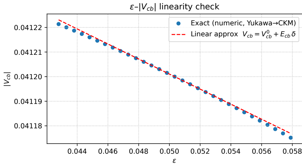
Figure A12. \epsilon variation and |V_{cb}| . Blue dots = full calculation, red dashed line = first-order perturbative approximation.
