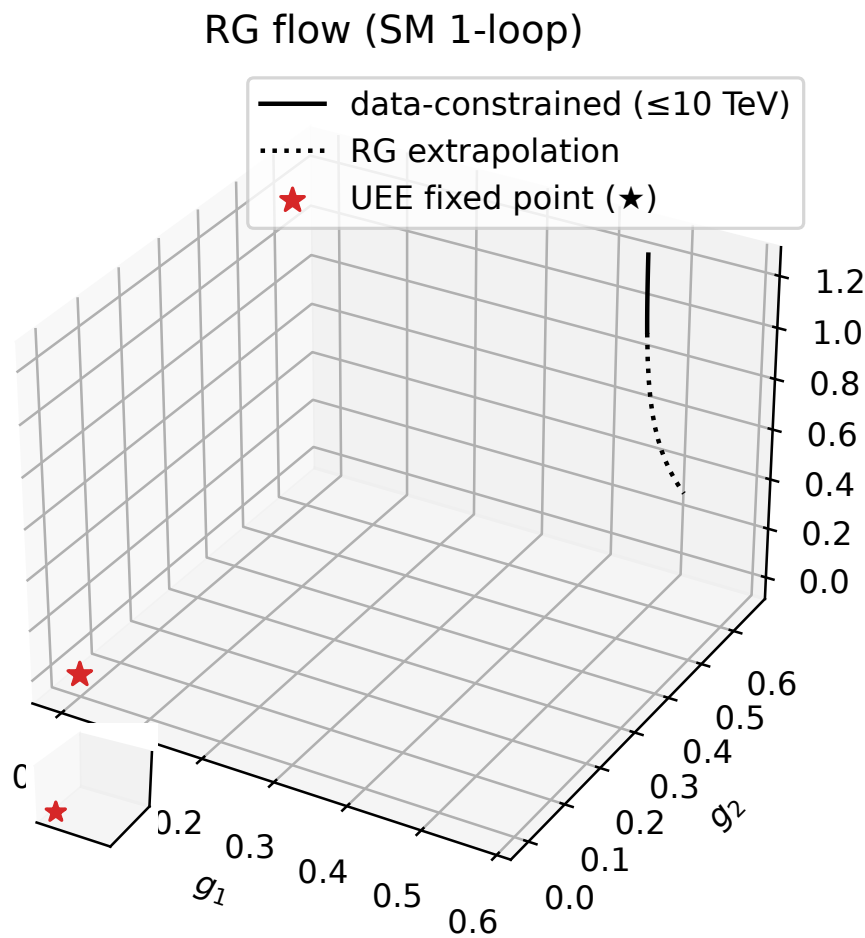
Figure A9. RG flow (3D). Thick solid line = measured region, dotted = extrapolation. ★ = UEE fixed point.
