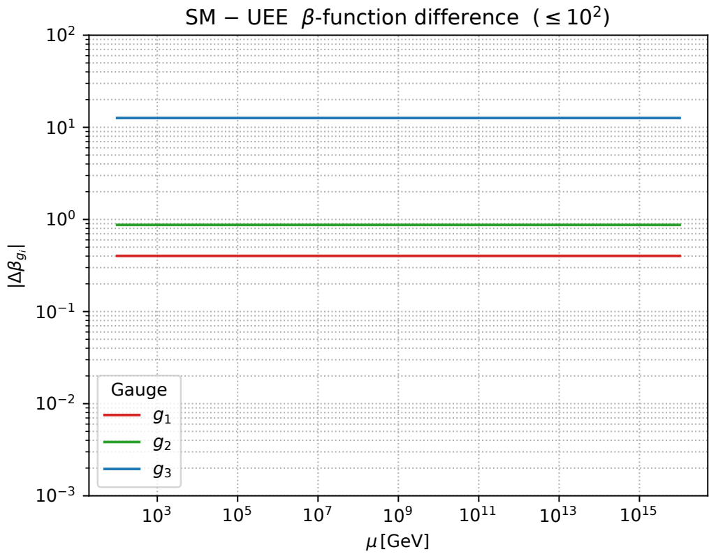
Figure A1. Difference of \beta functions between SM and UEE, |\Delta\beta_{g_i}| (combined 1–3 loop).
