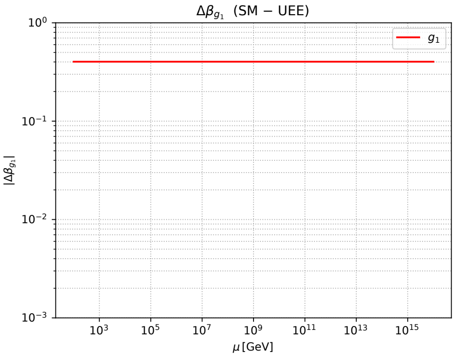
Figure A2. Plot of \Delta\beta_{g_1} only.
