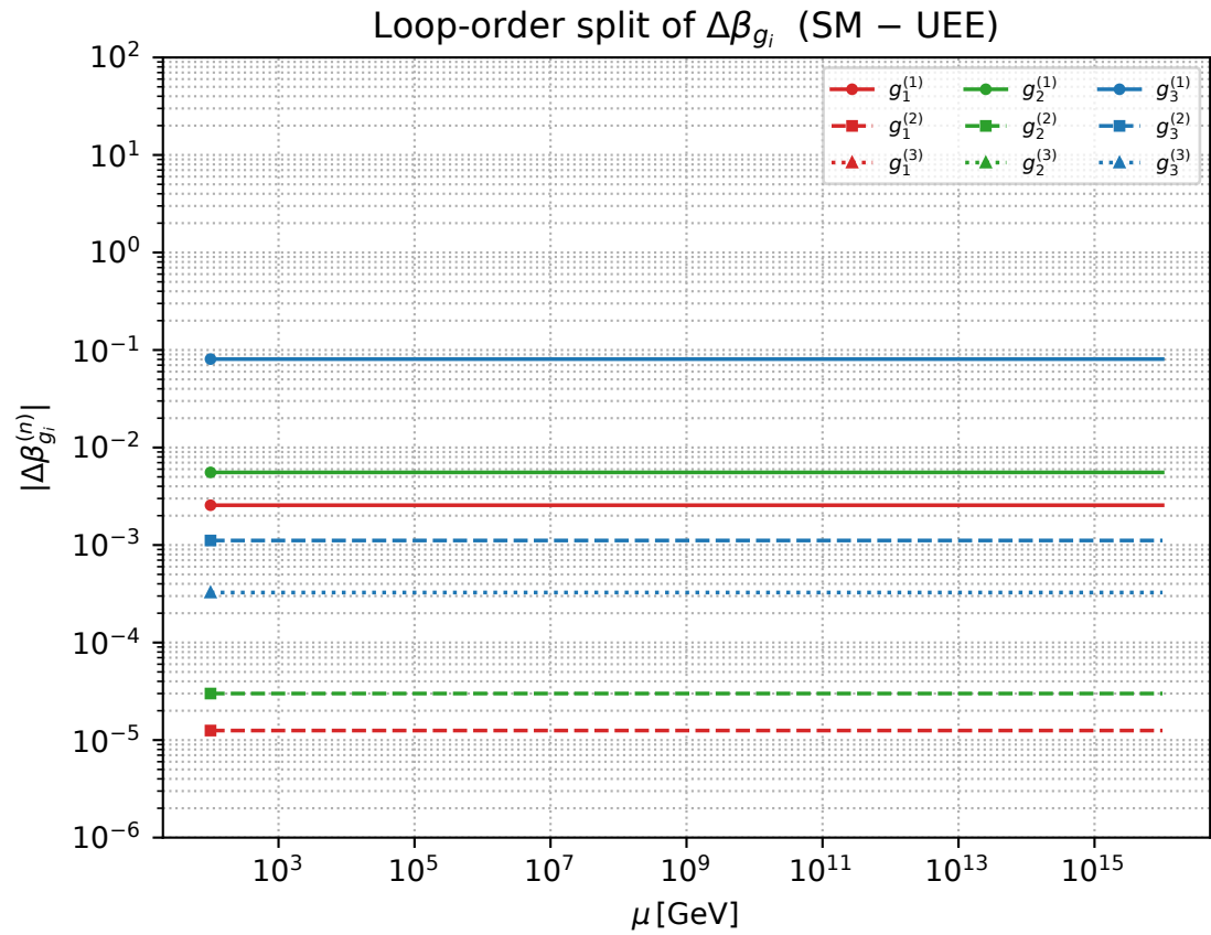
Figure A5. \Delta\beta_{g_i}^{(n)} by loop order. Solid line = 1-loop, dashed = 2-loop, dotted = 3-loop.
