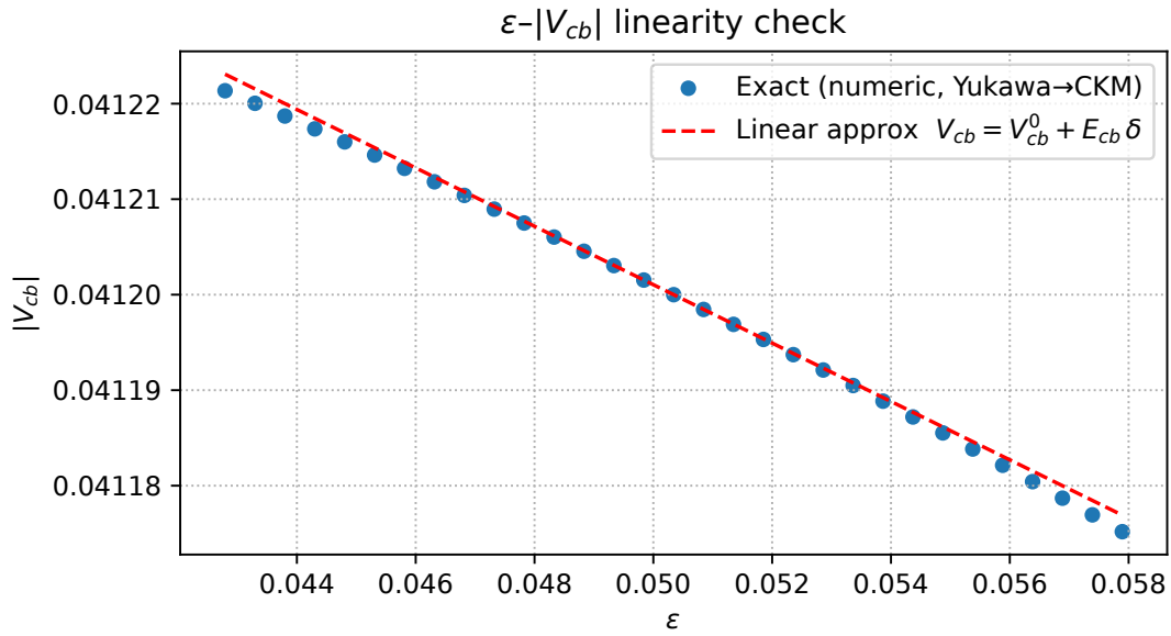
Figure A15. Linearity test of \epsilon variation versus |V_{cb}| . Blue dots = full recalculation of the Yukawa matrices, red dashed line = linear approximation E_{cb} \delta . The difference is below 10^{-6} , confirming the high precision of the linear perturbative formula.
