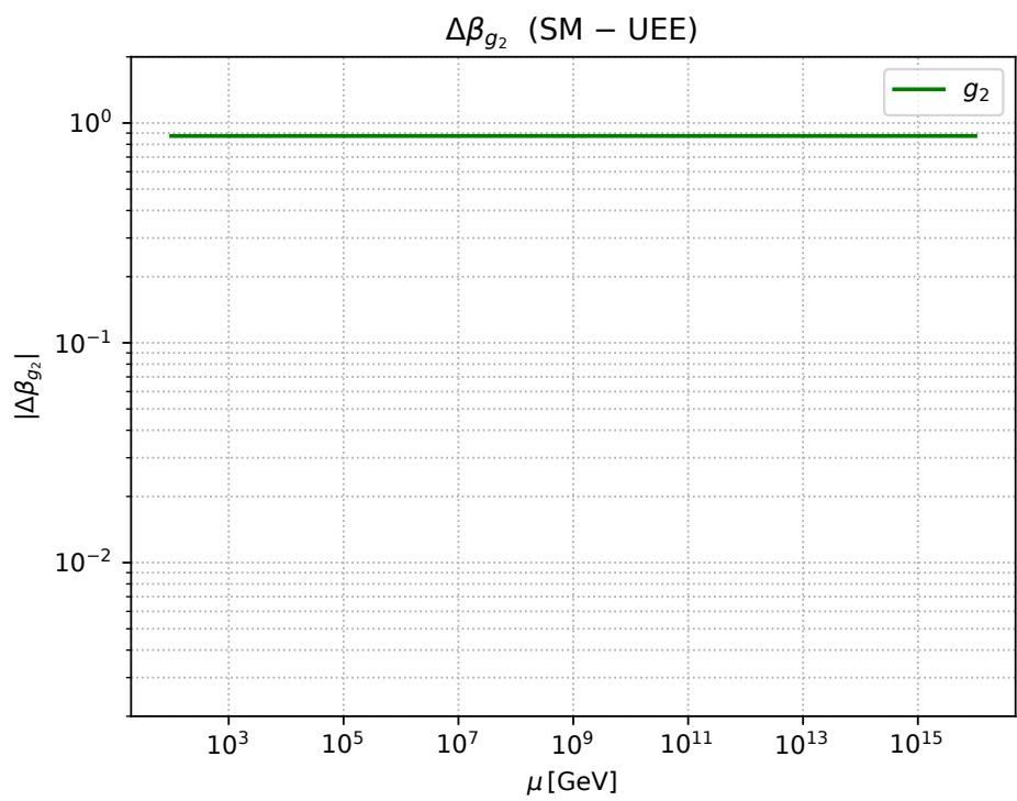
Figure A3. Plot of \Delta\beta_{g_2} only.
