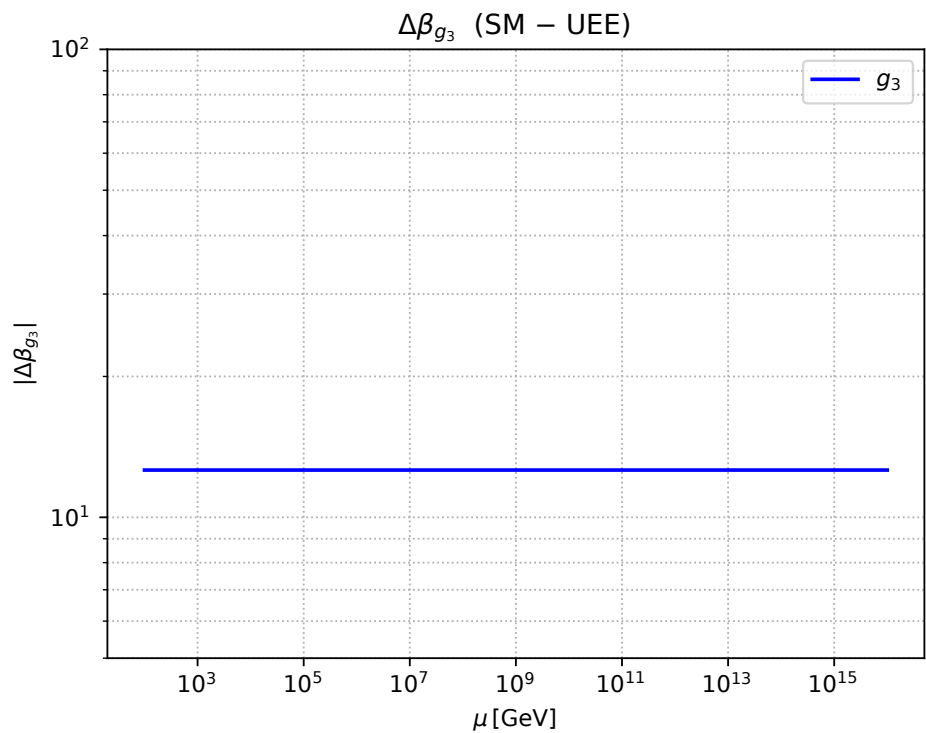
Figure A4. Plot of \Delta\beta_{g_3} only.
