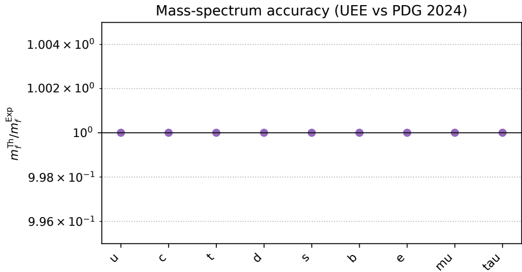
Figure A6. Mass ratios m_f^{Th}/m_f^{Exp} (logarithmic).
