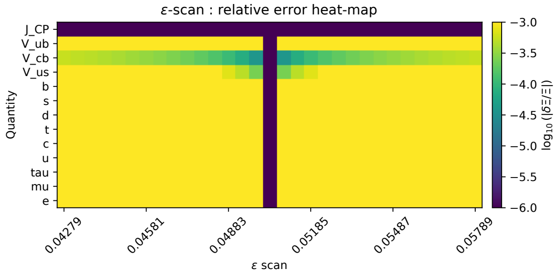
Figure A11. Heatmap of relative error \log_{10}(|\delta\Xi/\Xi|) with respect to \epsilon variation.
