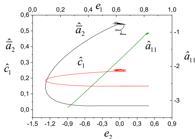
Figure 7. Phase portraits of AIS in spaces (e_1, \hat{a}_{11}) , (e_2, \hat{c}_1) and (e_2, \hat{a}_2) .
