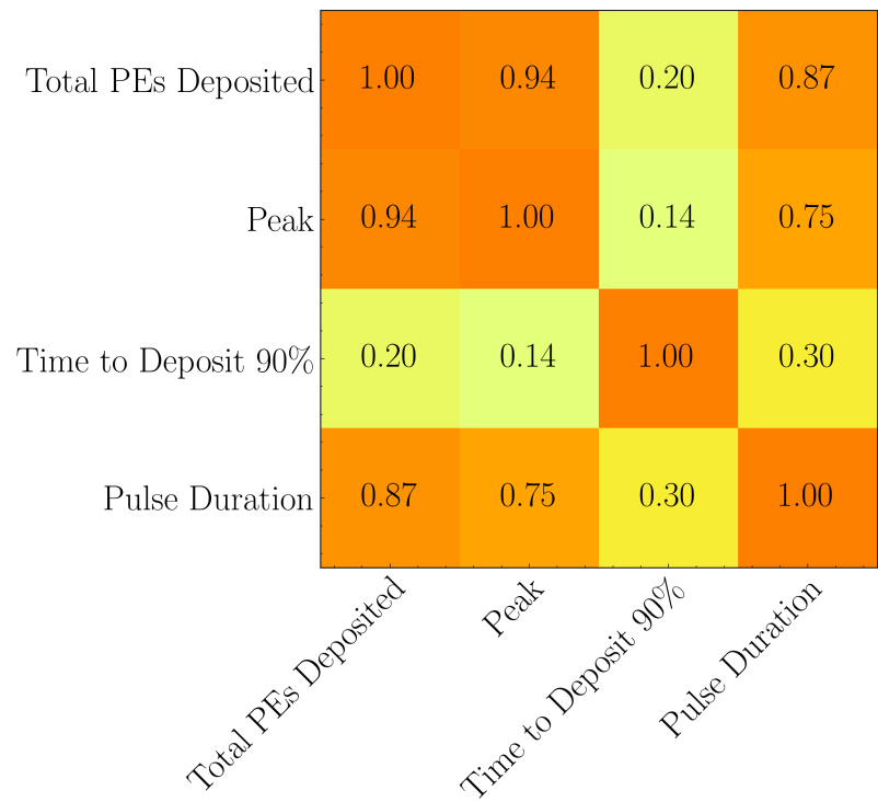
Figure 4. Cross-correlation matrix of initial feature set.
