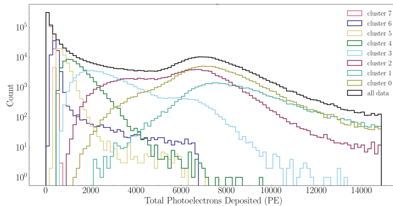
Figure 6. Histogram of charge, in black, with resulting clusters labeled and colored. The Y-axis is in a logarithmic scale for clarity.
