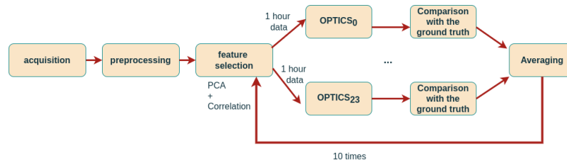
Figure 3. General data pipeline for the ML modelling.
