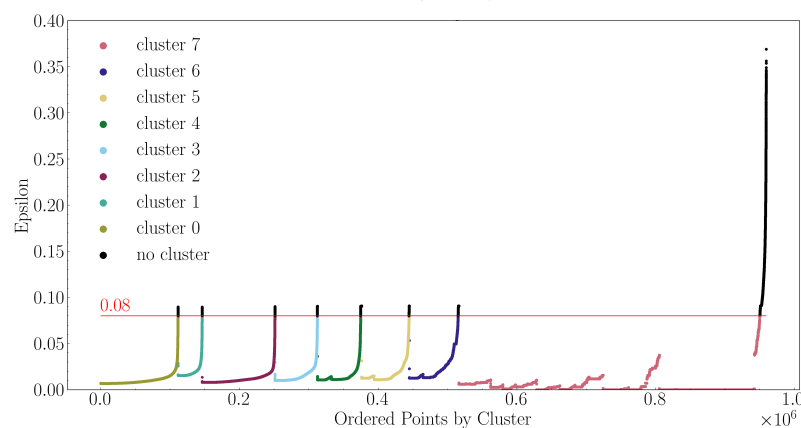
Figure 5. Example of a reachability plot from one run of the ML pipeline. A consistent cut-off threshold of 0.08 was used in every run where each independent run produced a similar plot. Points belonging to a cluster are colored and labeled accordingly, while any point in black did not gain membership to any cluster. A total of eight clusters were found.
